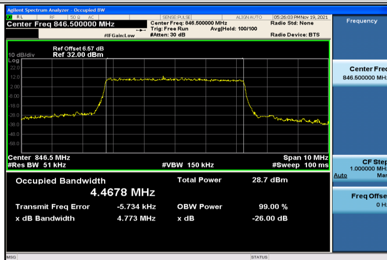
Band5-5MHz-16QAM-20625-25RB#0-4.4678
