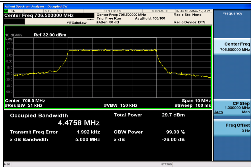
Band17-5MHz-QPSK-23755-25RB#0-4.4758
