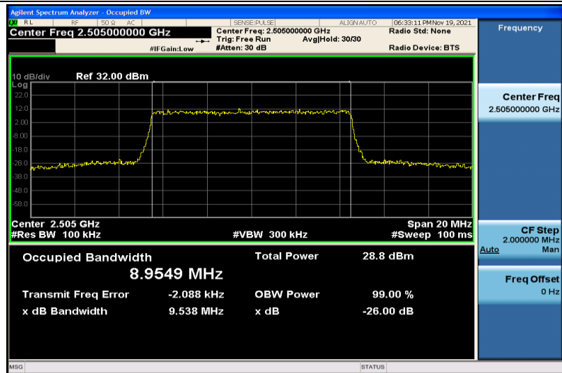
Band7-10MHz-16QAM-20800-50RB#0-8.9549
