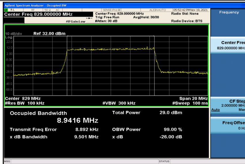
Band5-10MHz-16QAM-20450-50RB#0-8.9416
