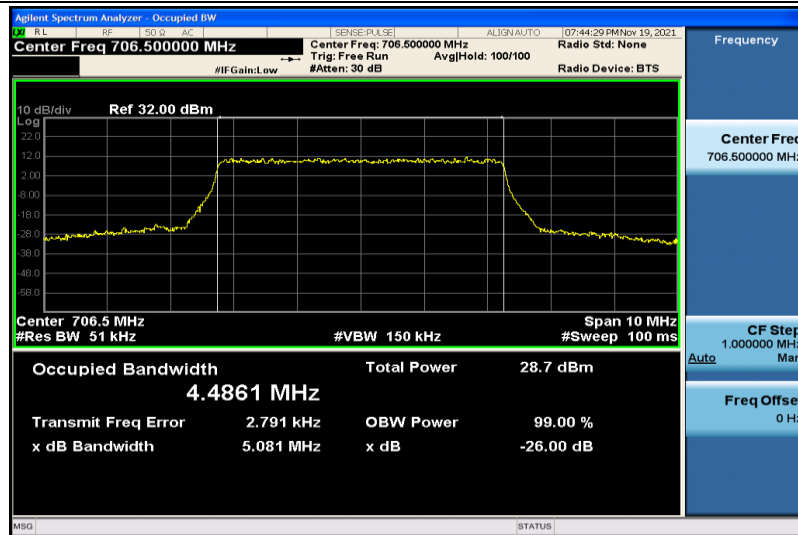
Band17-5MHz-16QAM-23755-25RB#0-4.4861
