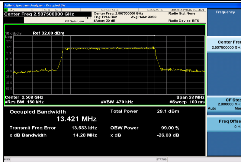
Band7-15MHz-16QAM-20825-75RB#0-13.421
