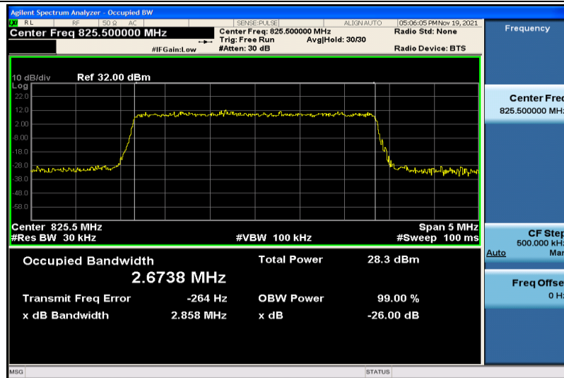
Band5-3MHz-16QAM-20415-15RB#0-2.6738
