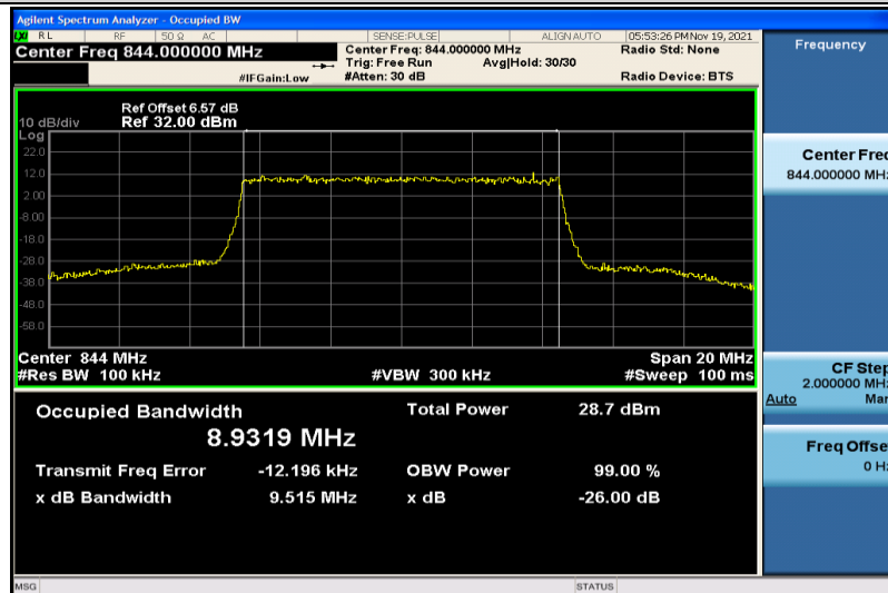
Band5-10MHz-16QAM-20600-50RB#0-8.9319
