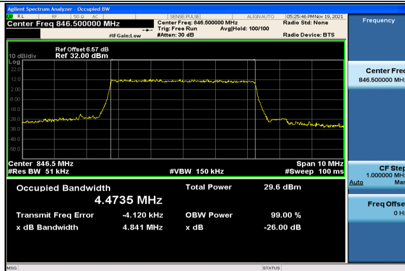
Band5-5MHz-QPSK-20625-25RB#0-4.4735
