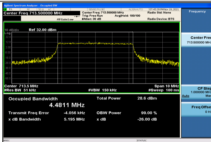
Band17-5MHz-16QAM-23825-25RB#0-4.4811
