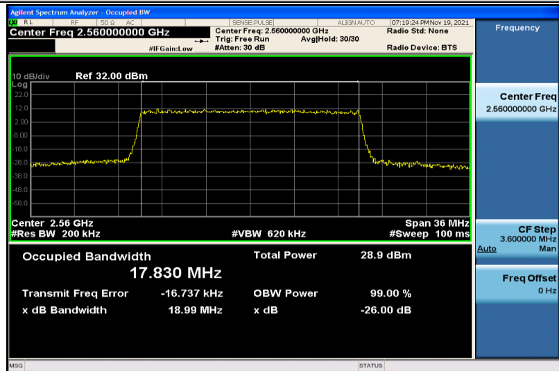
Band7-20MHz-16QAM-21350-100RB#0-17.830
