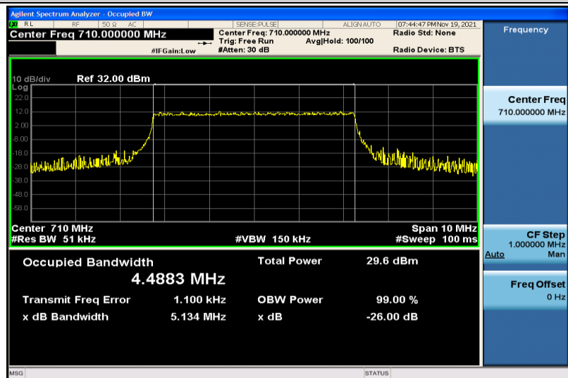
Band17-5MHz-QPSK-23790-25RB#0-4.4883
