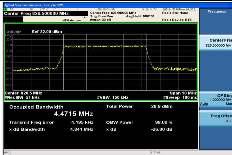
Band5-5MHz-16QAM-20425-25RB#0-4.4715
