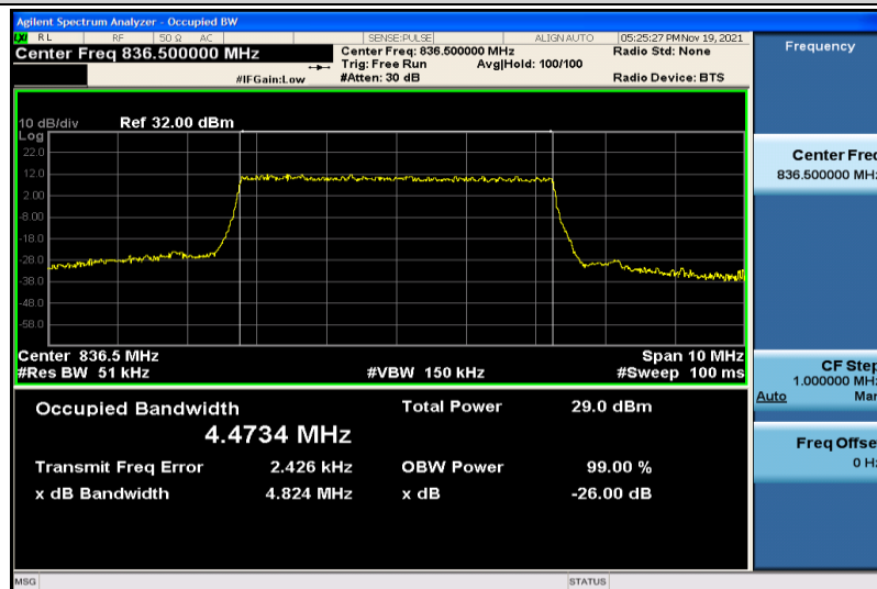
Band5-5MHz-16QAM-20525-25RB#0-4.4734
