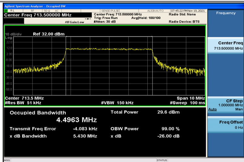
Band17-5MHz-QPSK-23825-25RB#0-4.4963
