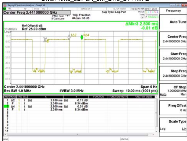
Dwell Time_8DPSK_3M_DH5_2441MHz
