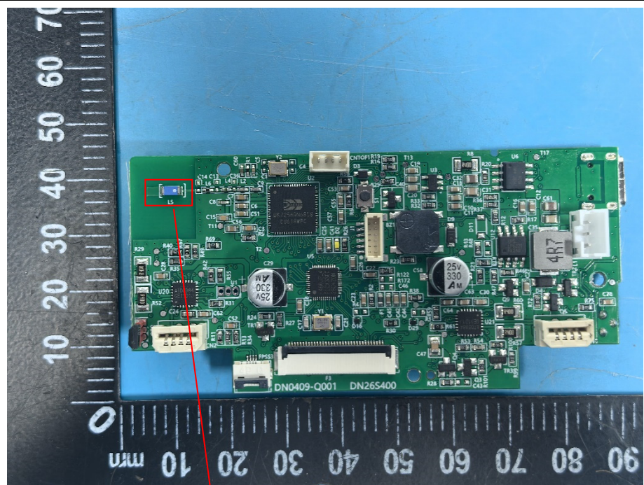
Bluetooth Antenna
