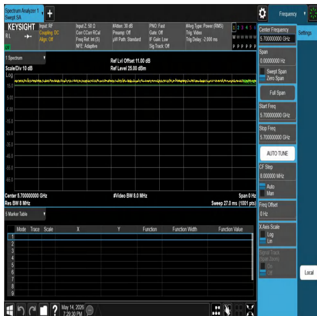
NTNV-11N20SISO-Ant1-5700
