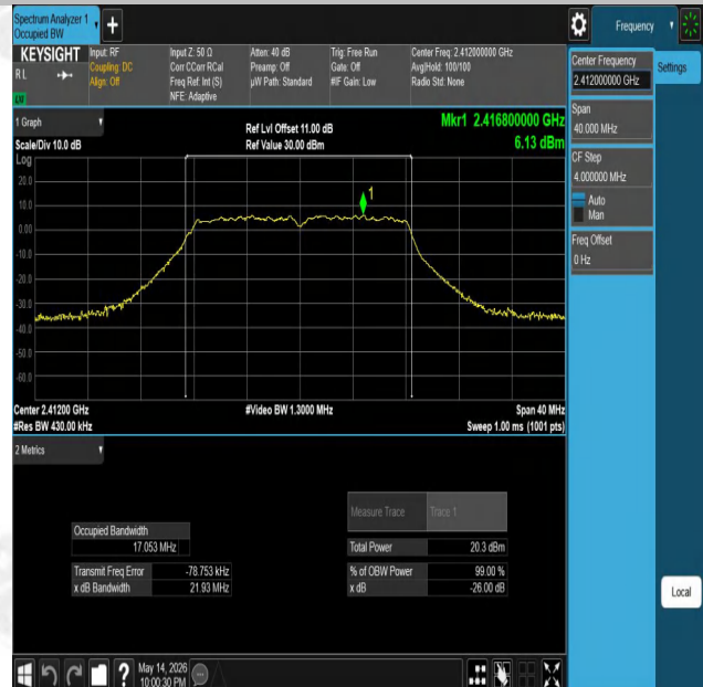
11G-Ant1-2412
