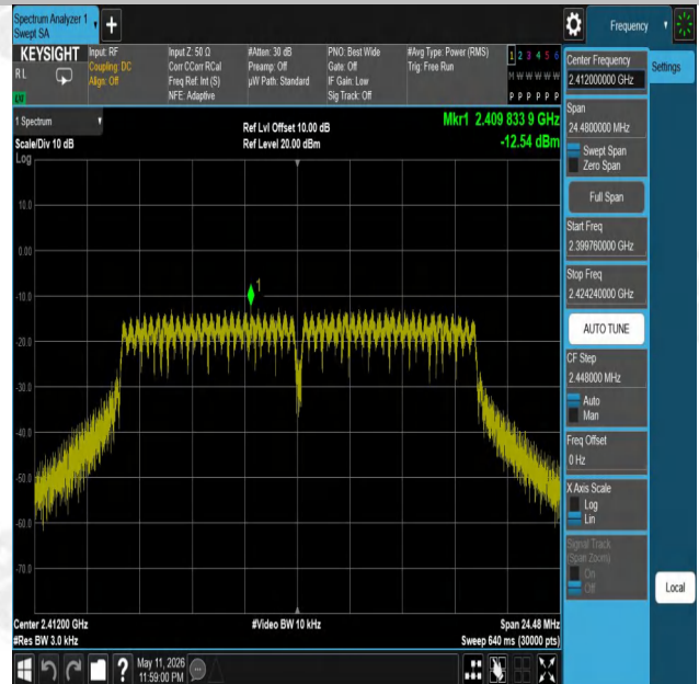
11G-Ant1-2412-PASS
