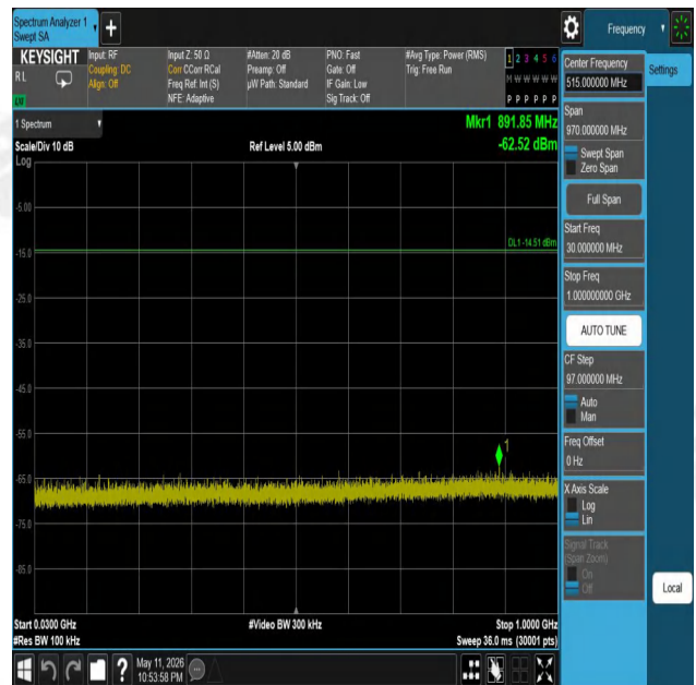
11B-Ant1-2412-30~1000-PASS
