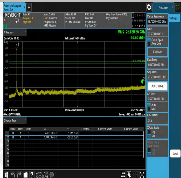
11G-Ant1-2412-1000~26500-PASS
