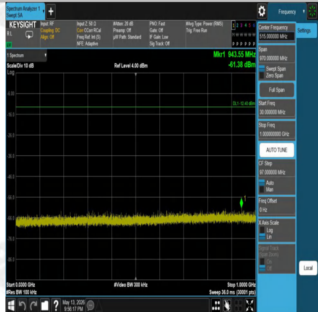
11B-Ant1-2462-30~1000-PASS
