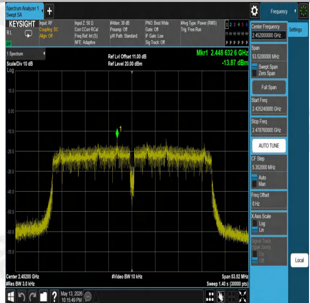
11N40SISO-Ant1-2452-PASS
