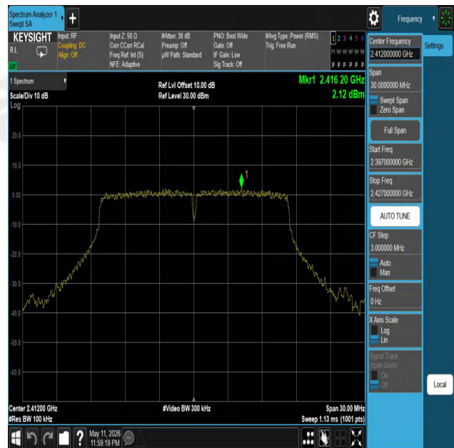
11G-Ant1-2412-0~Reference-PASS
