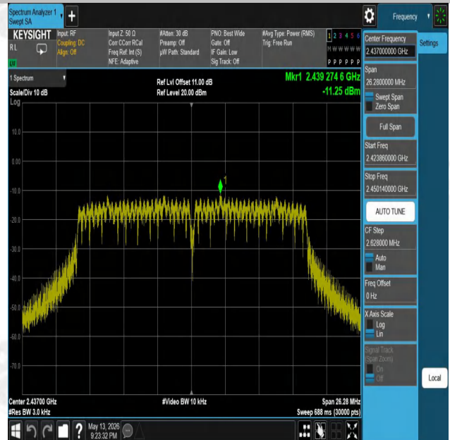
11N20SISO-Ant1-2437-PASS
