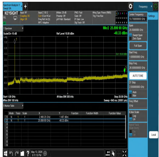
11G-Ant1-2462-1000~26500-PASS
