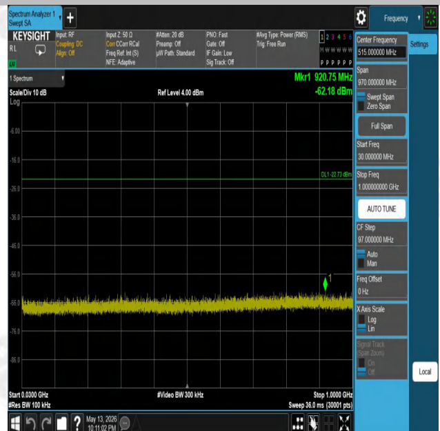
11N40SISO-Ant1-2437-30~1000-PASS
