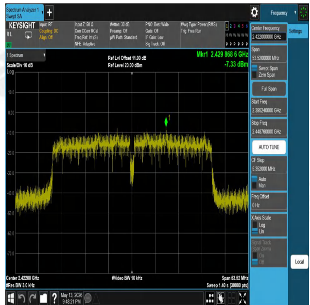
11N40SISO-Ant1-2422-PASS
