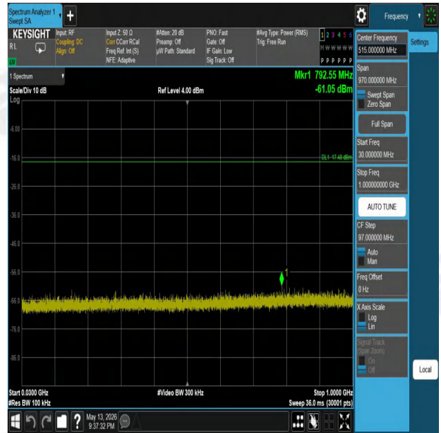
11N20SISO-Ant1-2462-30~1000-PASS
