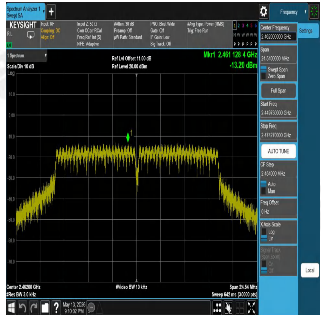
11G-Ant1-2462-PASS
