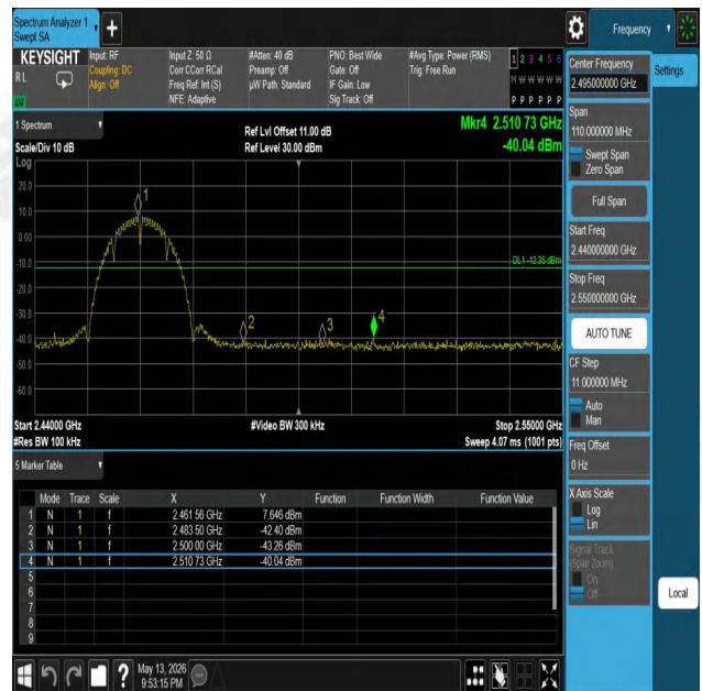
11B-Ant1-2462-PASS
