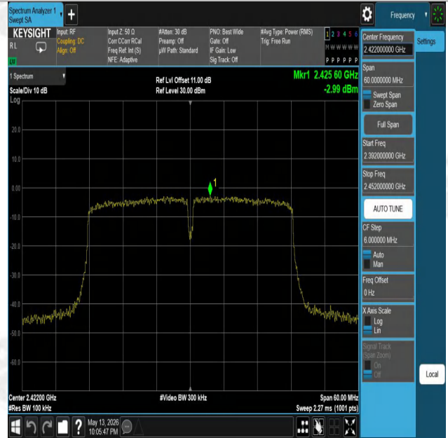
11N40SISO-Ant1-2422-0~Reference-PASS
