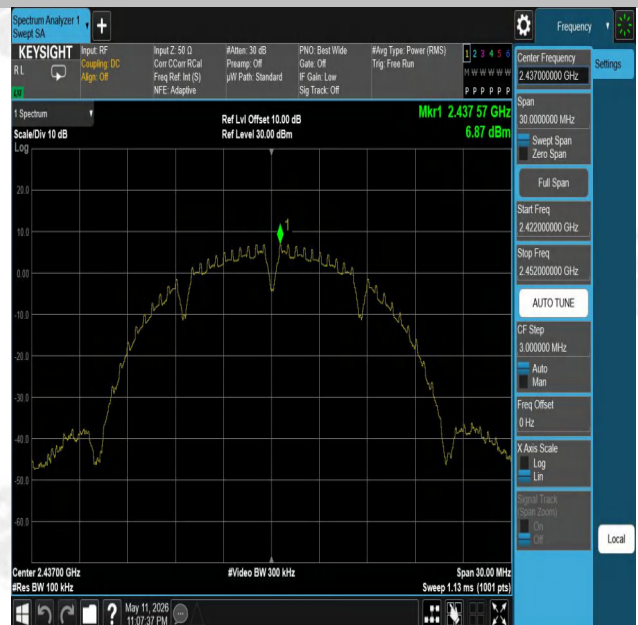
11B-Ant1-2437-0~Reference-PASS
