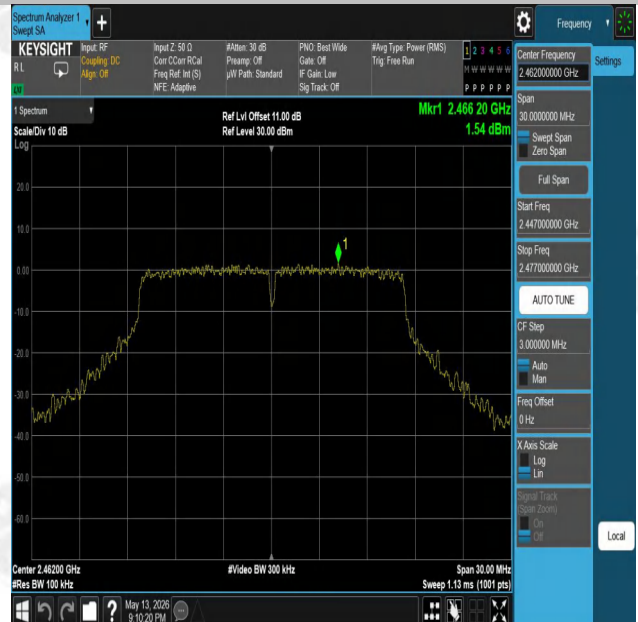
11G-Ant1-2462-0~Reference-PASS
