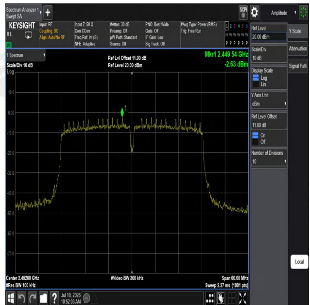
11N40SISO-Ant1-2452-0~Reference-PASS
