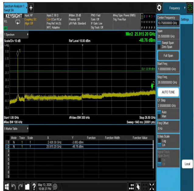
11N40SISO-Ant1-2422-1000~26500-PASS
