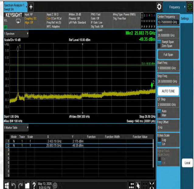
11N20SISO-Ant1-2437-1000~26500-PASS
