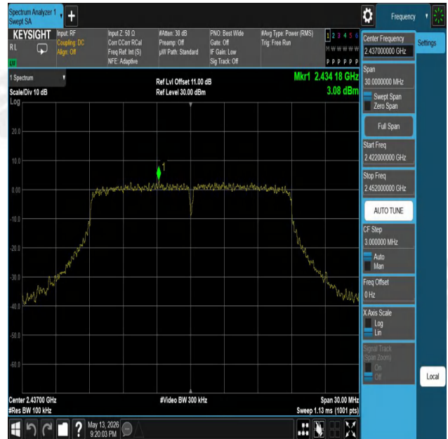
11N20SISO-Ant1-2437-0~Reference-PASS
