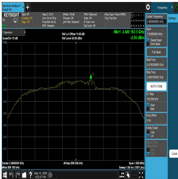
3DH5-Ant1-2480-0~Reference-PASS
