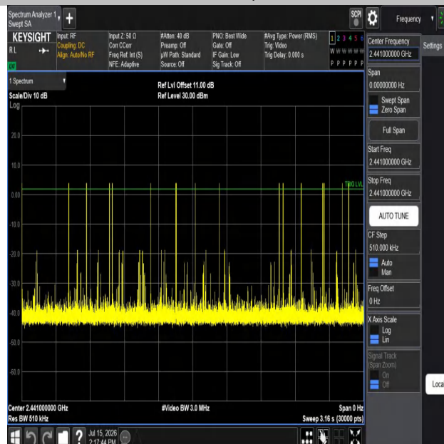
DH3-Ant1-Hop-PASS
