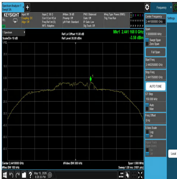
2DH5-Ant1-2441-0~Reference-PASS
