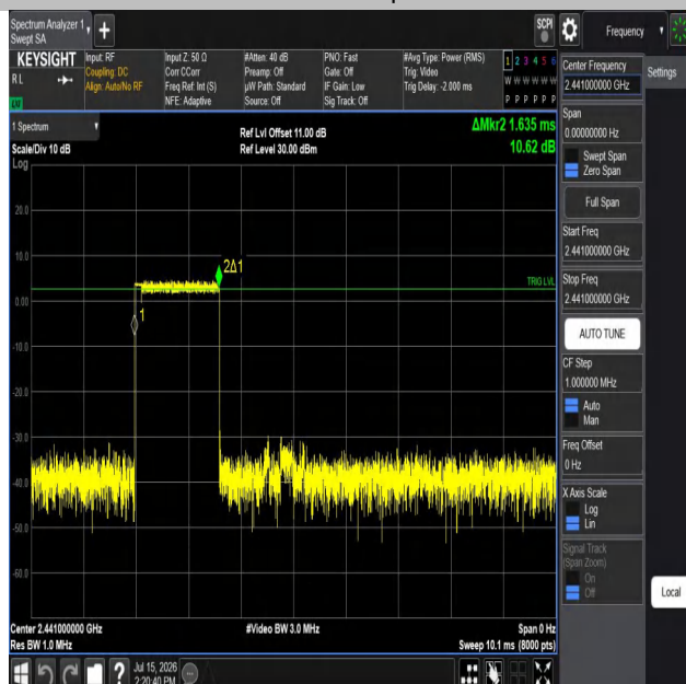
3DH3-Ant1-Hop-PASS
