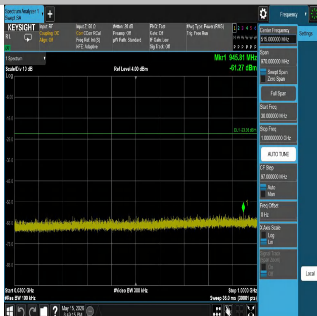
3DH5-Ant1-2441-30~1000-PASS
