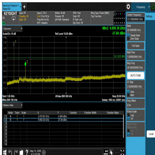
DH5-Ant1-2480-1000~26500-PASS
