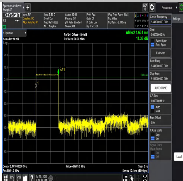
DH3-Ant1-Hop-PASS
