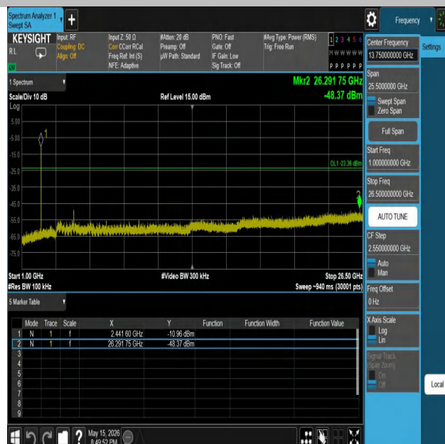
3DH5-Ant1-2441-1000~26500-PASS
