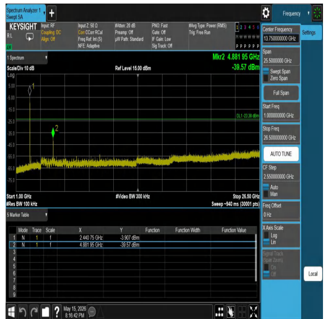
DH5-Ant1-2441-1000~26500-PASS
