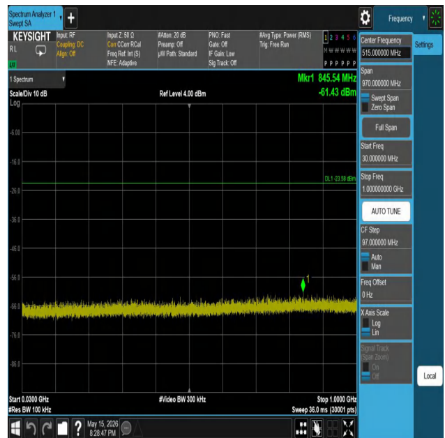
2DH5-Ant1-2441-30~1000-PASS
