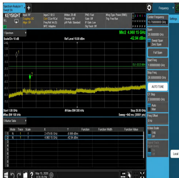
2DH5-Ant1-2480-1000~26500-PASS
