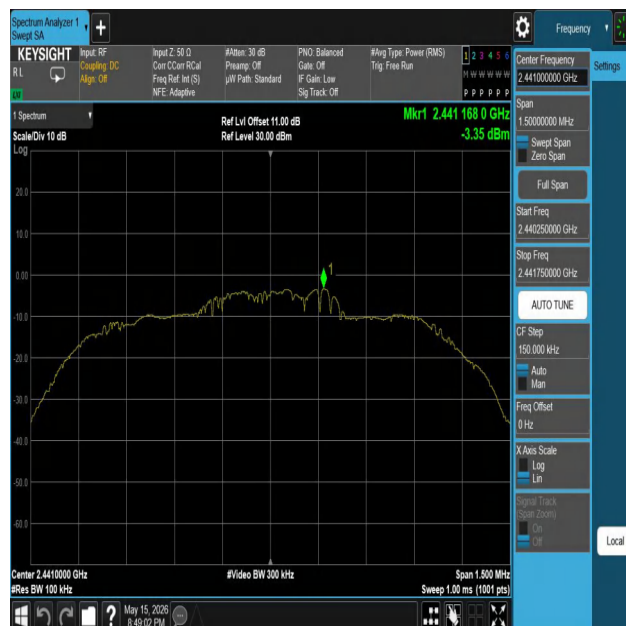
3DH5-Ant1-2441-0~Reference-PASS
