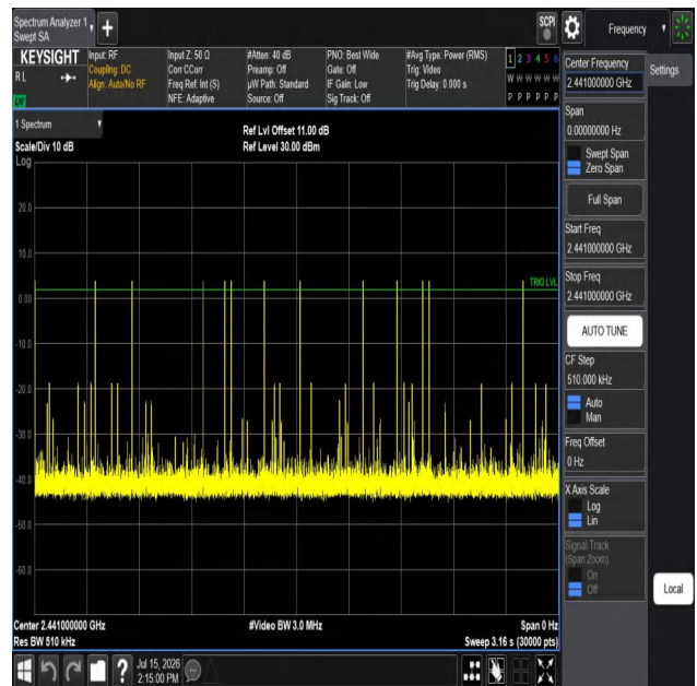
DH5-Ant1-Hop-PASS
