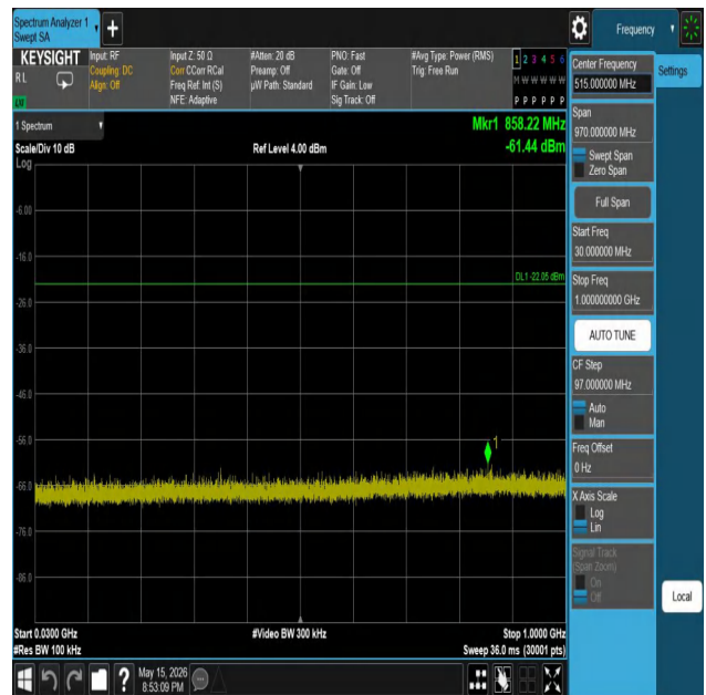
3DH5-Ant1-2480-30~1000-PASS
