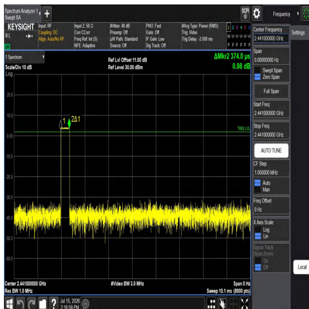
DH1-Ant1-Hop-PASS
