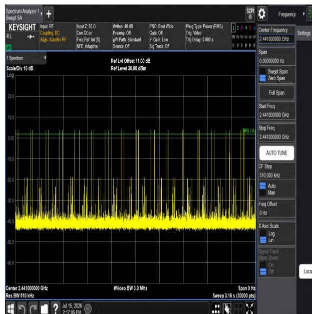
DH1-Ant1-Hop-PASS
