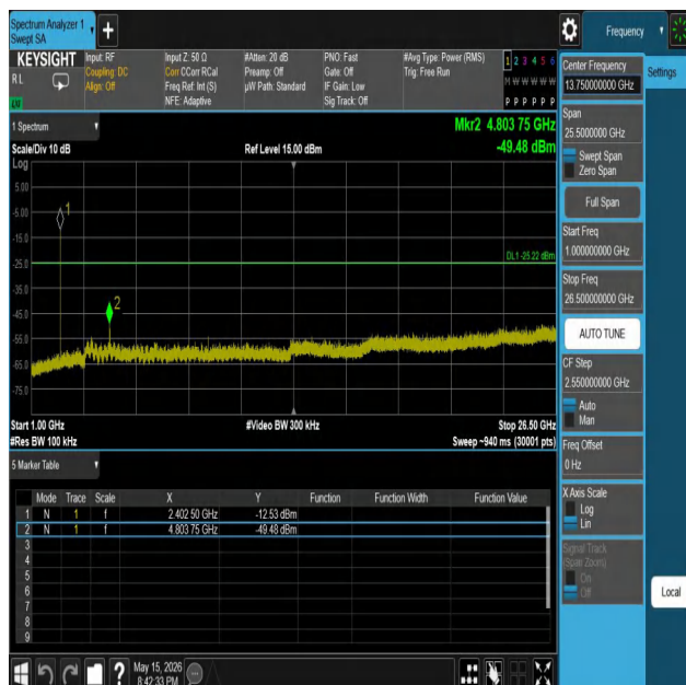
3DH5-Ant1-2402-1000~26500-PASS
