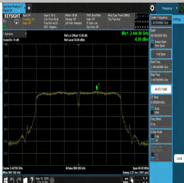
11N40SISO-Ant1-2437-0~Reference-PASS
