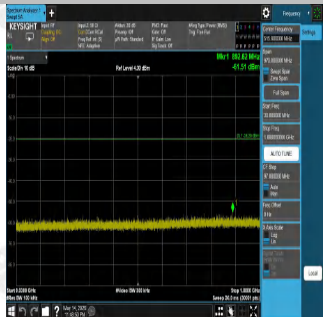
11N20SISO-Ant1-2412-30~1000-PASS
