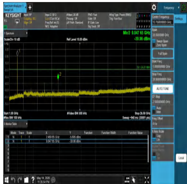
11G-Ant1-2462-1000~26500-PASS
