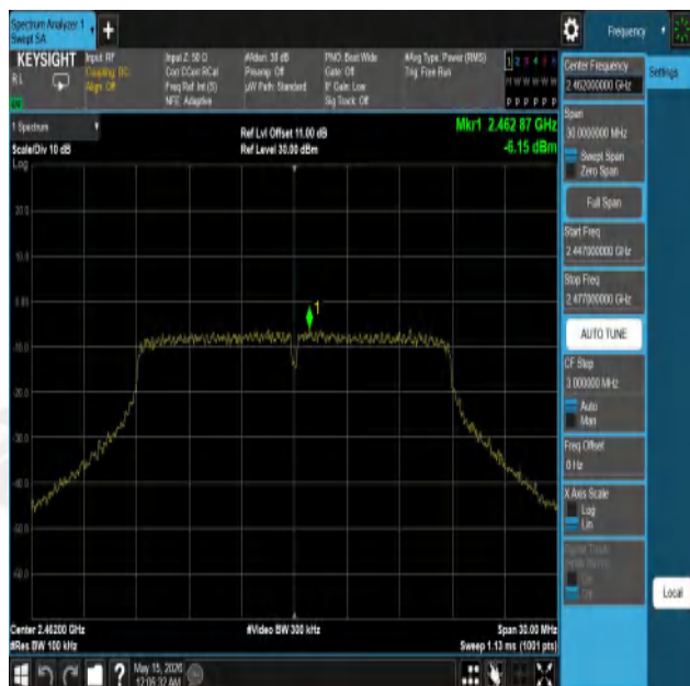
11N20SISO-Ant1-2462-0~Reference-PASS
