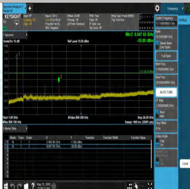
11N20SISO-Ant1-2462-1000~26500-PASS
