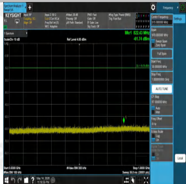
11B-Ant1-2462-30~1000-PASS
