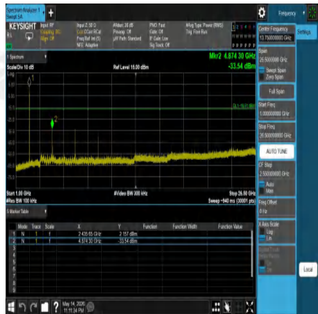
11B-Ant1-2437-1000~26500-PASS
