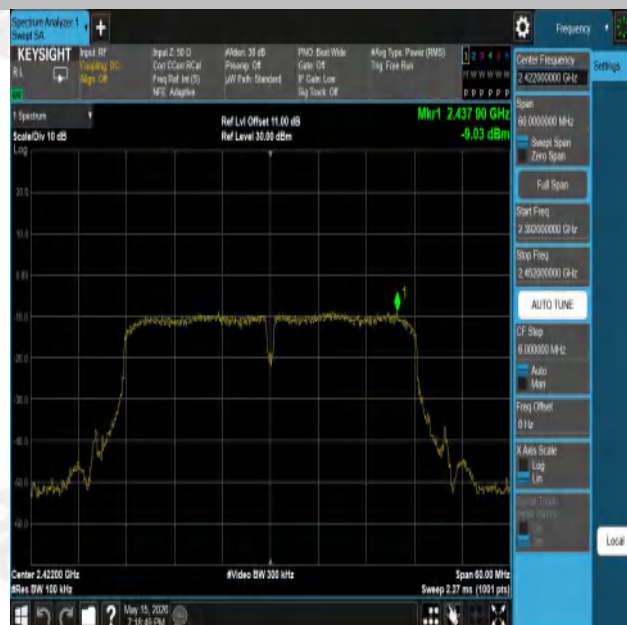
11N40SISO-Ant1-2422-0~Reference-PASS
