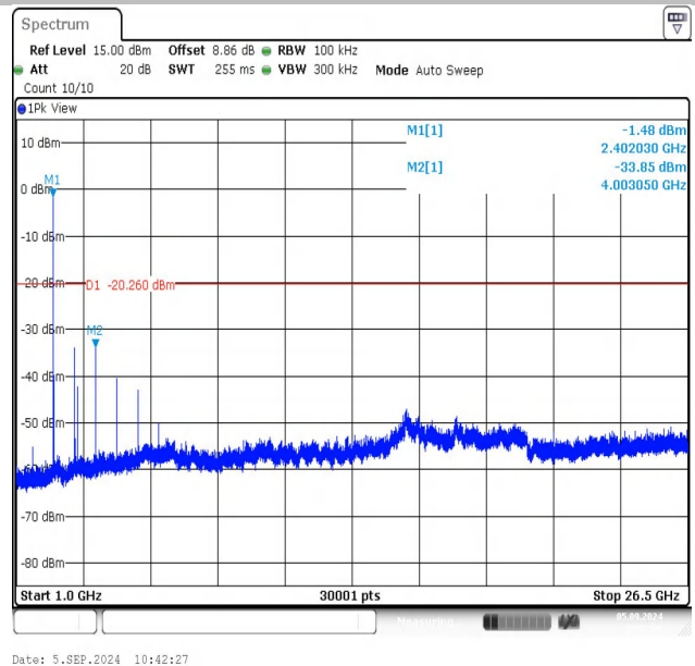
2DH5-Ant1-2402-1000~26500-PASS
