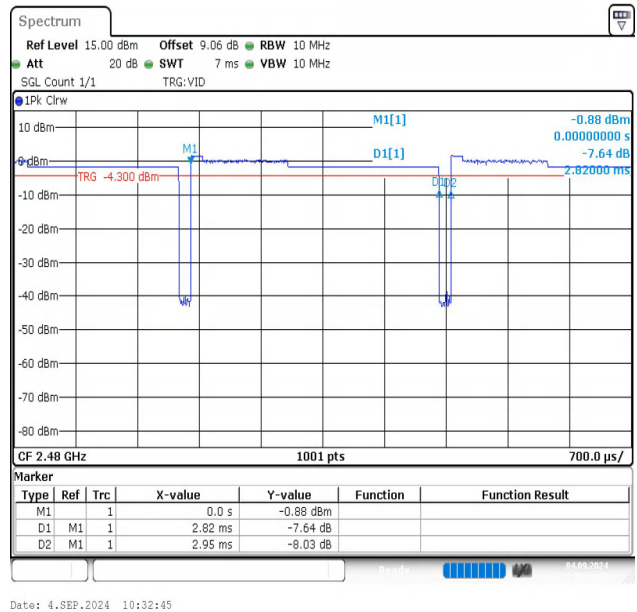
NTVN-2DH5-Ant1-2480
