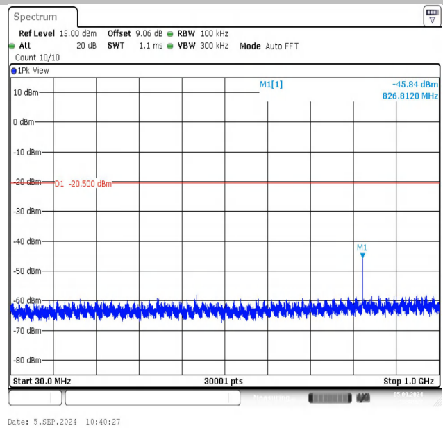
DH5-Ant1-2480-30~1000-PASS
