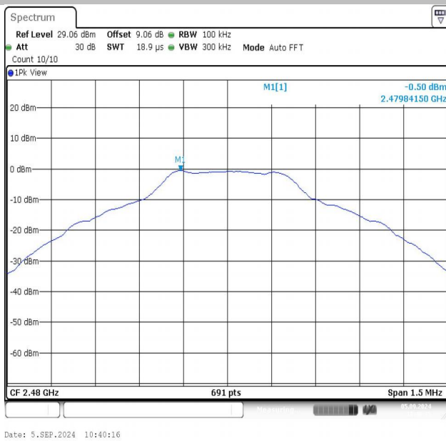
DH5-Ant1-2480-0~Reference-PASS
