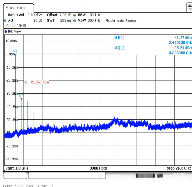
2DH5-Ant1-2480-1000~26500-PASS
