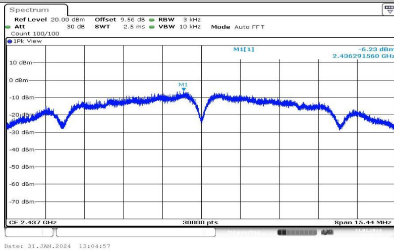
11B-Ant1-2437--6.23-0.00-0.00-0.00
