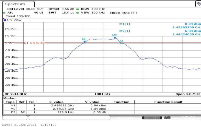
BLE_1M-Ant1-2440
