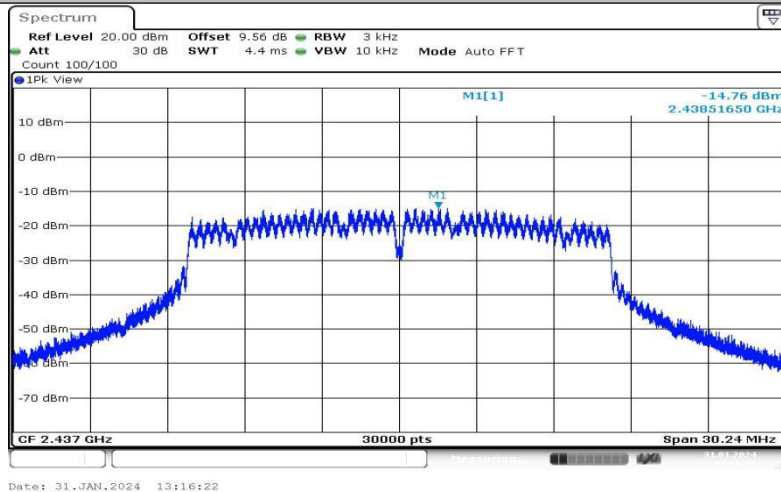
11G-Ant1-2437--14.76-0.00-0.00-0.00
