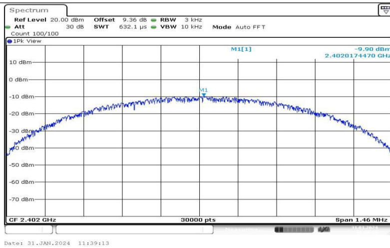
BLE_1M-Ant1-2402--9.90-0.00-0.00-0.00
