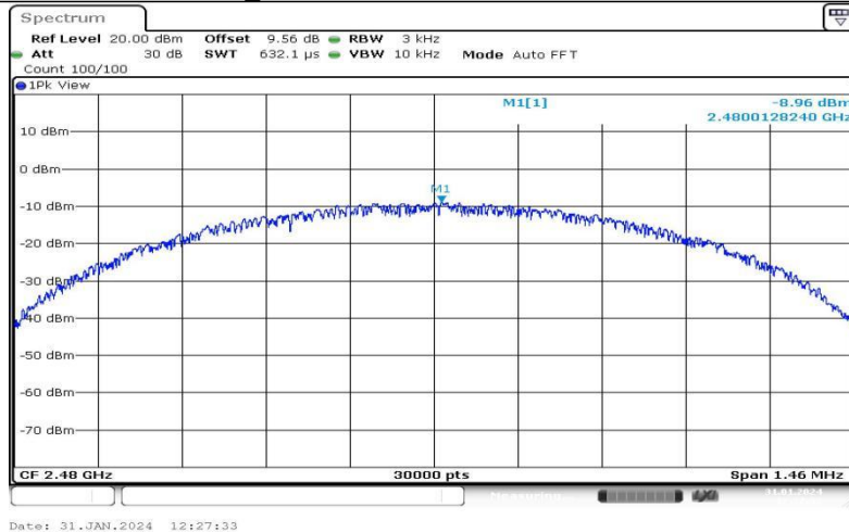
BLE_1M-Ant1-2480--8.96-0.00-0.00-0.00
