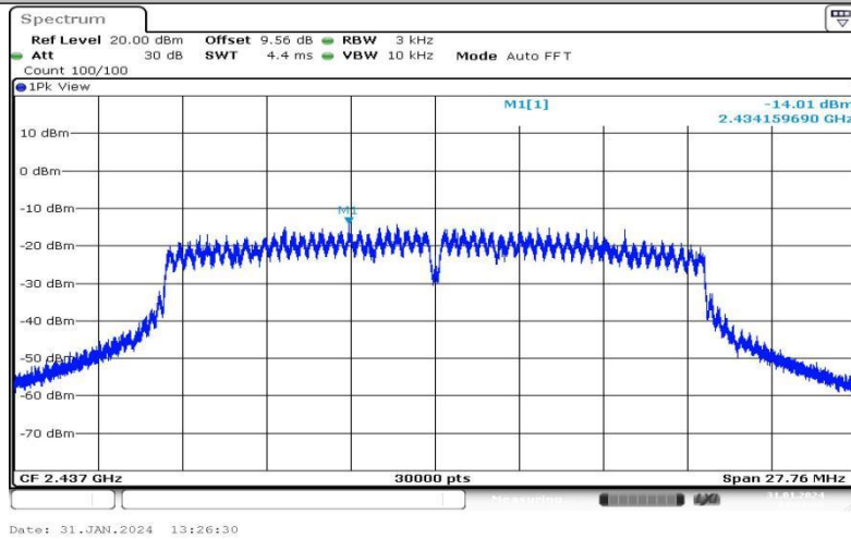
11N20SISO-Ant1-2437--14.01-0.00-0.00-0.00
