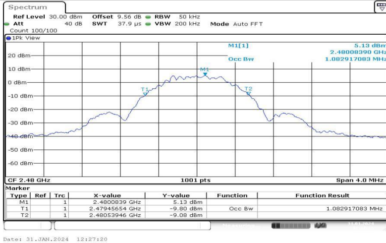
BLE_1M-Ant1-2480
