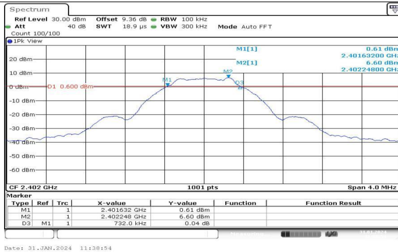
BLE_1M-Ant1-2402
