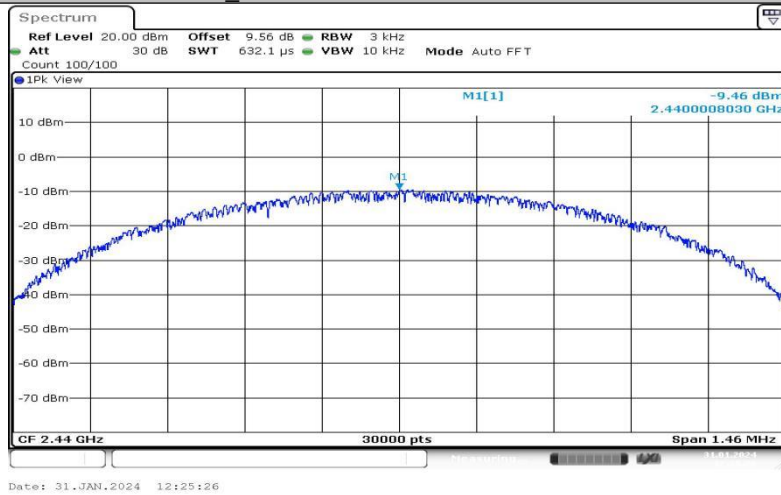
BLE_1M-Ant1-2440--9.46-0.00-0.00-0.00
