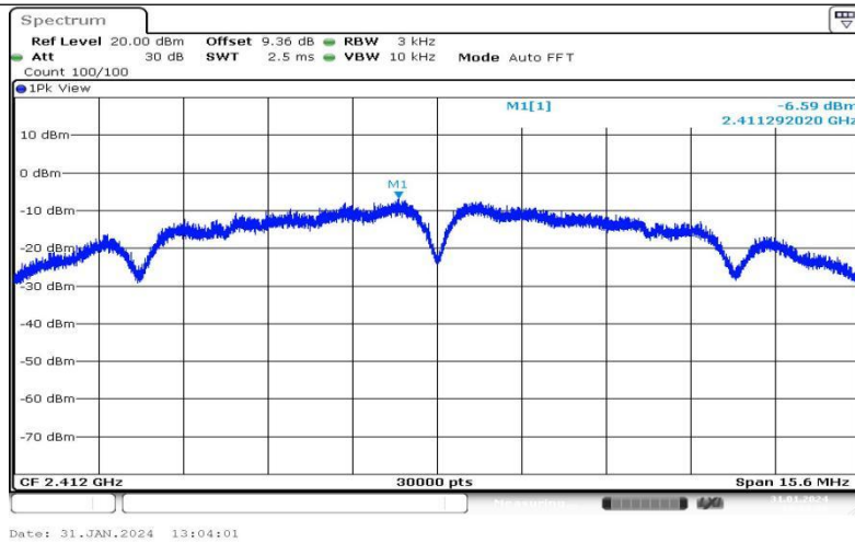
11B-Ant1-2412--6.59-0.00-0.00-0.00
