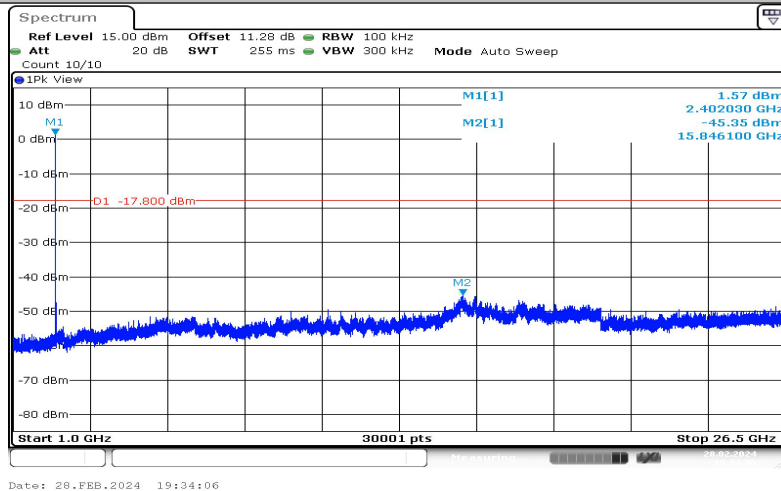
3DH5-Ant1-2402-1000~26500-2.20
