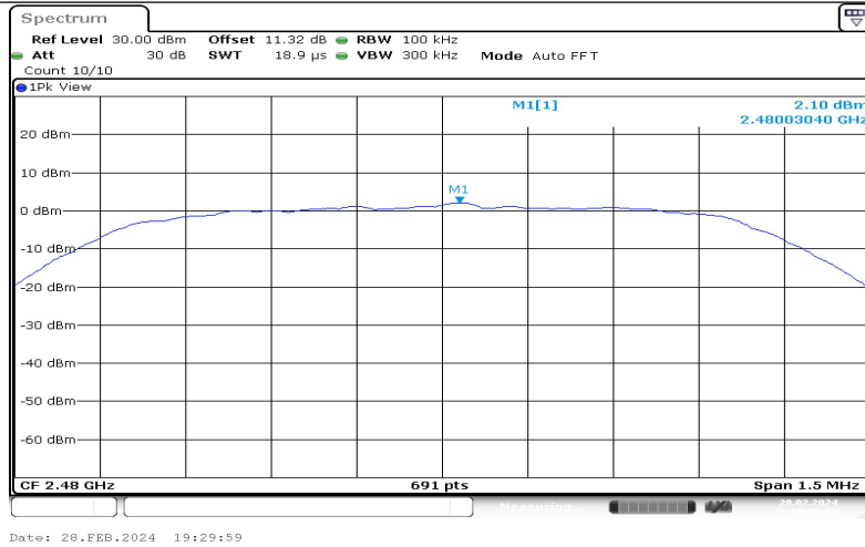
2DH5-Ant1-2480-0~Reference-2.10
