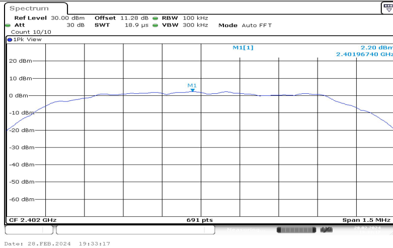
3DH5-Ant1-2402-0~Reference-2.20
