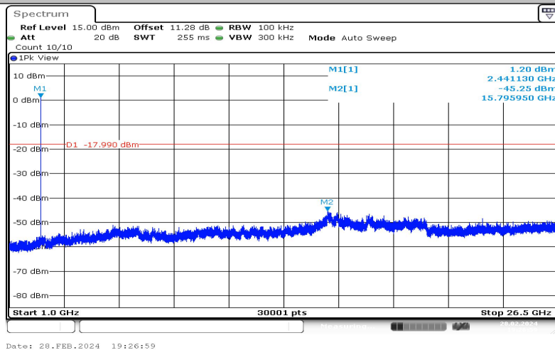
2DH5-Ant1-2441-1000~26500-2.01
