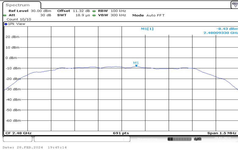
3DH5-Ant1-2480-0~Reference--8.43
