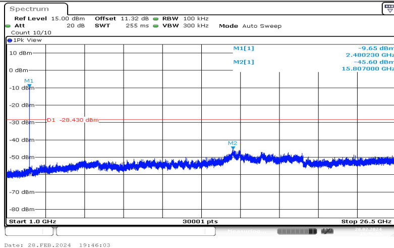
3DH5-Ant1-2480-1000~26500--8.43
