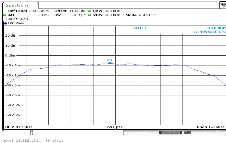
3DH5-Ant1-2441-0~Reference--8.16
