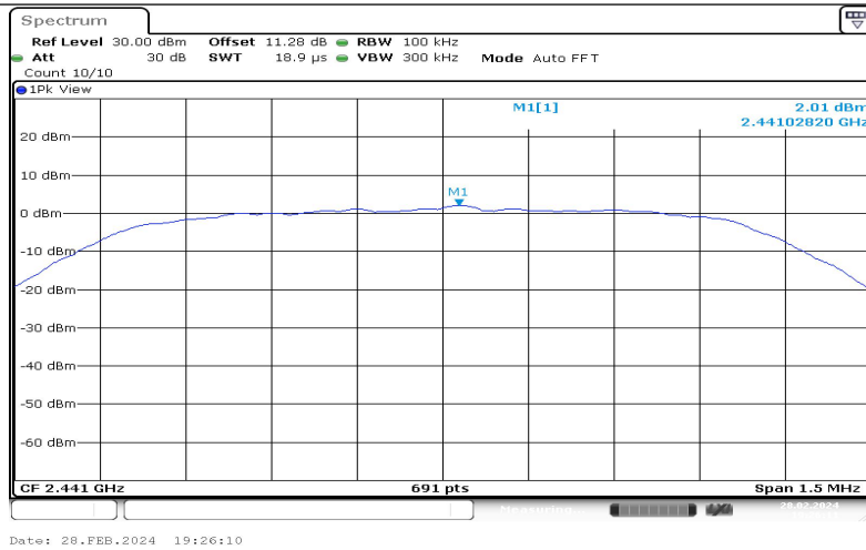
2DH5-Ant1-2441-0~Reference-2.01
