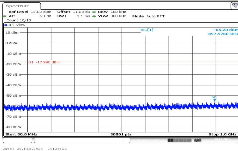
2DH5-Ant1-2441-30~1000-2.01
