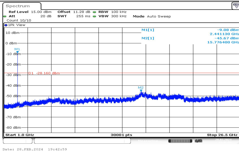
3DH5-Ant1-2441-1000~26500--8.16
