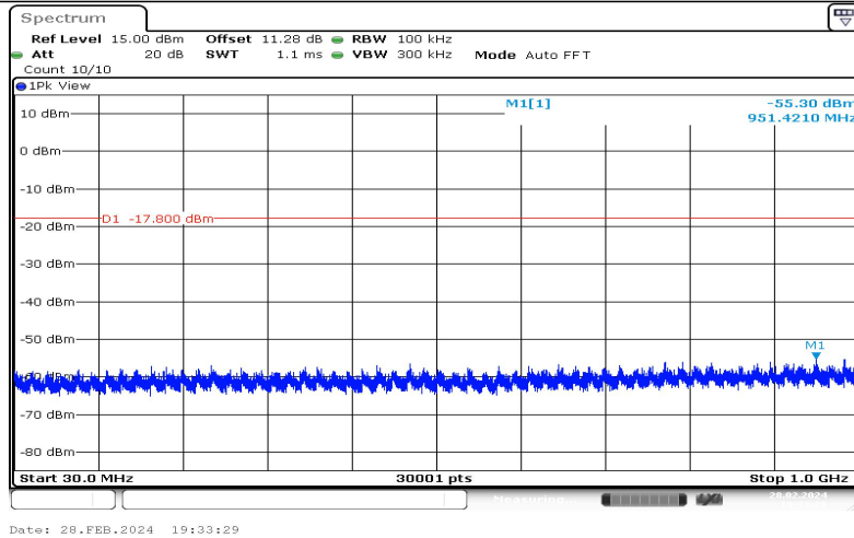
3DH5-Ant1-2402-30~1000-2.20
