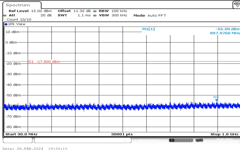
2DH5-Ant1-2480-30~1000-2.10
