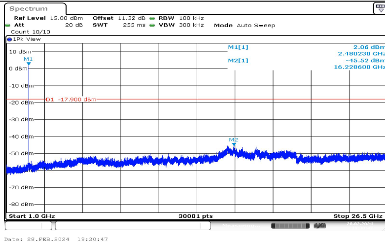
2DH5-Ant1-2480-1000~26500-2.10
