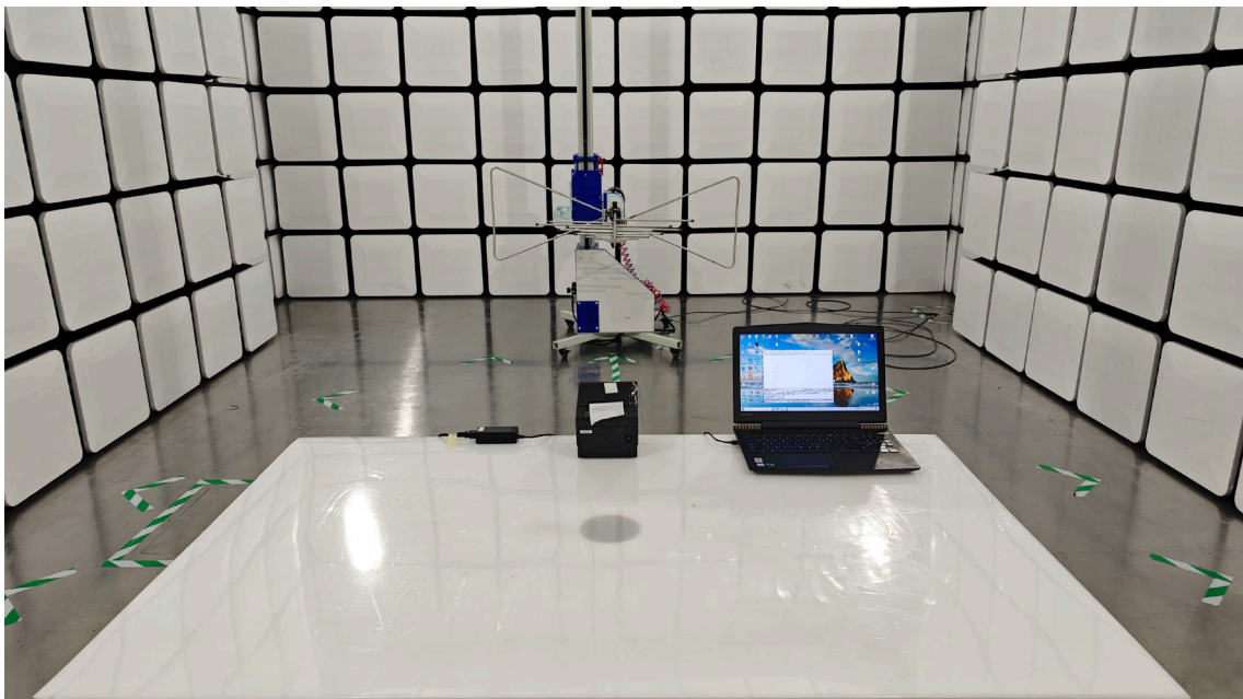
Radiated emission (30-1000MHz)
