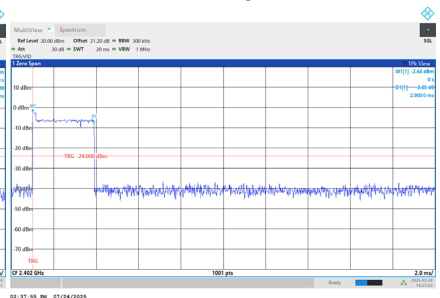
2DH5
