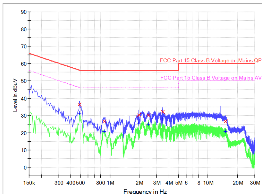
Conducted Emission Test FCC Part 15
