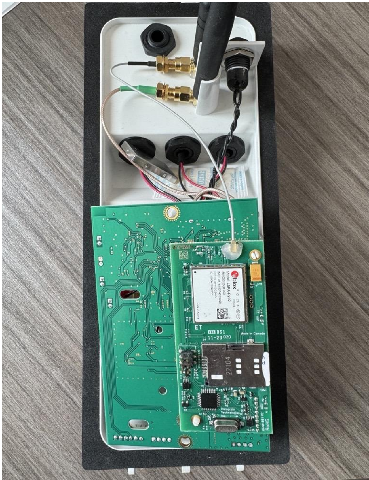
PCB underside assembled (flipped)
