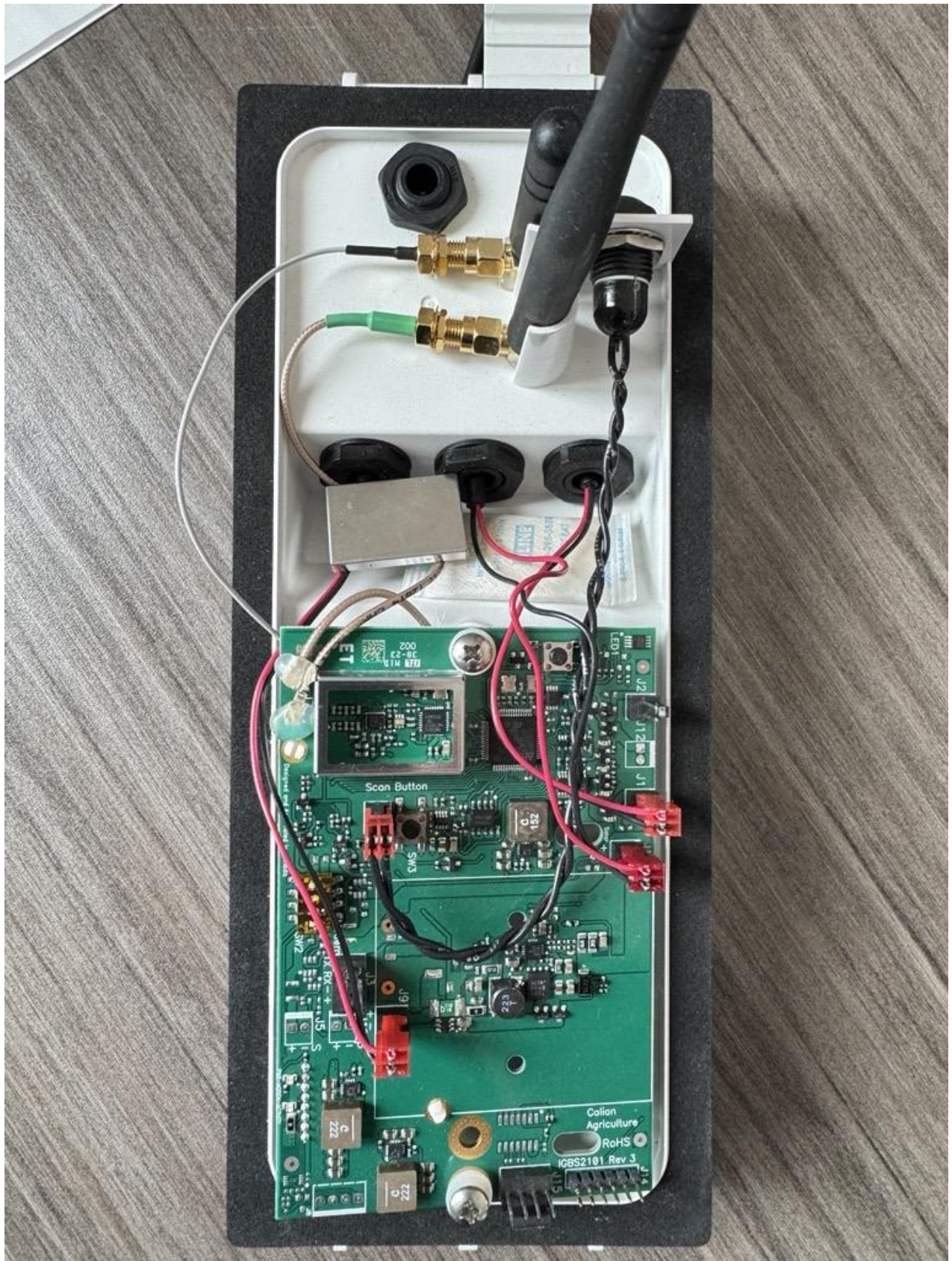
RF Shield Removed.
