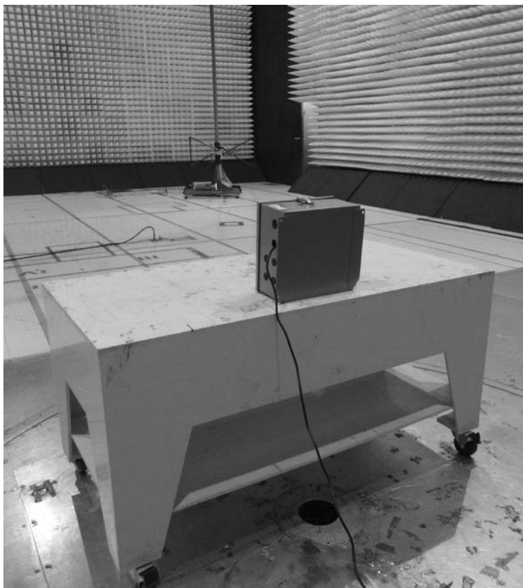
Electromagnetic Radiated Disturbance Setup Photograph
