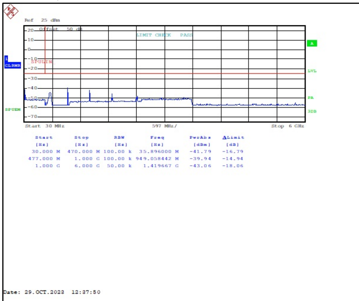
Plot 5-1: Spurious Emissions at Antenna Terminals – 473.0 MHz
