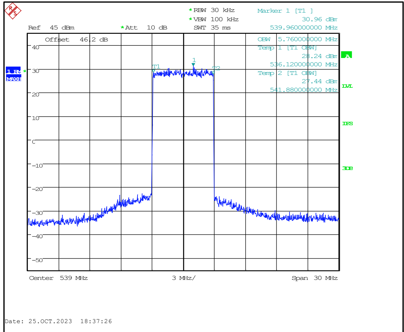
Plot 7-16: 99% Occupied Bandwidth – 539.0 MHz
