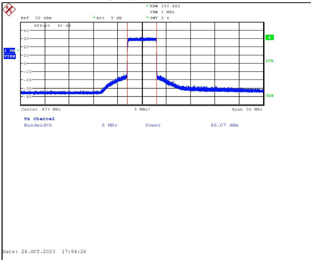
Plot 4-1: RF Conducted Average Output Power – 473.0 MHz
