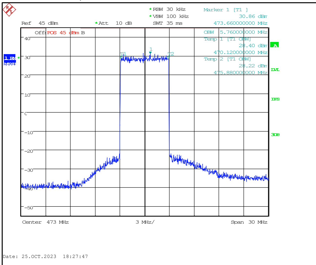
Plot 7-15: 99% Occupied Bandwidth – 473.0 MHz
