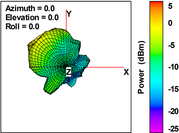
Total Power
