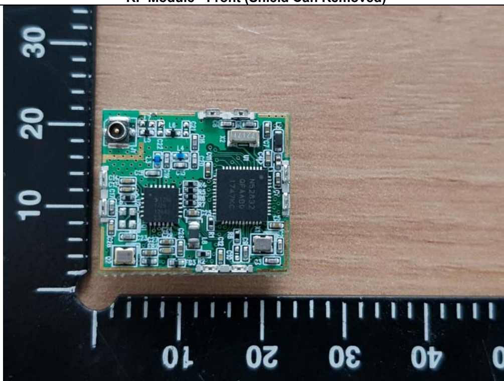
RF Module - Front (Shield Can Removed)
