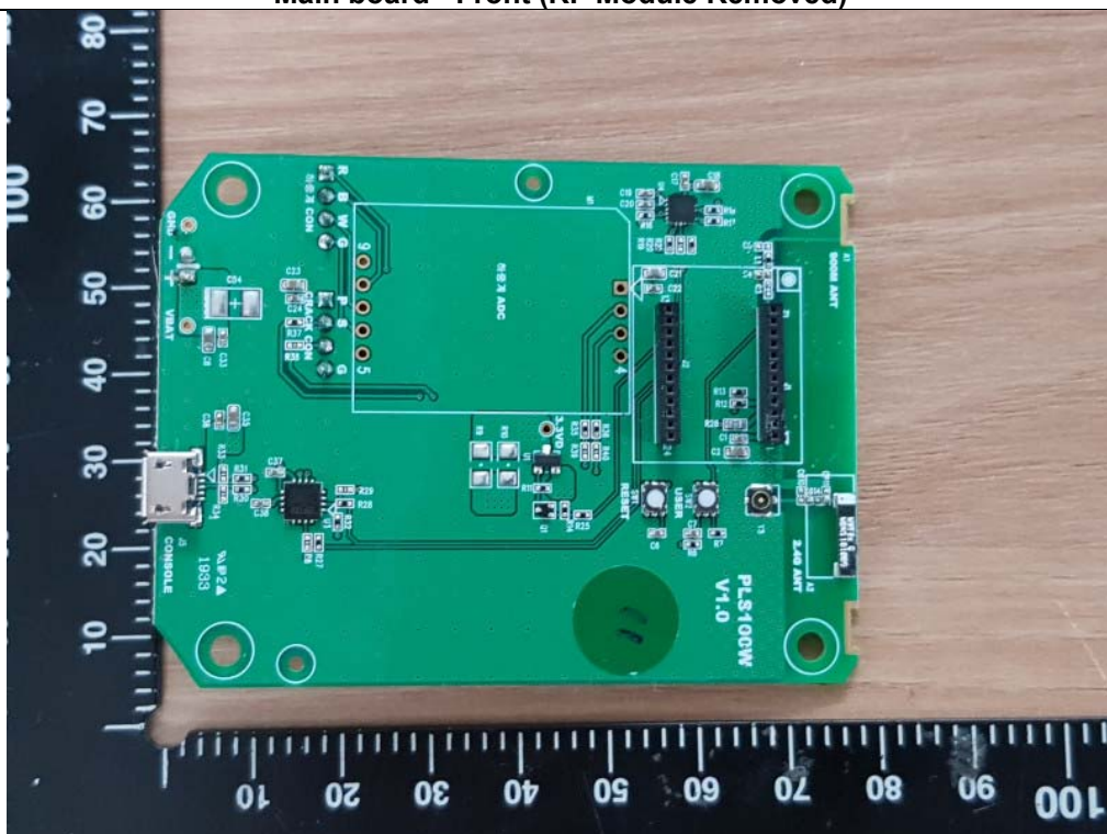
Main board - Front (RF Module Removed)
