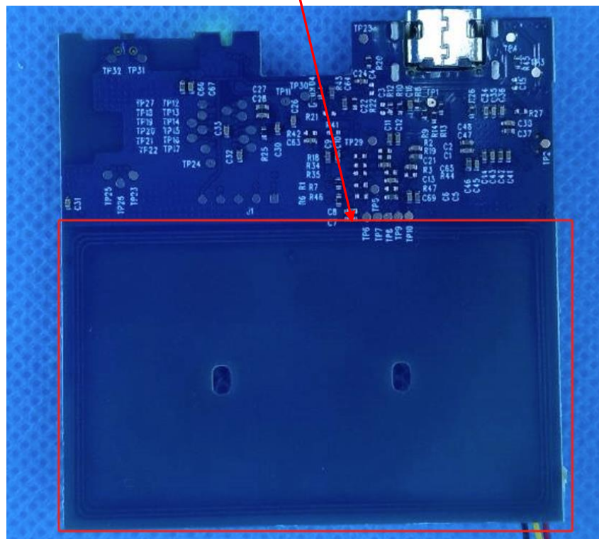
View of NFC antenna
