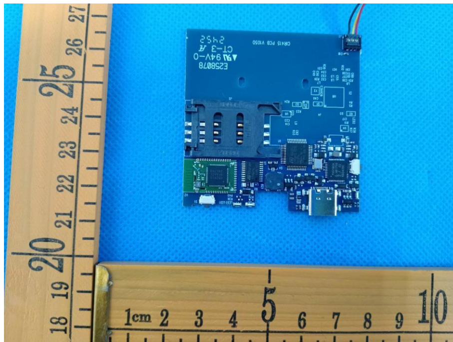
Inner circuit view
