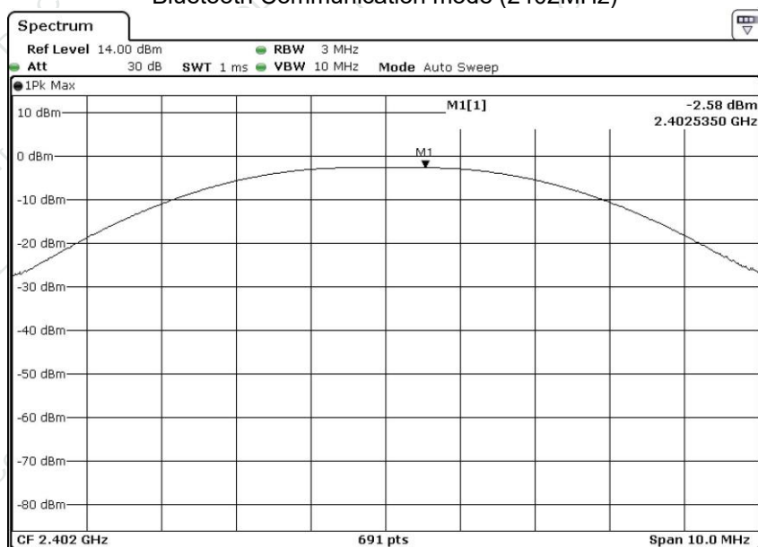
Test plot of Maximum Peak Conducted Output Power : Bluetooth Communication mode (2402MHz)
