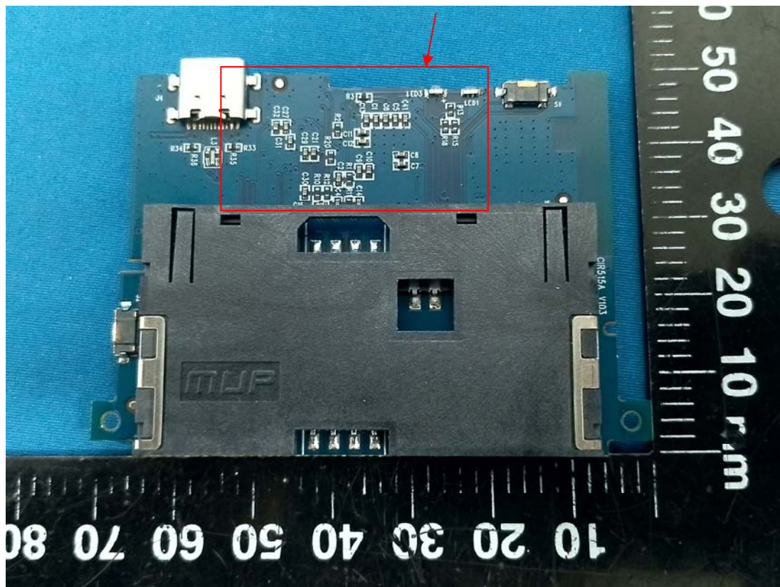
smartcard interface IC: STMicroelectronics ST8024
