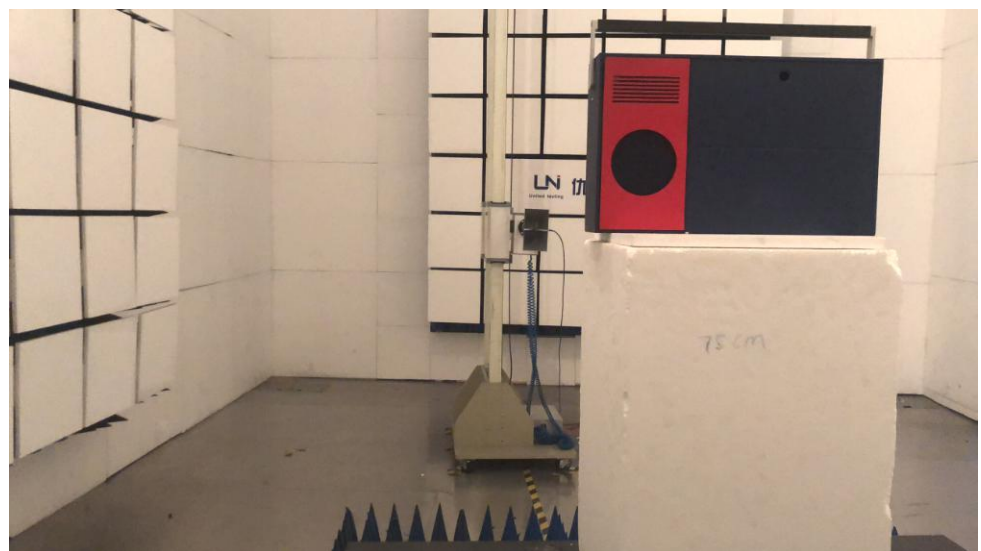
Radiated Emission (Above 1G)
