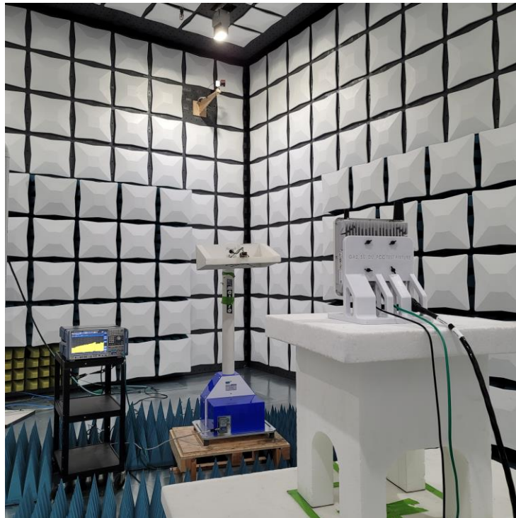
Setup 6. Test Setup 18-40GHz – DU
