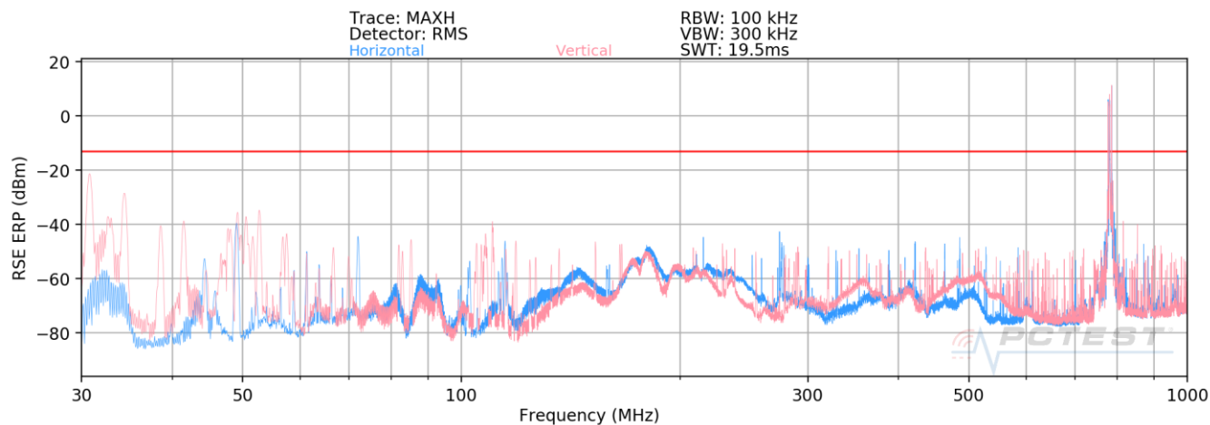
Plot 7-9. HBF Antenna Radiated Spurious Plot 30 MHz - 1 GHz (1CC QPSK Mid Channel H Beam)
