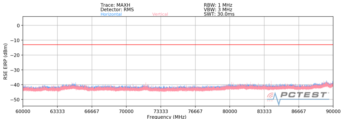
Plot 7-15. Radiated Spurious Plot 60-90 GHz (1CC QPSK Mid Channel H Beam)
