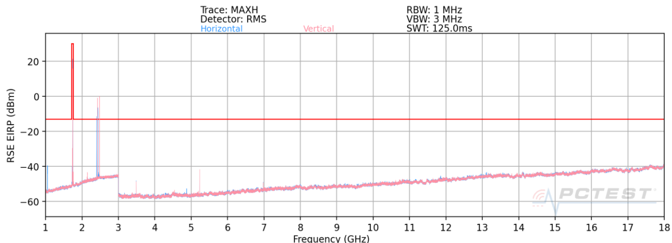
Plot 7-11. Radiated Spurious Plot 1-18 GHz (1CC QPSK Mid Channel H Beam) – B4
