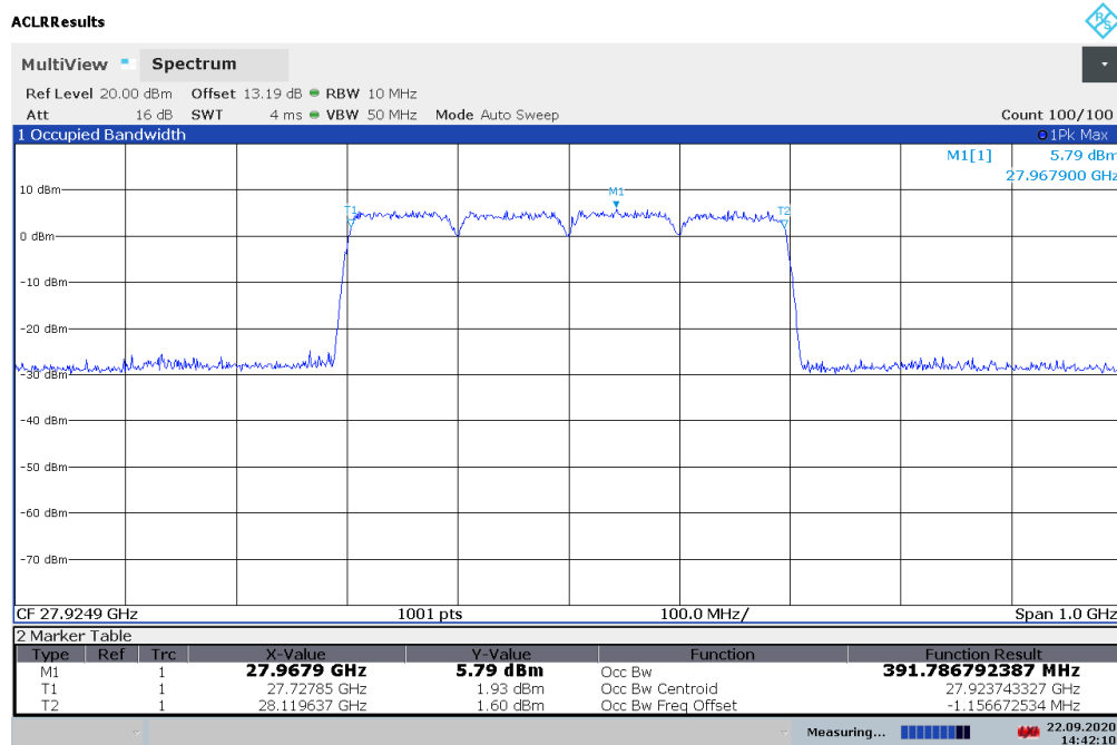
Plot 7-8. Occupied Bandwidth Plot - HBF Antenna (400MHz 4CC- 16QAM - Mid Channel) – V
