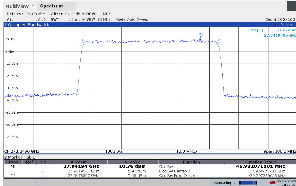
Plot 7-3. Occupied Bandwidth Plot - HBF Antenna (50MHz - QPSK - Mid Channel) – V
