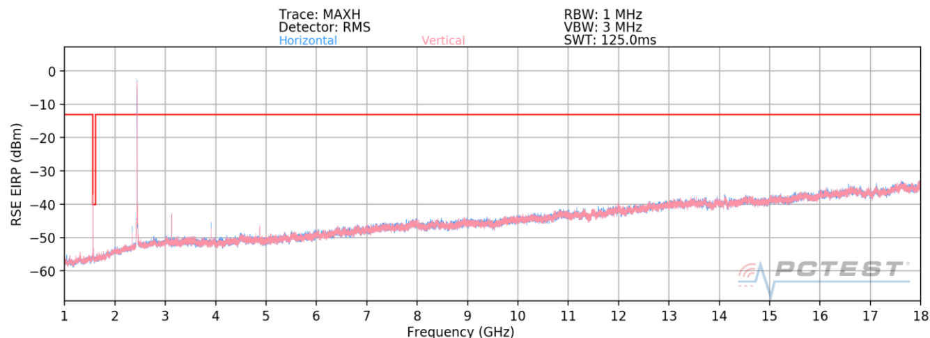
Plot 7-10. Radiated Spurious Plot 1-18 GHz (1CC QPSK Mid Channel H Beam) – B13
