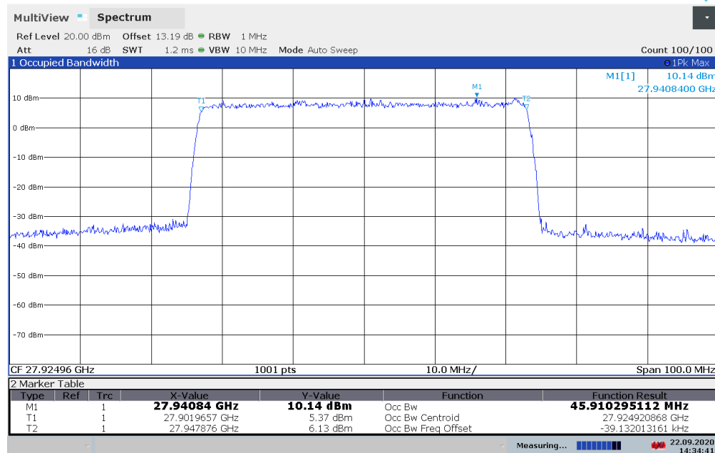
Plot 7-4. Occupied Bandwidth Plot - HBF Antenna (50MHz - 16QAM - Mid Channel) – V
