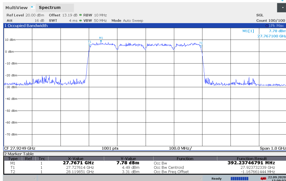
Plot 7-6. Occupied Bandwidth Plot - HBF Antenna (400MHz 4CC- 16QAM - Mid Channel) – H
