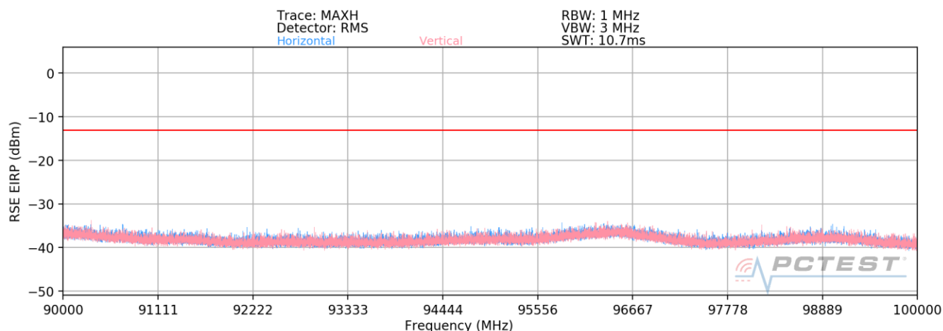
Plot 7-16. Radiated Spurious Plot 90-100 GHz (1CC QPSK Mid Channel H Beam)
