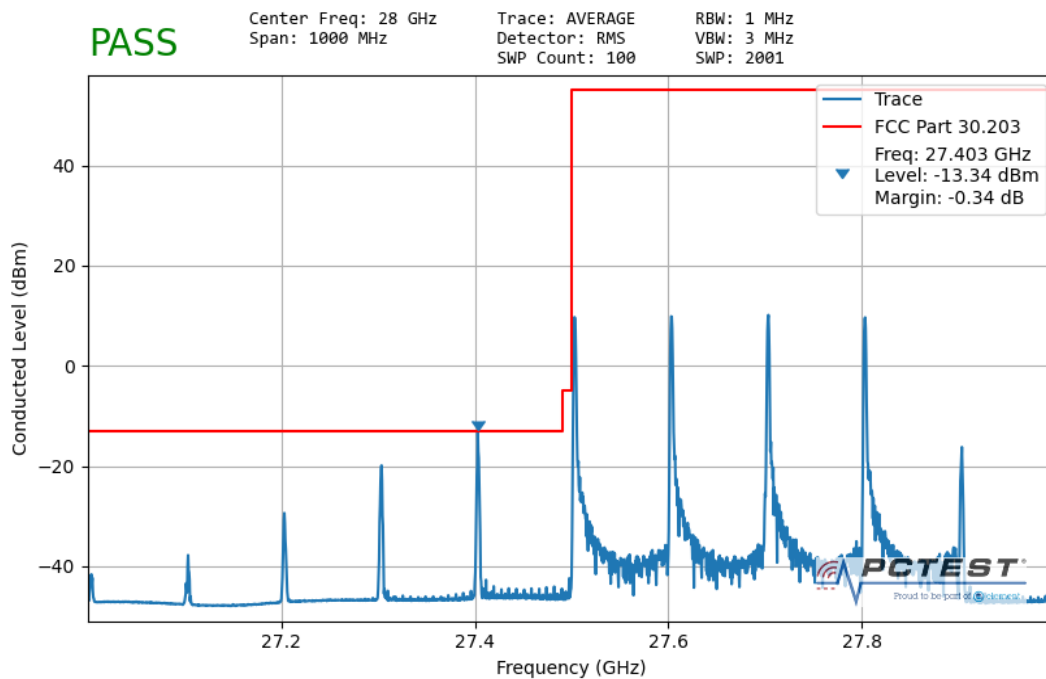
Plot 7-22. Lower Band Edge Plot (100MHz 4CC QPSK 1 RB)
