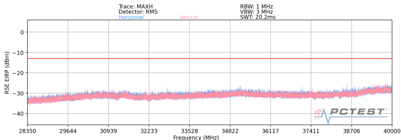
Plot 7-13. Radiated Spurious Plot 28.35-40 GHz (1CC QPSK Mid Channel H Beam)
