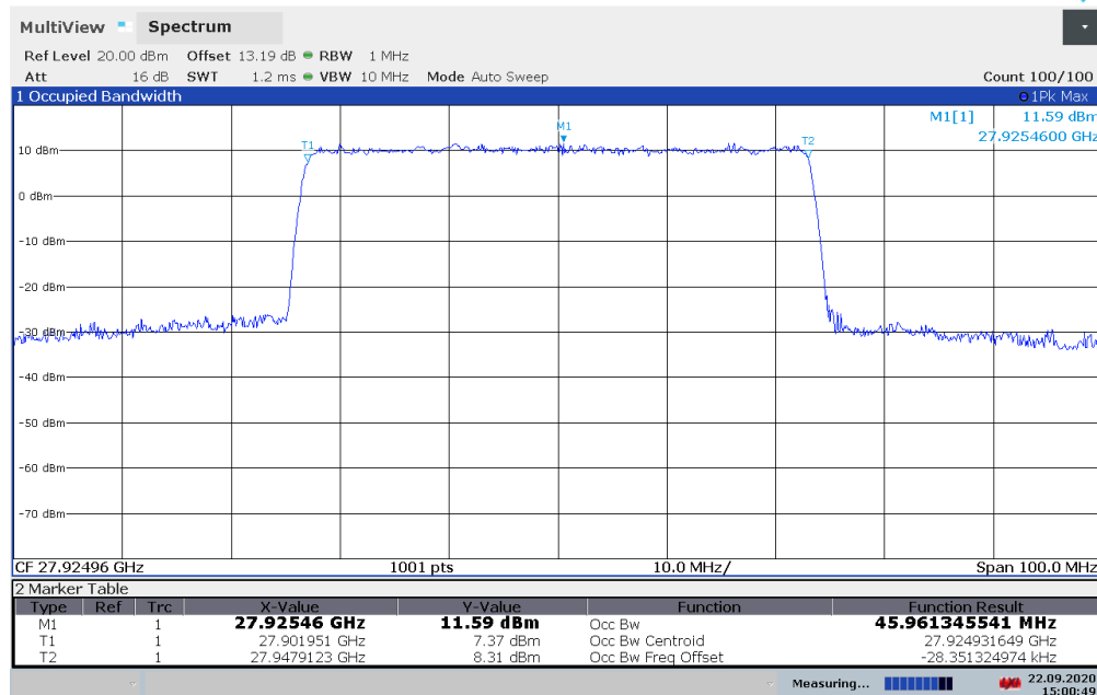
Plot 7-2. Occupied Bandwidth Plot - HBF Antenna (50MHz - 16QAM - Mid Channel) – H
