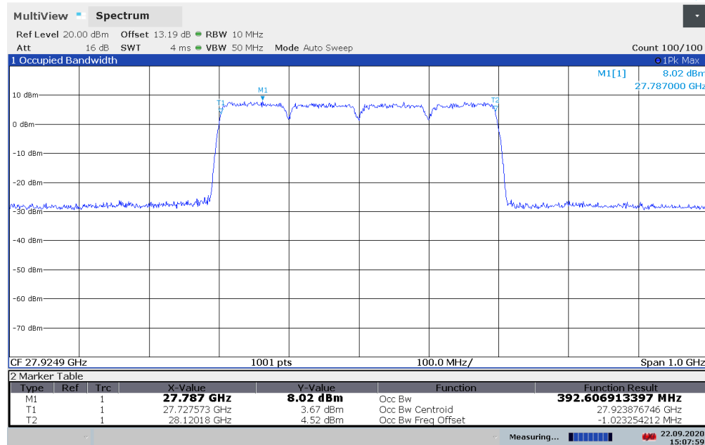
Plot 7-5. Occupied Bandwidth - HBF Antenna Plot (100MHz 4CC- QPSK - Mid Channel) – H
