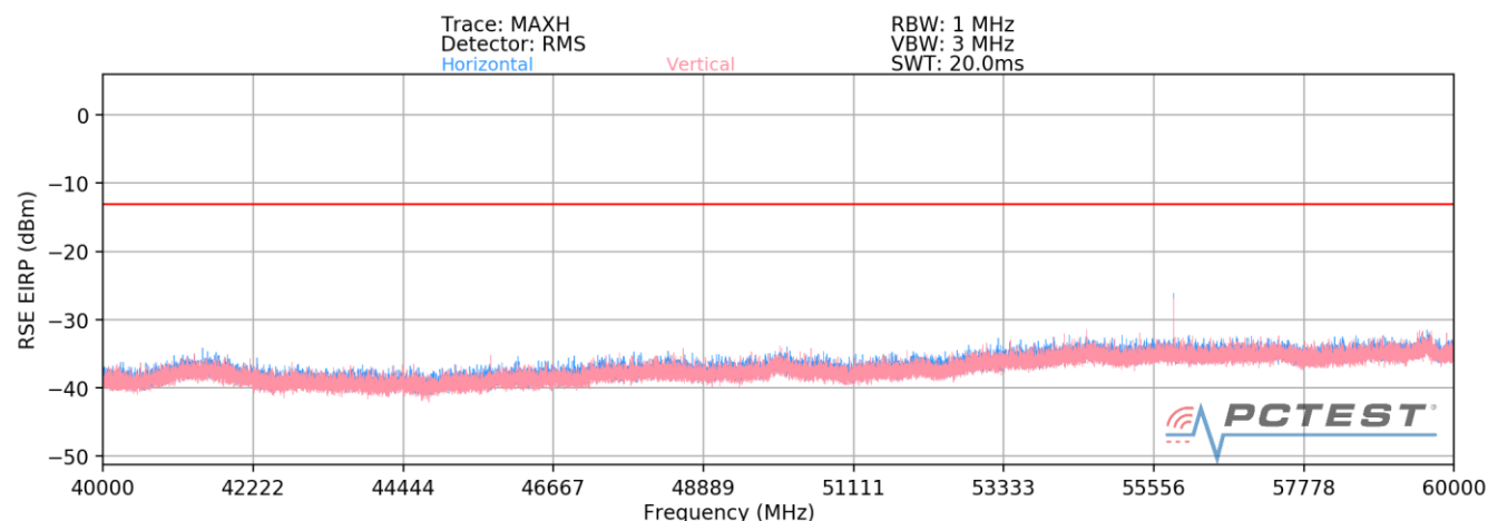
Plot 7-14. Radiated Spurious Plot 40-60 GHz (1CC QPSK Mid Channel H Beam)
