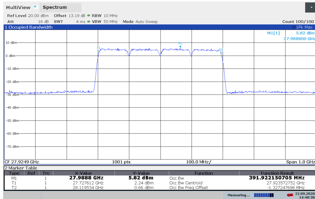
Plot 7-7. Occupied Bandwidth - HBF Antenna Plot (100MHz 4CC- QPSK - Mid Channel) – V
