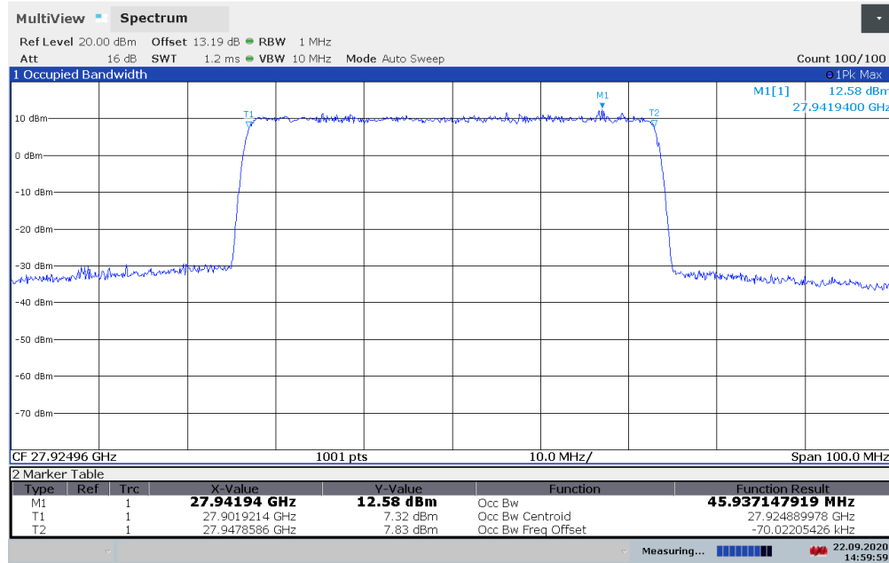
Plot 7-1. Occupied Bandwidth Plot - HBF Antenna (50MHz - QPSK - Mid Channel) – H
