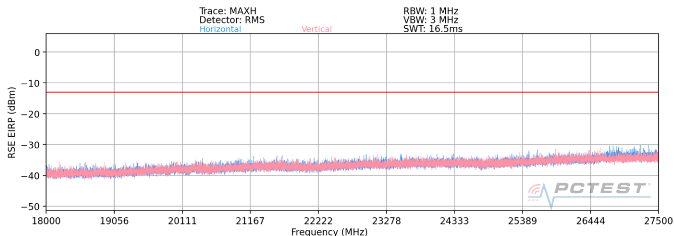
Plot 7-12. Radiated Spurious Plot 18-27.5 GHz (1CC QPSK Mid Channel H Beam)
