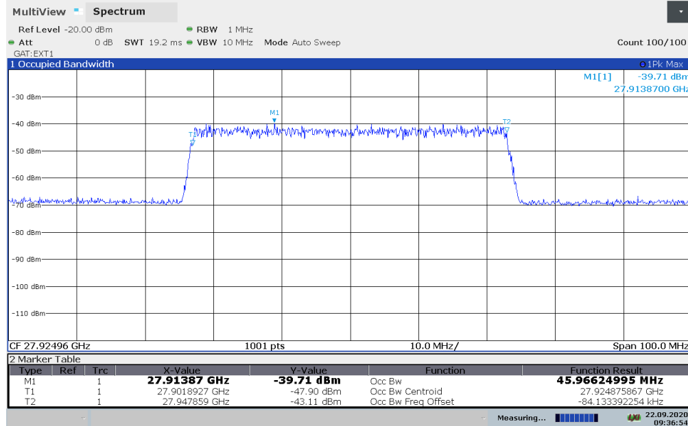
Plot 6-1. Occupied Bandwidth Input at 0.5dB below AGC Threshold.
