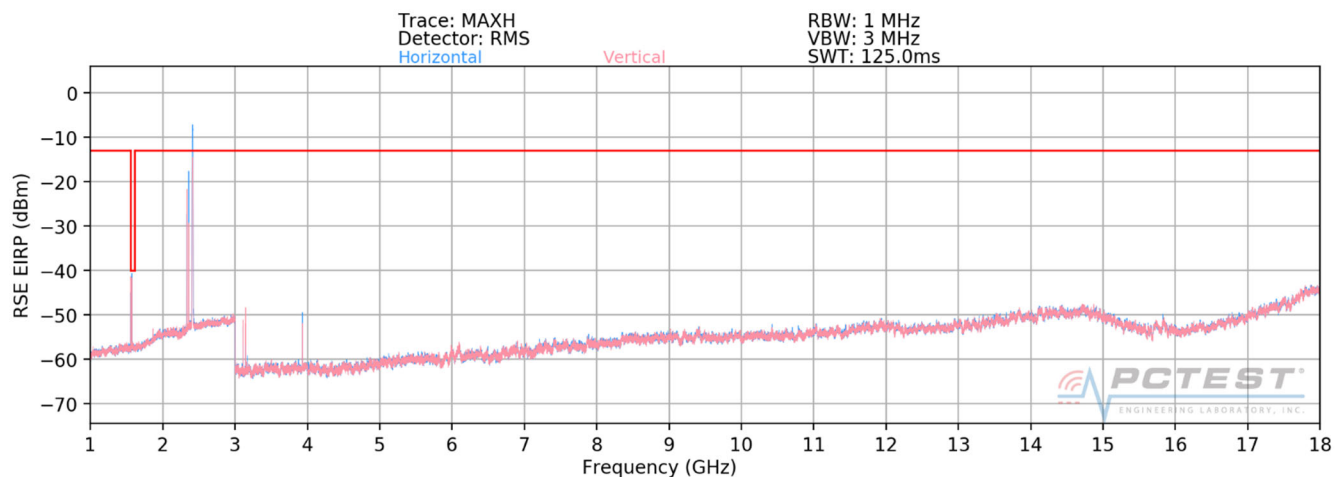
Plot 7-3. Band 13 - Radiated Spurious Emissions Plot <18GHz
