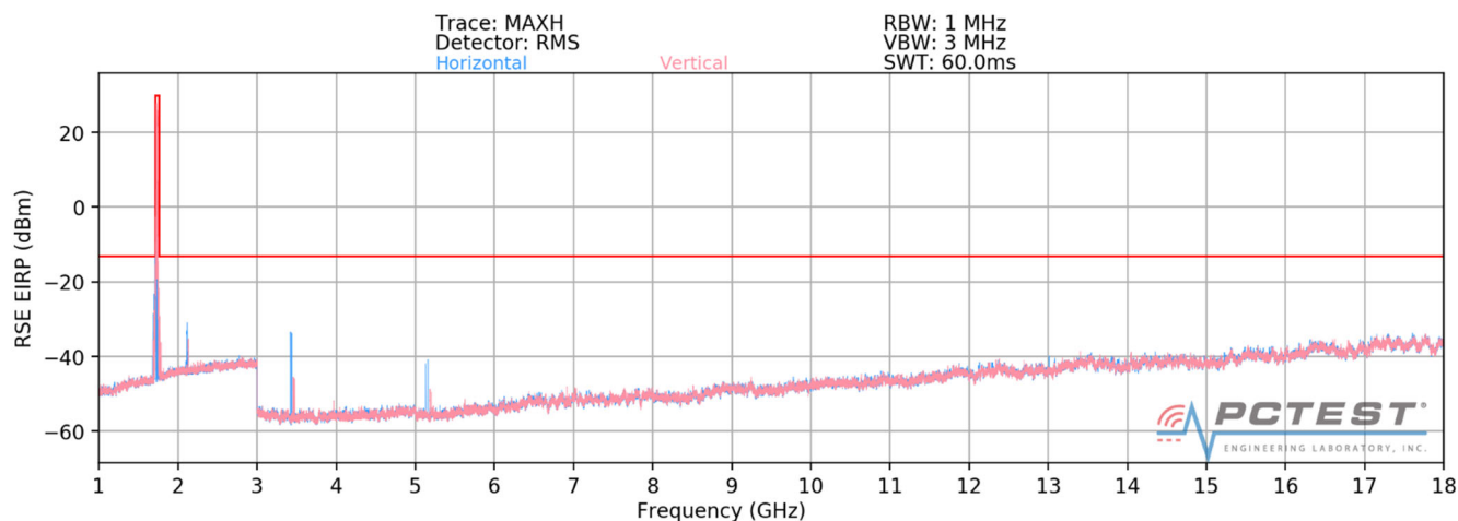
Plot 7-2. Radiated Spurious Plot above 1GHz (Band 4)
