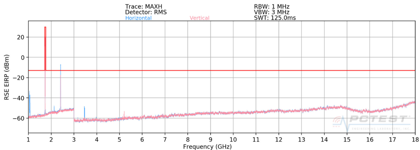
Plot 7-4. Band 4 - Radiated Spurious Emissions Plot <18GHz
