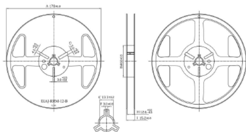
c. Reel Drawing
