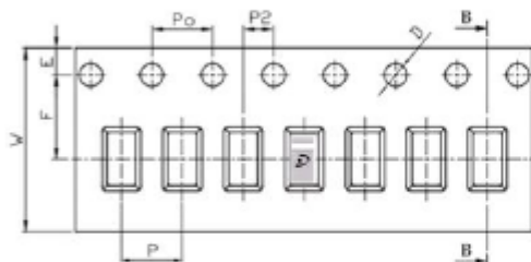
a. Tape Drawing
