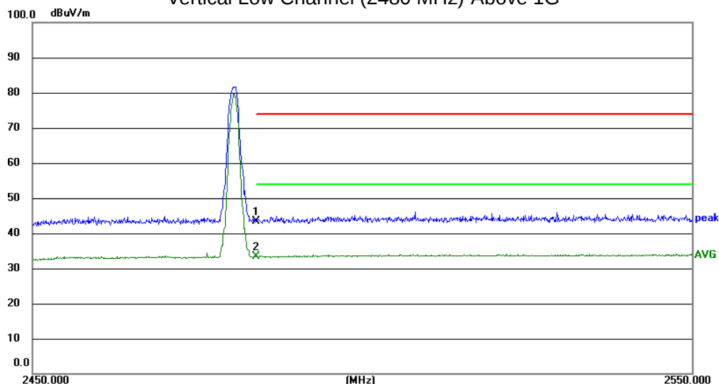
Vertical Low Channel (2480 MHz)-Above 1G
