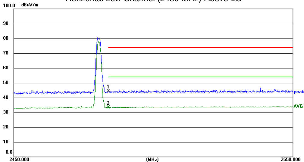
Horizontal Low Channel (2480 MHz)-Above 1G
