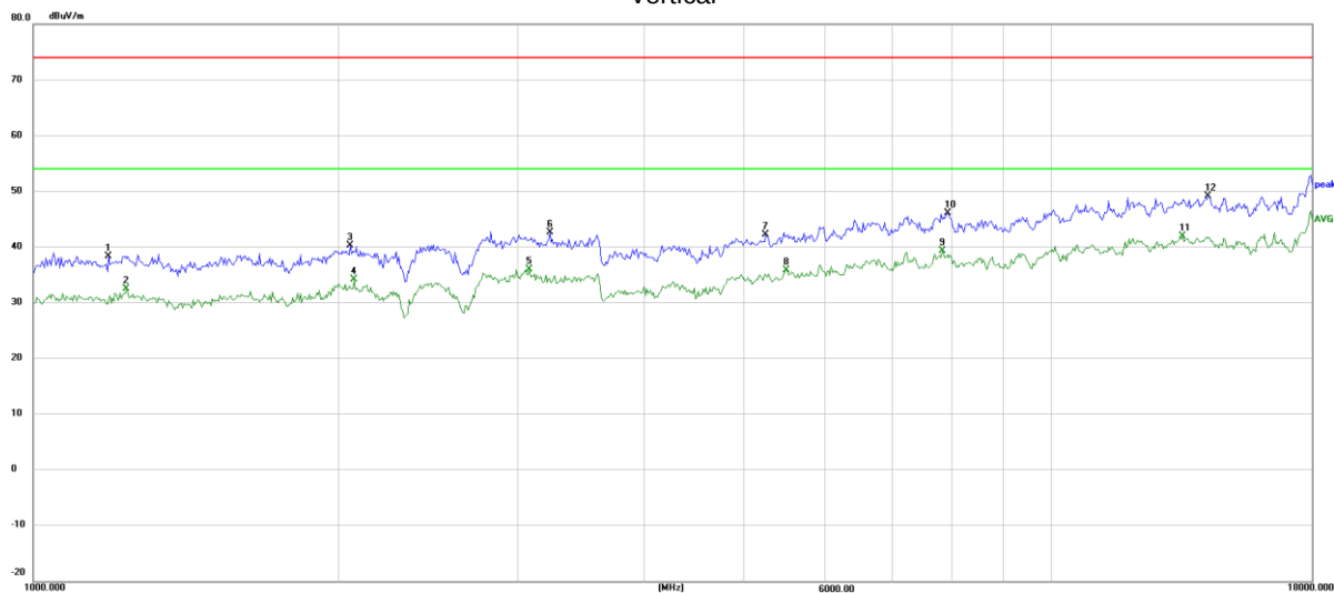
Low Channel (2402 MHz)(GFSK)--Above 1G Vertical
