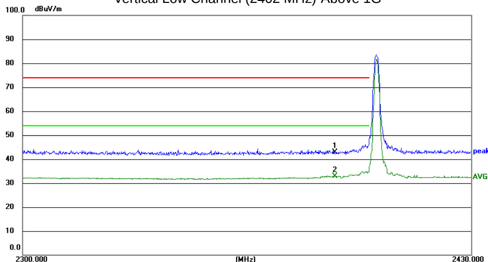
Vertical Low Channel (2402 MHz)-Above 1G
