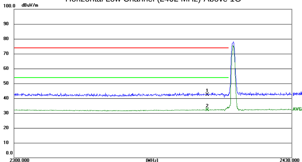
Horizontal Low Channel (2402 MHz)-Above 1G
