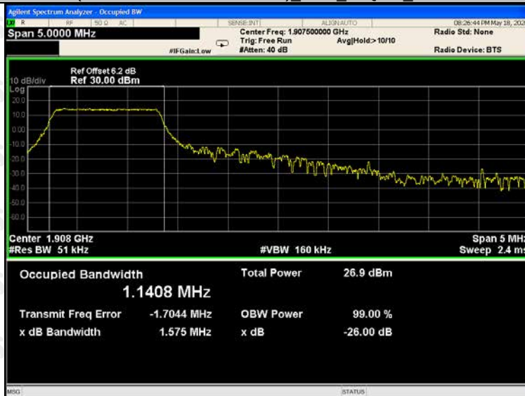
(Channel Bandwidth: 5 MHz) HCH_16QAM_5RB#0
