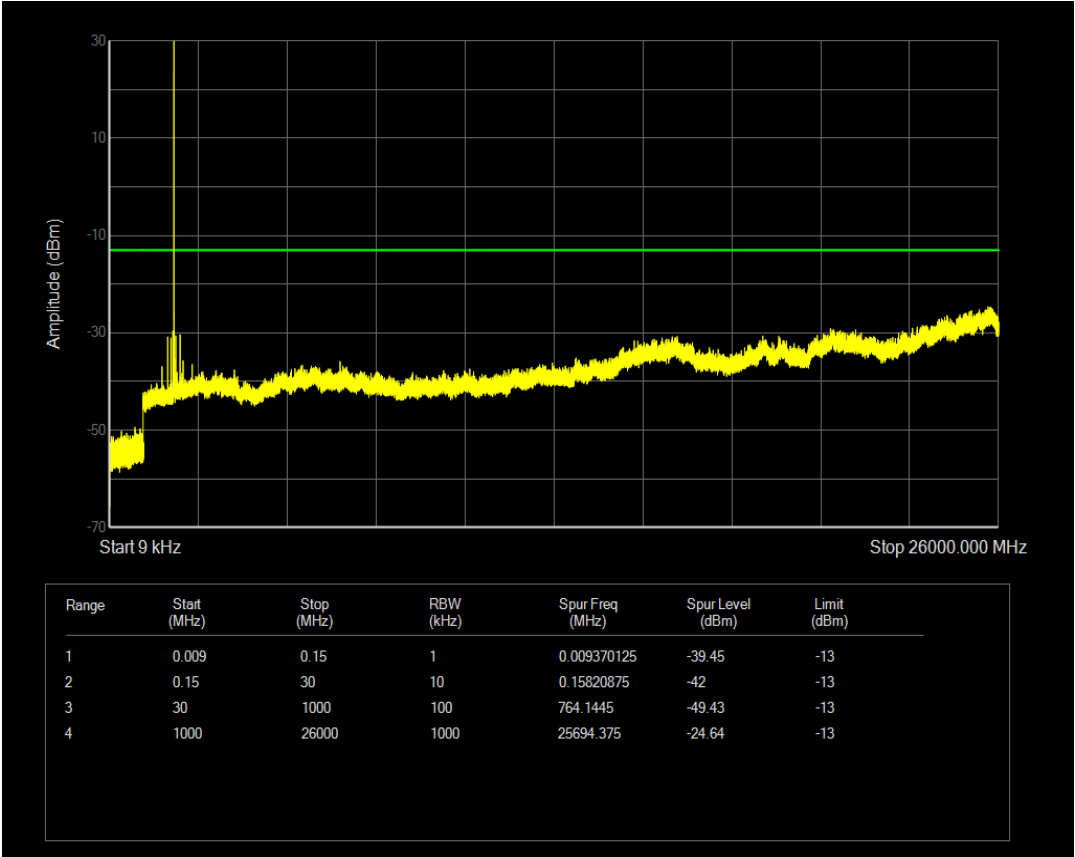
Band2 QAM16 BW=10MHz Channel=19150 RB Size=6 Position=#0 NB Index=0
