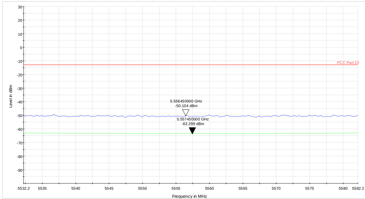
Harmonic 3
