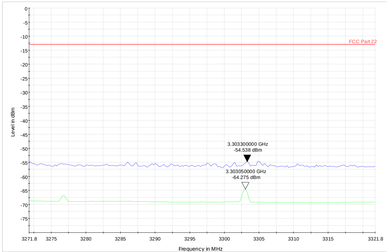
Harmonic 4
