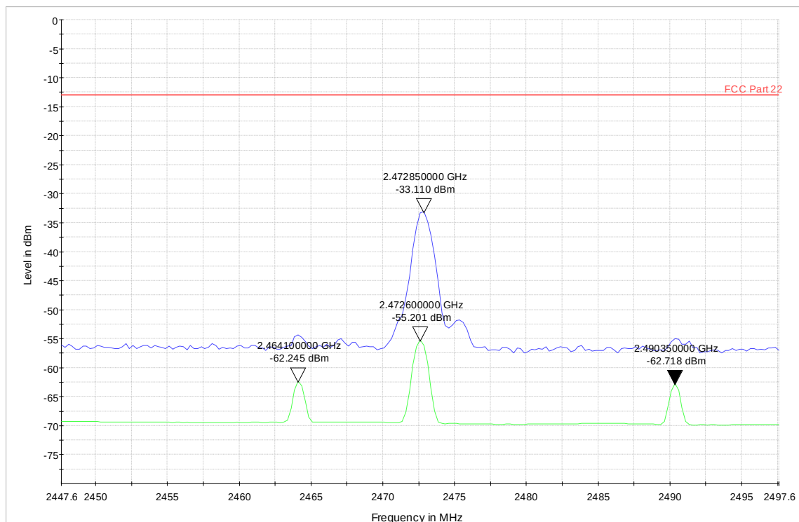
Harmonic 3
