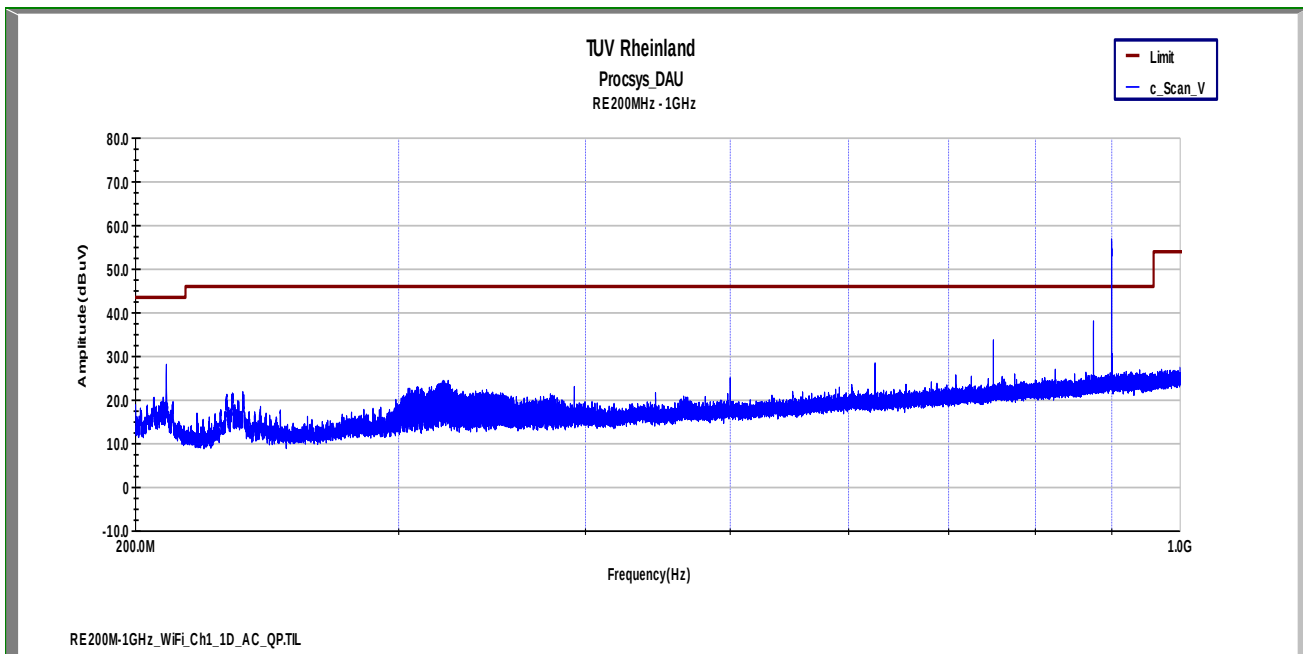
Horizontal polarization
