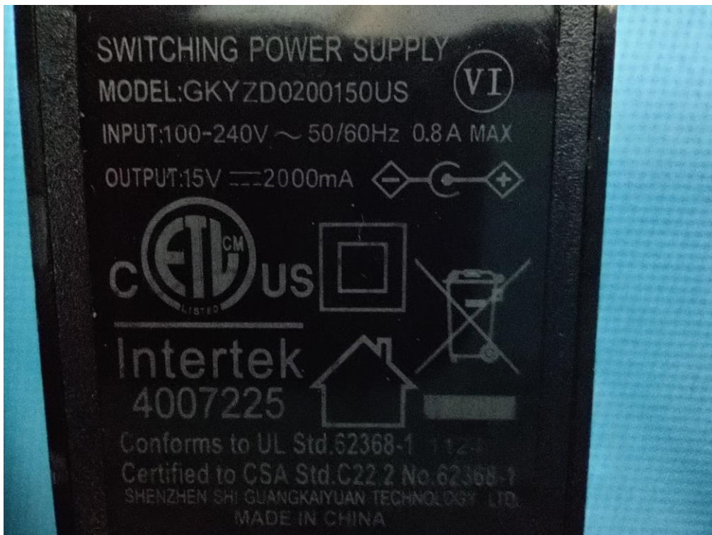
ADAPTER VIEW OF EUT(FIGURE 2)
