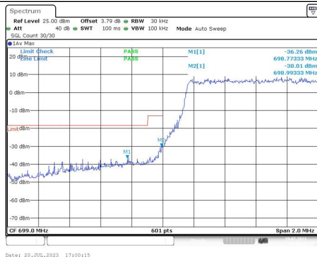
Band12-1.4MHz-16QAM-23173-1RB#0
