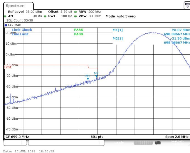
Band12-10MHz-16QAM-23060-1RB#49
