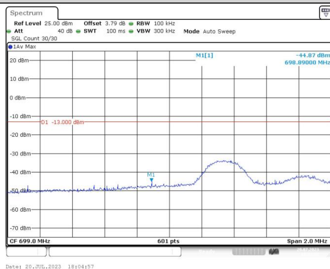
Band12-5MHz-16QAM-23035-25RB#0
