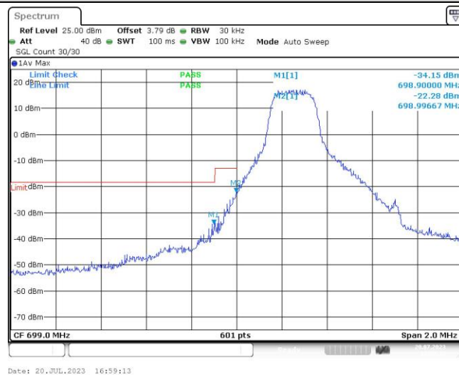
Band12-1.4MHz-QPSK-23017-1RB#5
