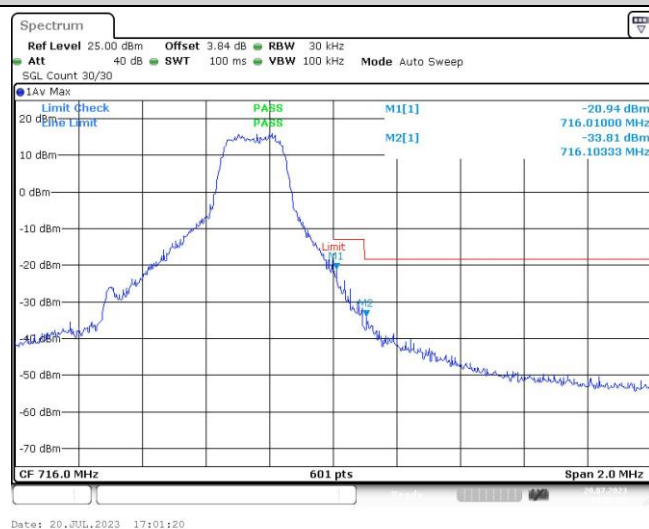
Band12-1.4MHz-16QAM-23173-6RB#0
