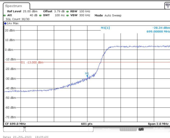
Band12-5MHz-16QAM-23155-1RB#0
