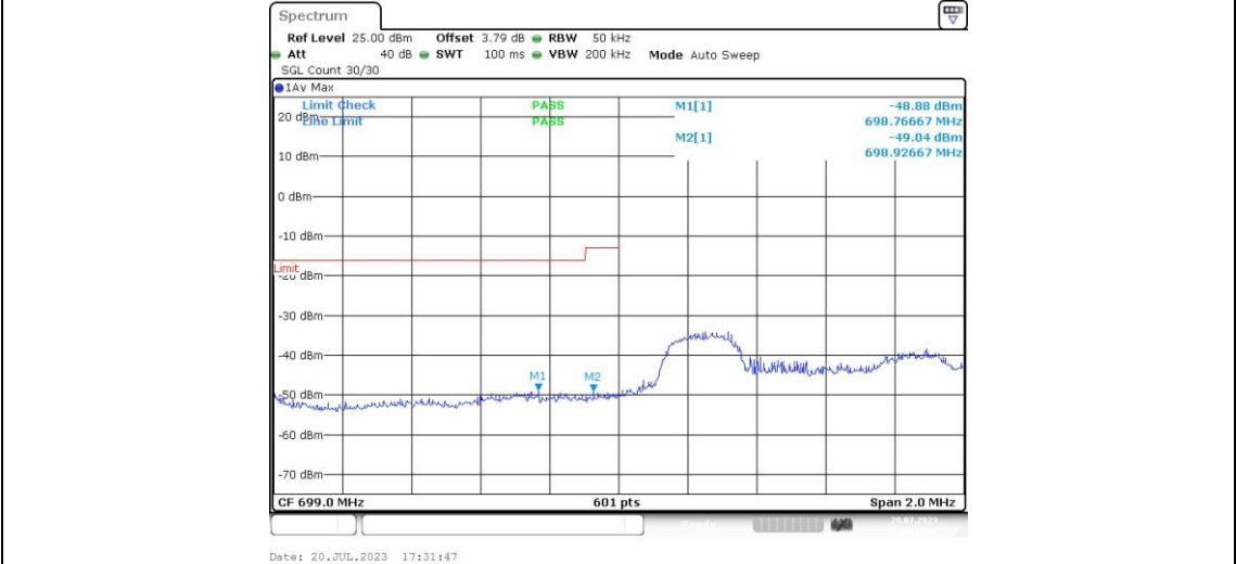
Band12-3MHz-QPSK-23025-15RB#0
