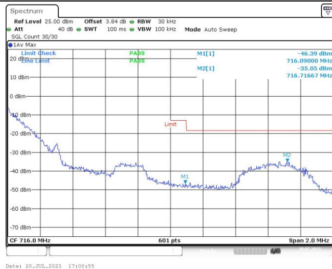
Band12-1.4MHz-16QAM-23173-1RB#5
