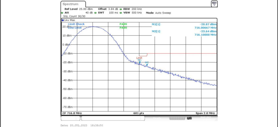
Band12-10MHz-16QAM-23130-50RB#0
