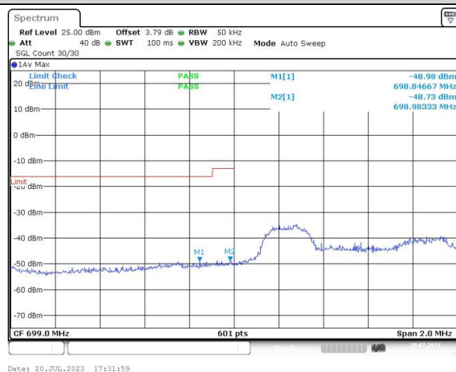
Band12-3MHz-16QAM-23025-15RB#0
