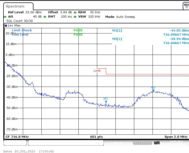
Band12-1.4MHz-QPSK-23173-1RB#5
