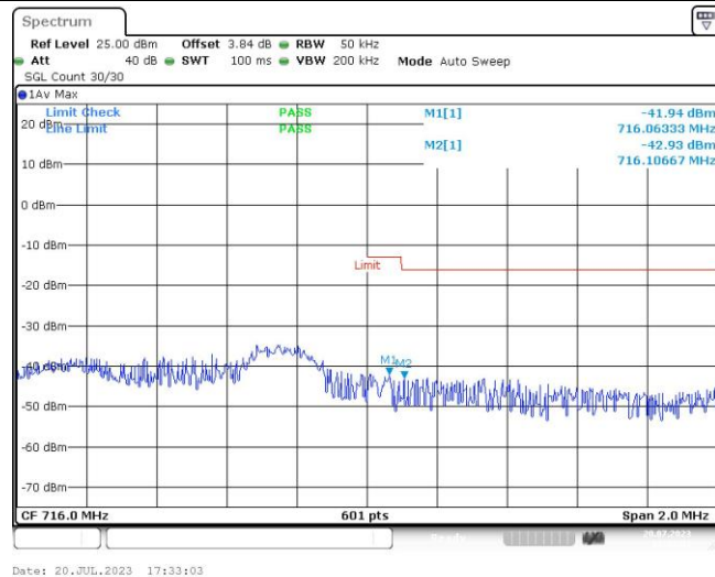
Band12-3MHz-16QAM-23165-1RB#14
