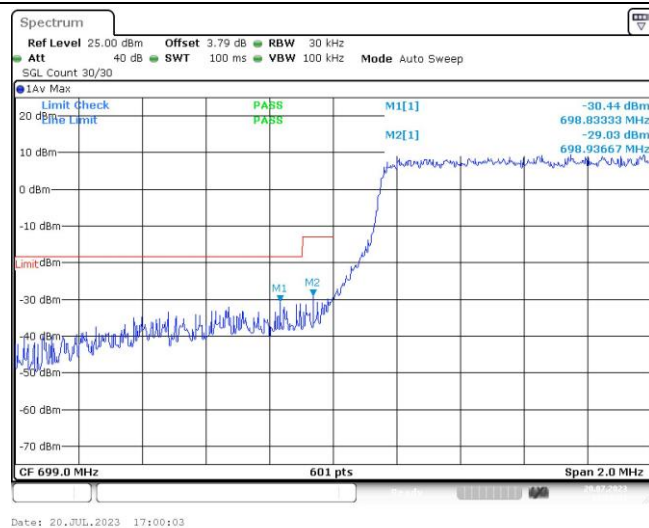
Band12-1.4MHz-QPSK-23173-1RB#0
