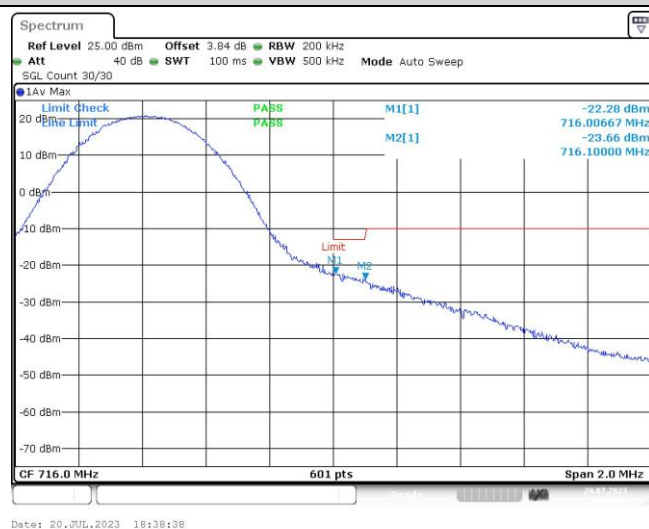
Band12-10MHz-QPSK-23130-50RB#0
