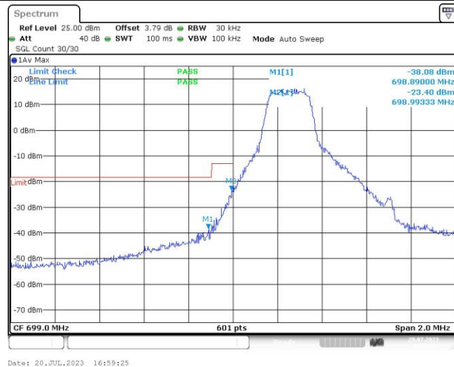
Band12-1.4MHz-16QAM-23017-1RB#5
