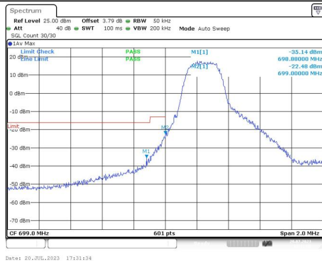
Band12-3MHz-16QAM-23025-1RB#14
