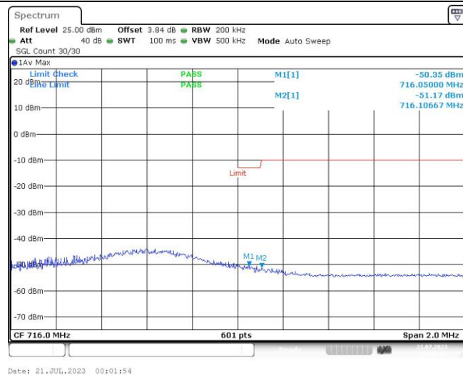
Band17-10MHz-QPSK-23800-1RB#49
