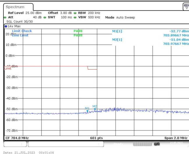
Band17-10MHz-16QAM-23780-50RB#0
