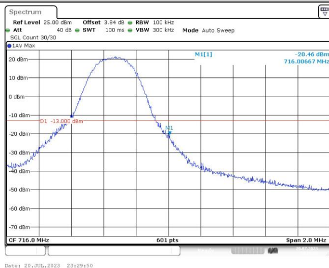
Band17-5MHz-16QAM-23825-25RB#0
