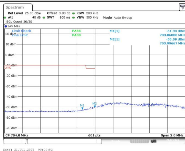
Band17-10MHz-QPSK-23780-50RB#0
