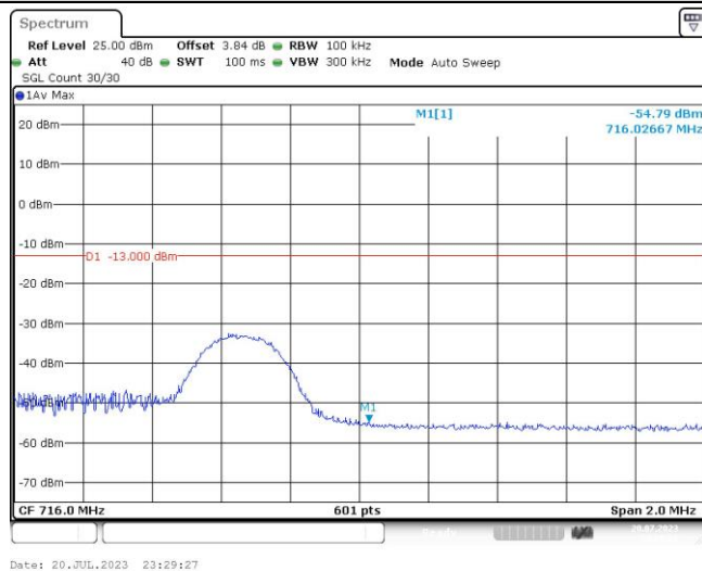
Band17-5MHz-16QAM-23825-1RB#24
