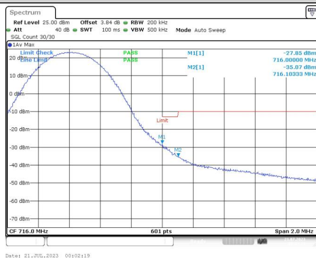
Band17-10MHz-QPSK-23800-50RB#0
