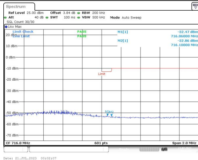
Band17-10MHz-16QAM-23800-1RB#49
