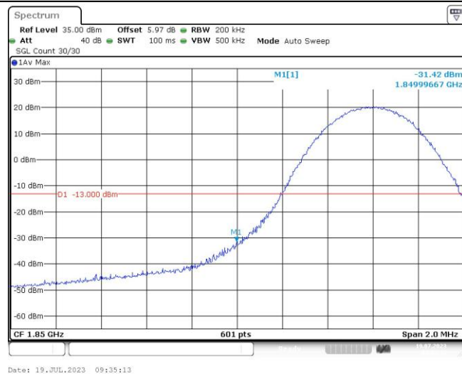
Band2-10MHz-16QAM-18650-1RB#49
