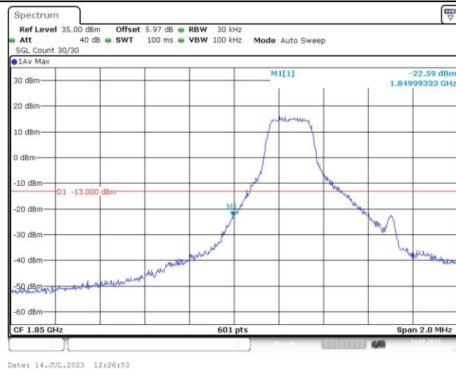
Band2-1.4MHz-16QAM-18607-1RB#5
