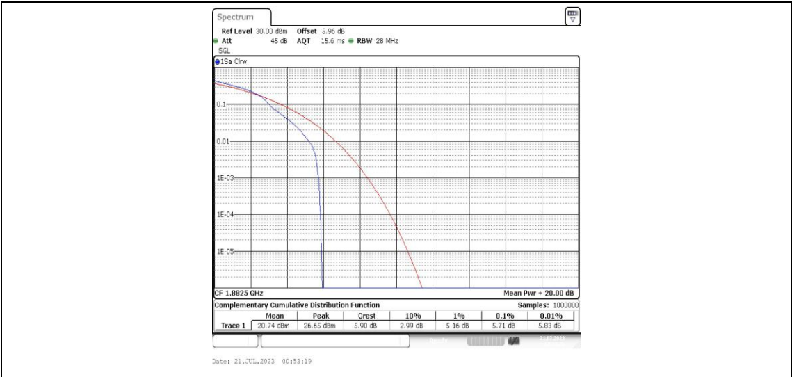
Band25-1.4MHz-16QAM-26365-1RB#0-PASS
