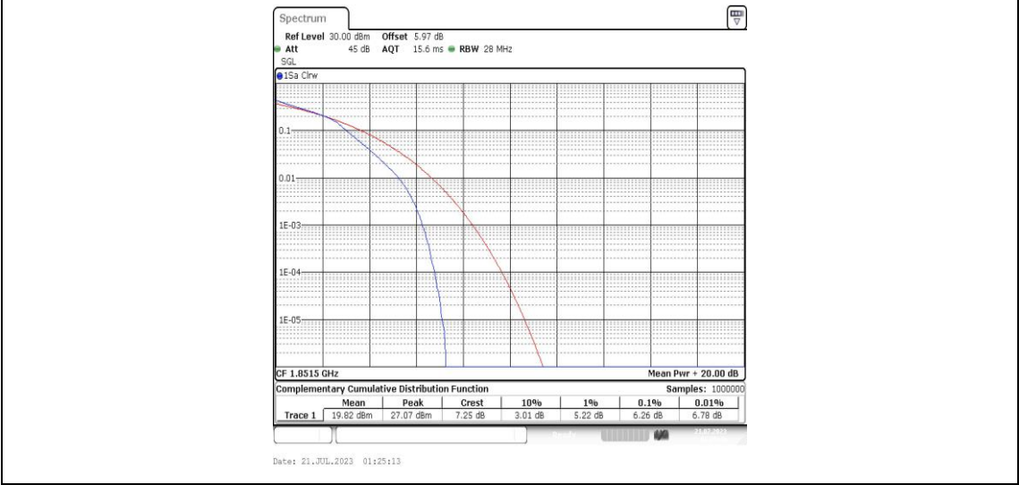
Band25-3MHz-16QAM-26055-15RB#0-PASS
