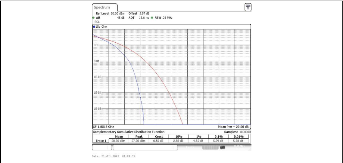
Band25-3MHz-QPSK-26055-15RB#0-PASS
