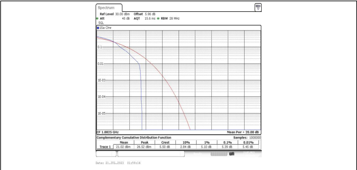
Band25-5MHz-16QAM-26365-1RB#0-PASS
