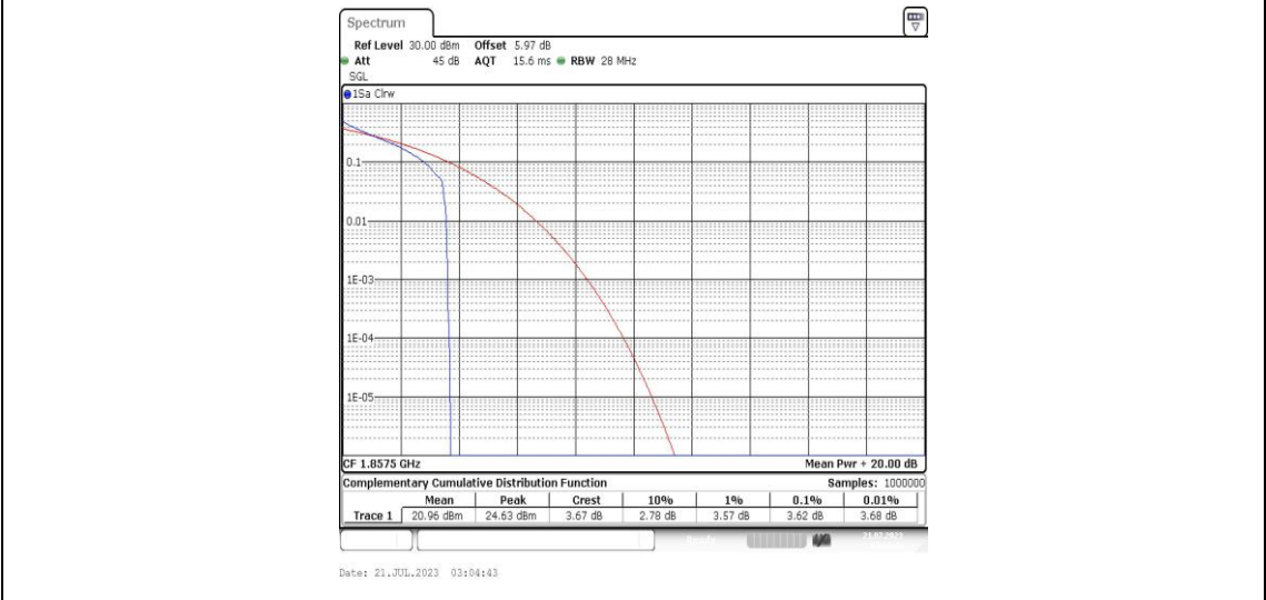
Band25-15MHz-QPSK-26115-1RB#0-PASS
