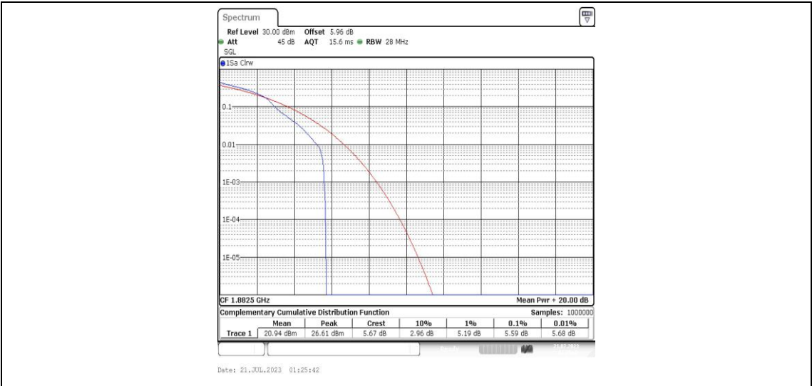
Band25-3MHz-16QAM-26365-1RB#0-PASS
