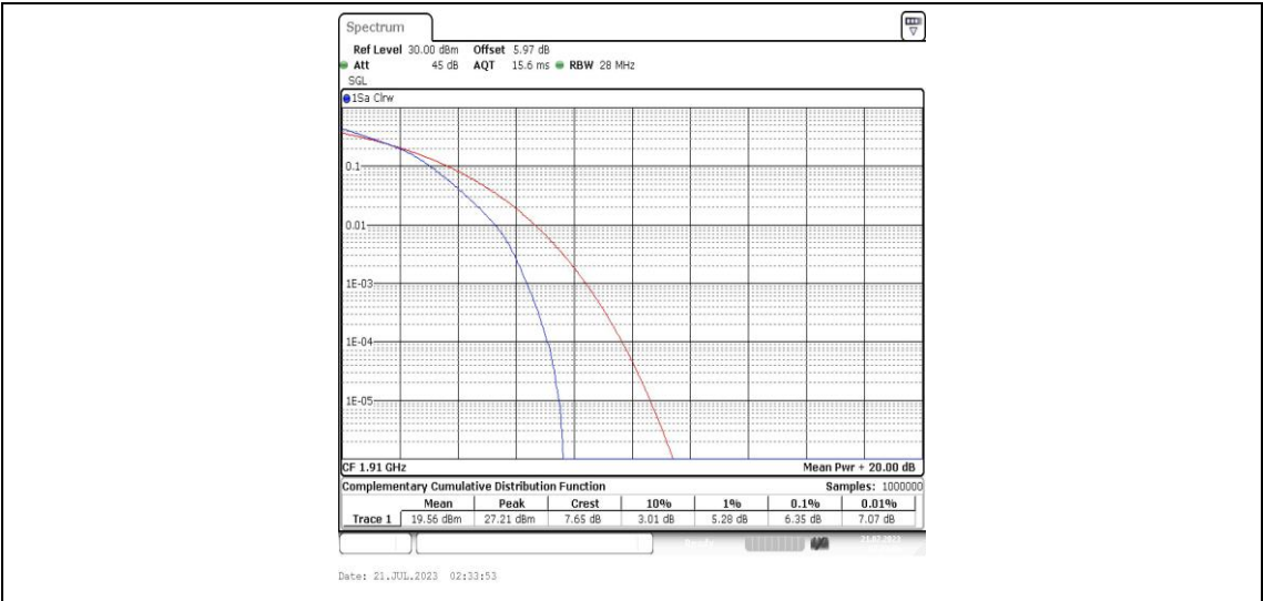
Band25-10MHz-16QAM-26640-50RB#0-PASS
