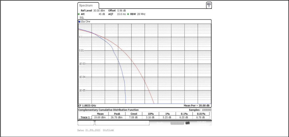
Band25-1.4MHz-16QAM-26365-6RB#0-PASS
