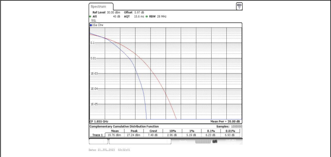
Band25-10MHz-16QAM-26090-50RB#0-PASS
