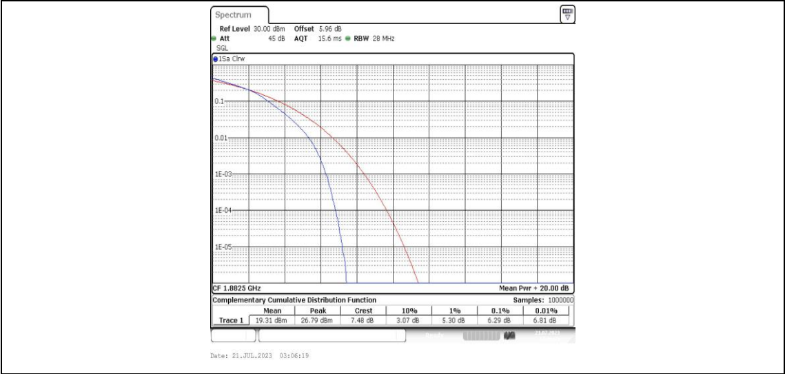
Band25-15MHz-16QAM-26365-75RB#0-PASS
