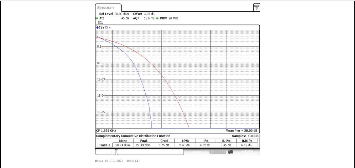
Band25-10MHz-QPSK-26090-50RB#0-PASS
