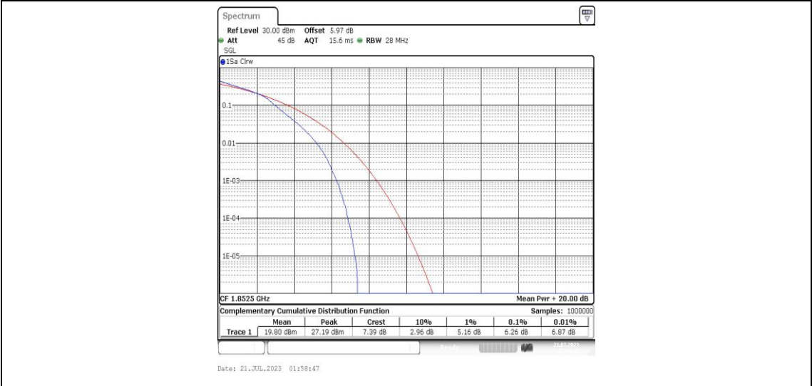
Band25-5MHz-16QAM-26065-25RB#0-PASS
