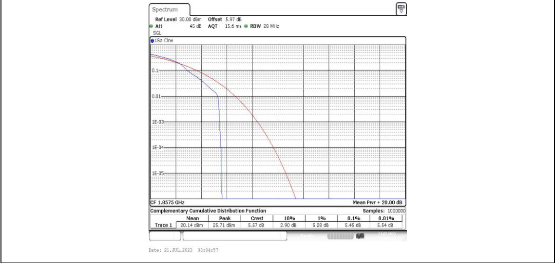
Band25-15MHz-16QAM-26115-1RB#0-PASS
