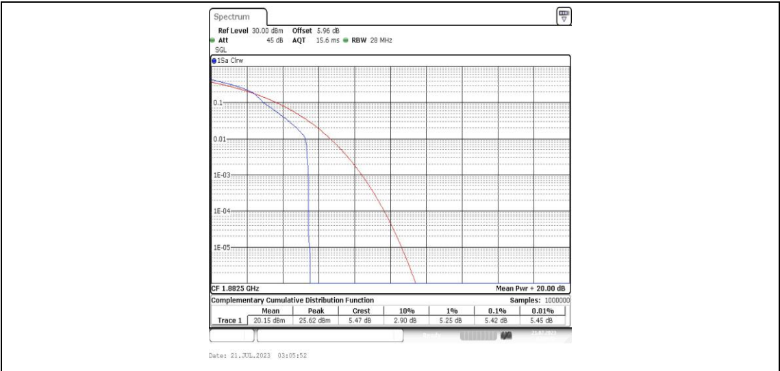
Band25-15MHz-16QAM-26365-1RB#0-PASS
