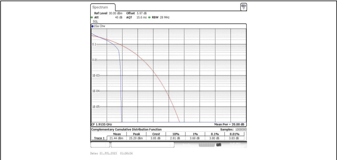
Band25-3MHz-QPSK-26675-1RB#0-PASS
