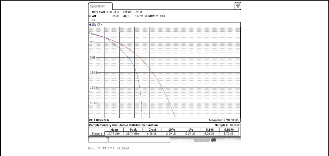
Band25-3MHz-16QAM-26365-15RB#0-PASS
