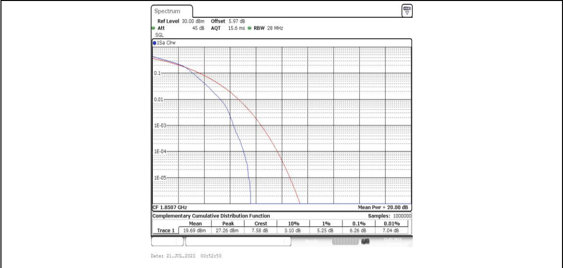
Band25-1.4MHz-16QAM-26047-6RB#0-PASS
