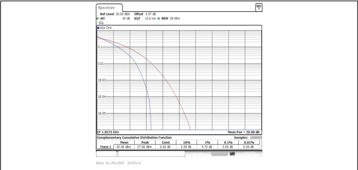
Band25-15MHz-QPSK-26115-75RB#0-PASS
