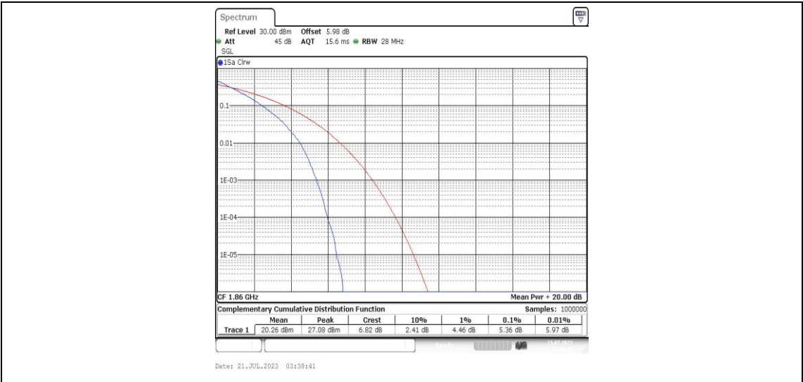
Band25-20MHz-QPSK-26140-100RB#0-PASS
