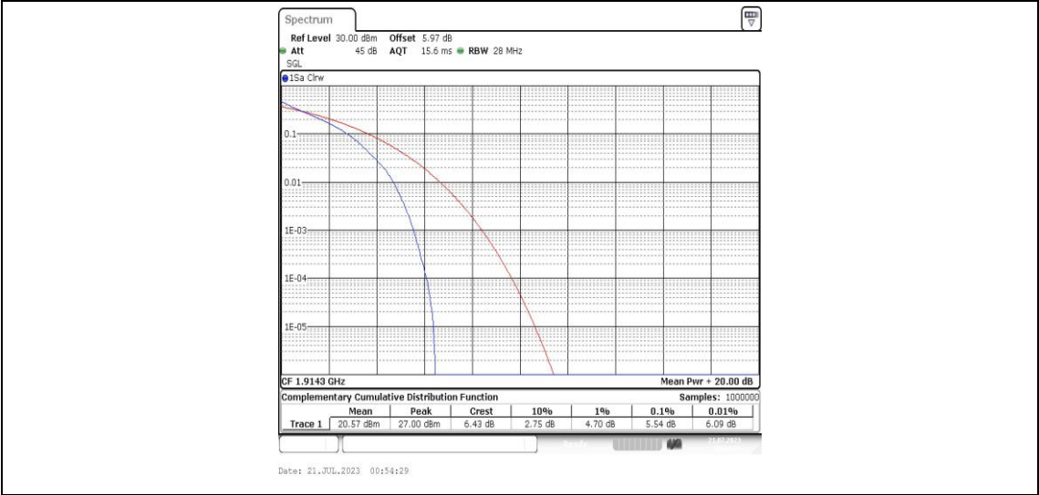
Band25-1.4MHz-QPSK-26683-6RB#0-PASS
