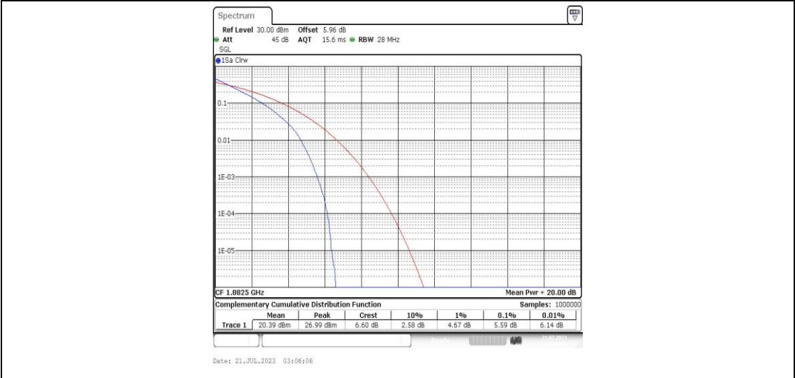
Band25-15MHz-QPSK-26365-75RB#0-PASS
