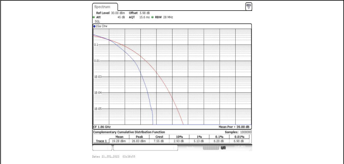
Band25-20MHz-16QAM-26140-100RB#0-PASS
