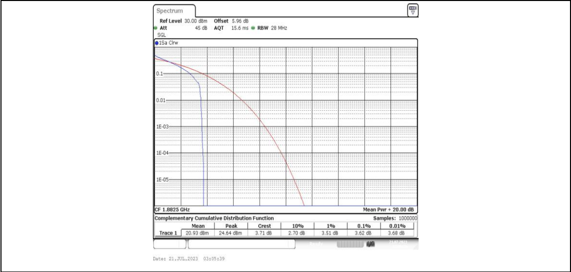
Band25-15MHz-QPSK-26365-1RB#0-PASS
