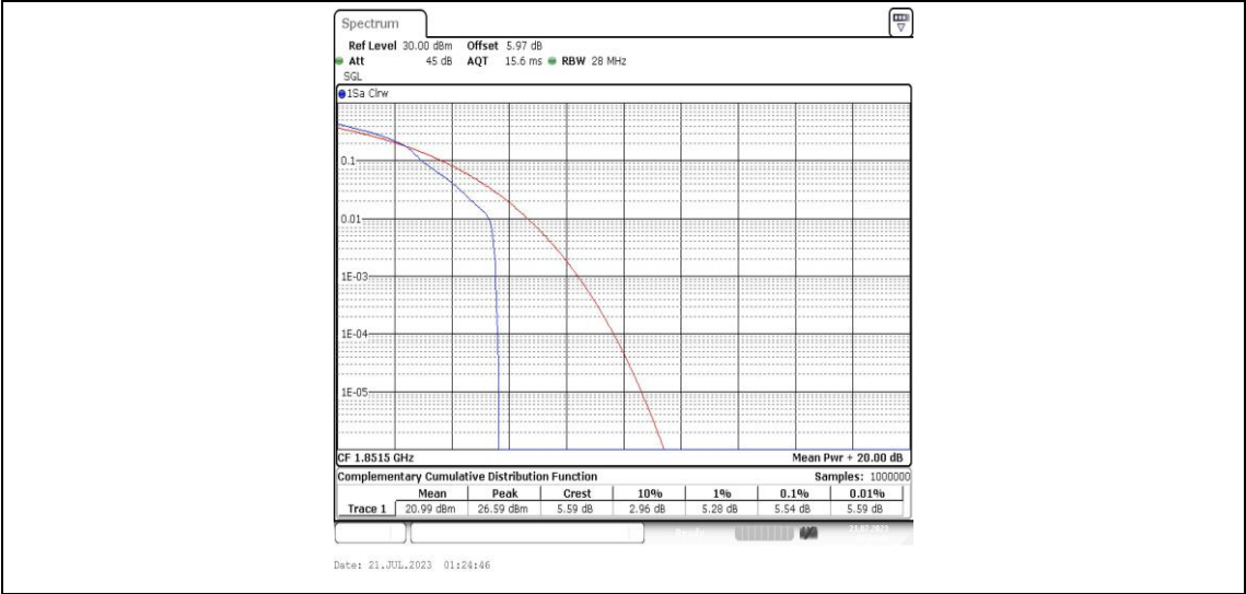
Band25-3MHz-16QAM-26055-1RB#0-PASS
