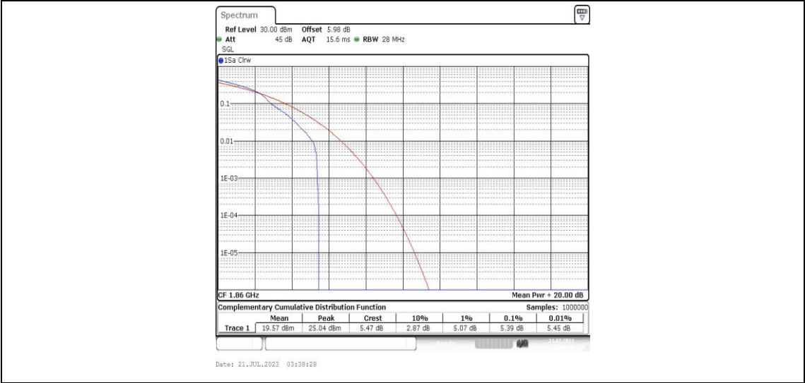
Band25-20MHz-16QAM-26140-1RB#0-PASS
