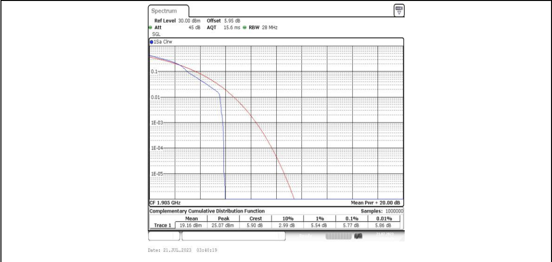
Band25-20MHz-16QAM-26590-1RB#0-PASS
