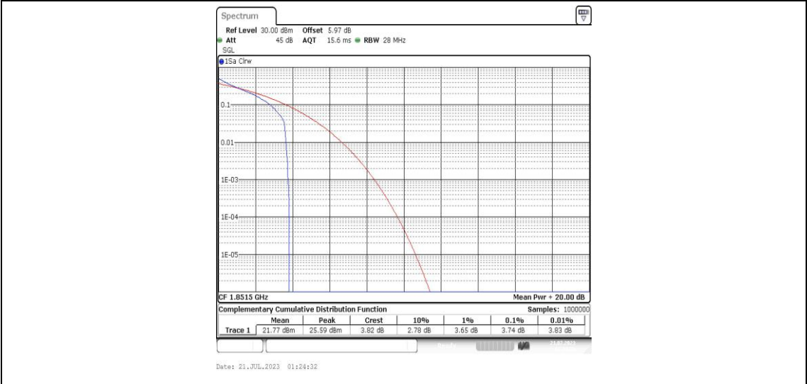
Band25-3MHz-QPSK-26055-1RB#0-PASS
