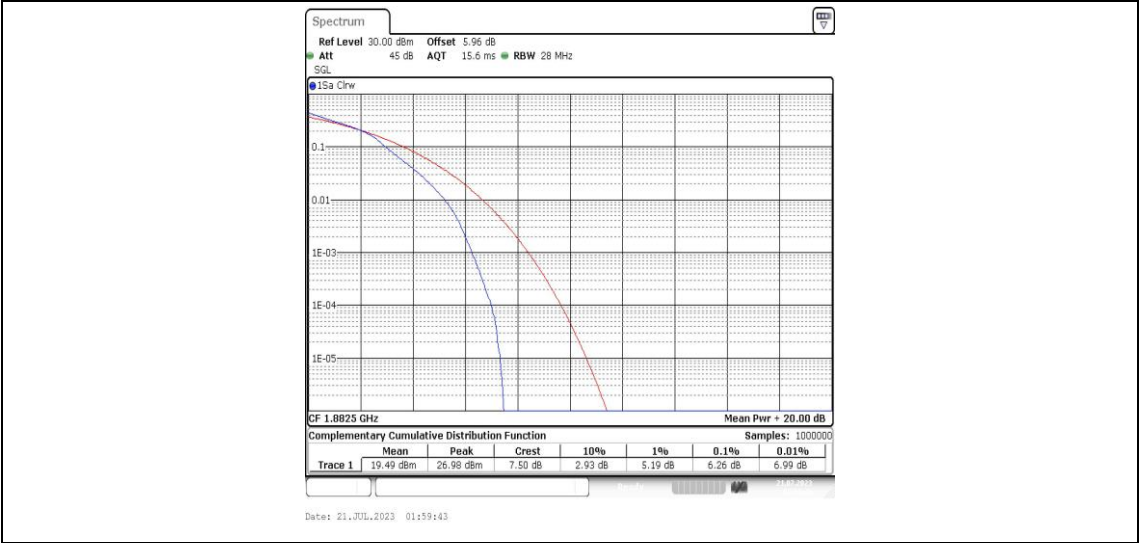
Band25-5MHz-16QAM-26365-25RB#0-PASS
