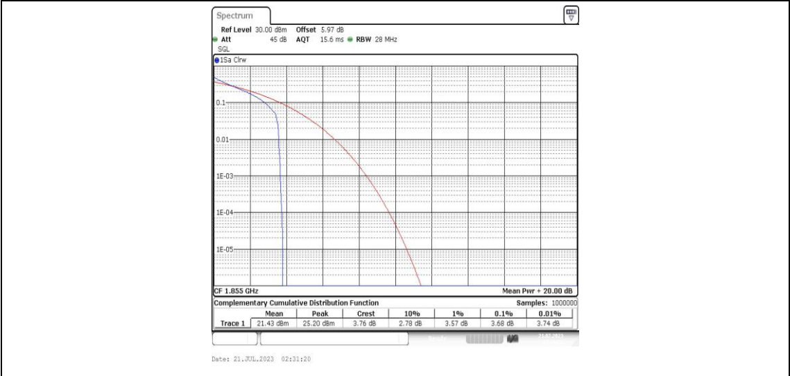
Band25-10MHz-QPSK-26090-1RB#0-PASS
