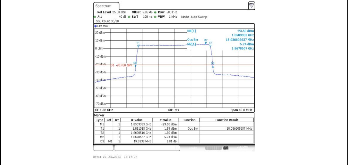
Band25-20MHz-16QAM-26140-100RB#0-PASS
