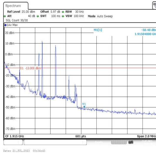
Band25-1.4MHz-QPSK-26683-1RB#0-PASS
