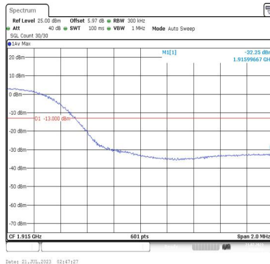
Band25-15MHz-QPSK-26615-75RB#0-PASS
