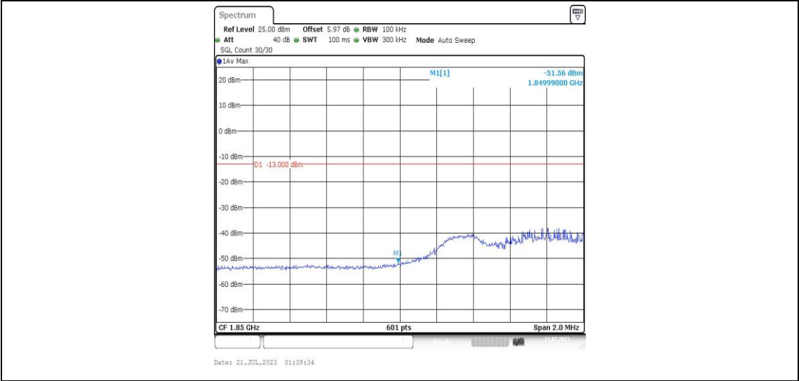
Band25-5MHz-QPSK-26065-1RB#24-PASS
