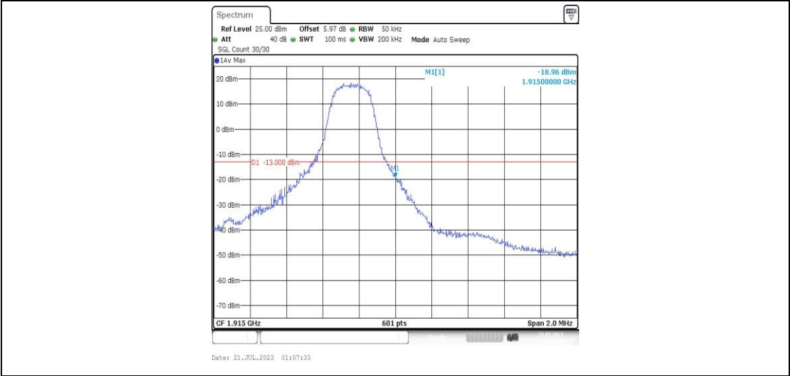
Band25-3MHz-QPSK-26675-1RB#14-PASS
