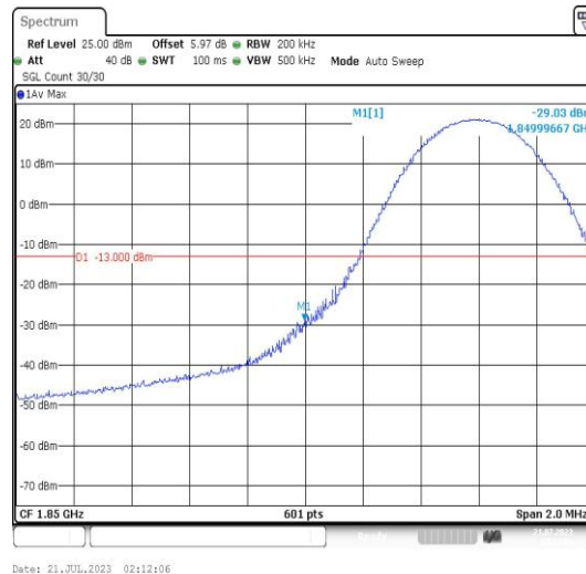
Band25-10MHz-QPSK-26090-1RB#0-PASS
