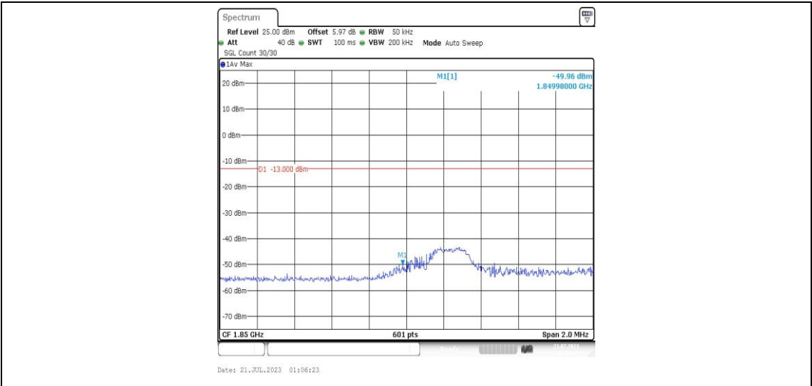
Band25-3MHz-16QAM-26055-1RB#14-PASS
