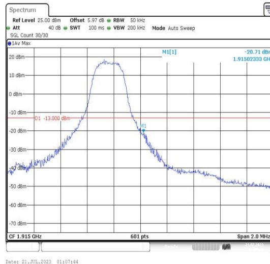
Band25-3MHz-16QAM-26675-1RB#14-PASS
