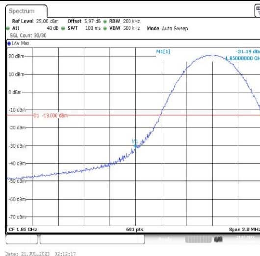
Band25-10MHz-16QAM-26090-1RB#0-PASS
