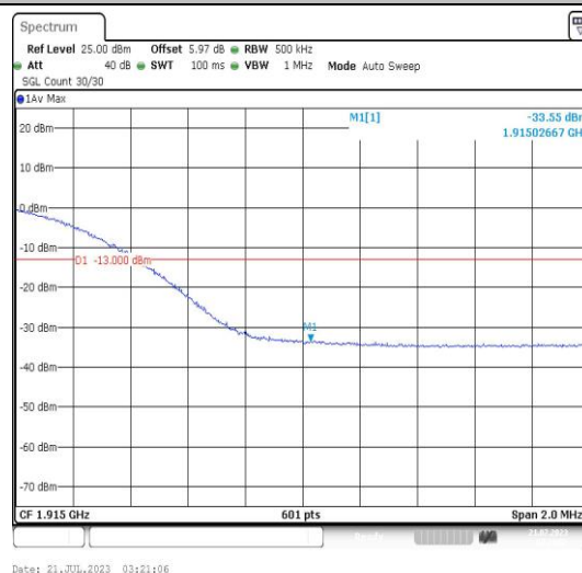
Band25-20MHz-16QAM-26590-100RB#0-PASS
