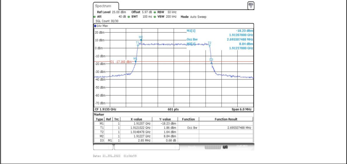
Band25-3MHz-QPSK-26675-15RB#0-PASS
