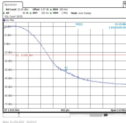
Band25-15MHz-16QAM-26615-1RB#74-PASS
