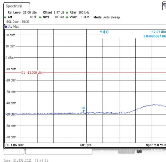
Band25-15MHz-16QAM-26115-1RB#74-PASS
