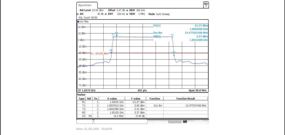
Band25-15MHz-QPSK-26115-75RB#0-PASS
