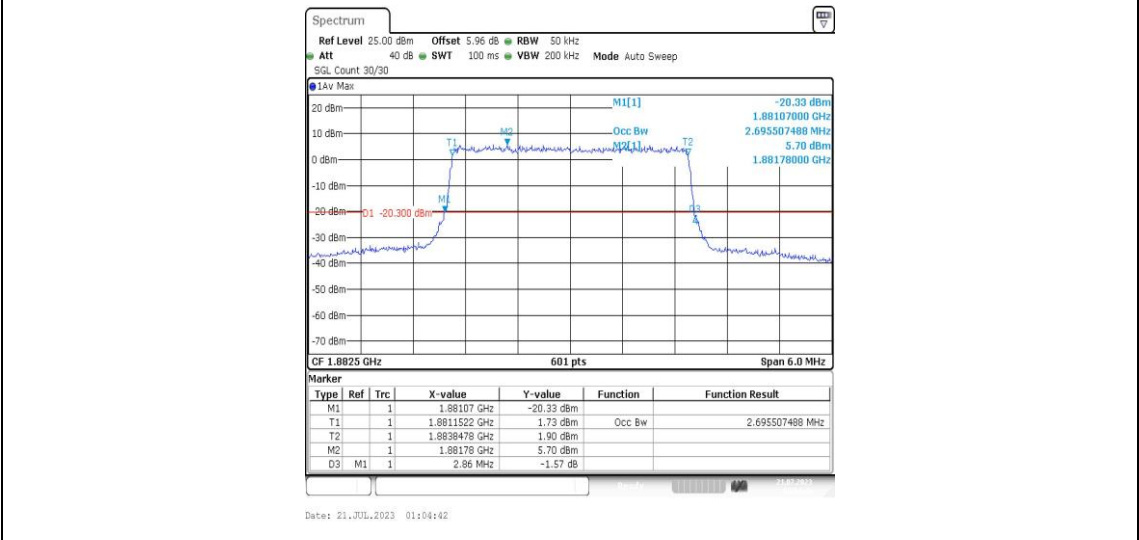
Band25-3MHz-16QAM-26365-15RB#0-PASS
