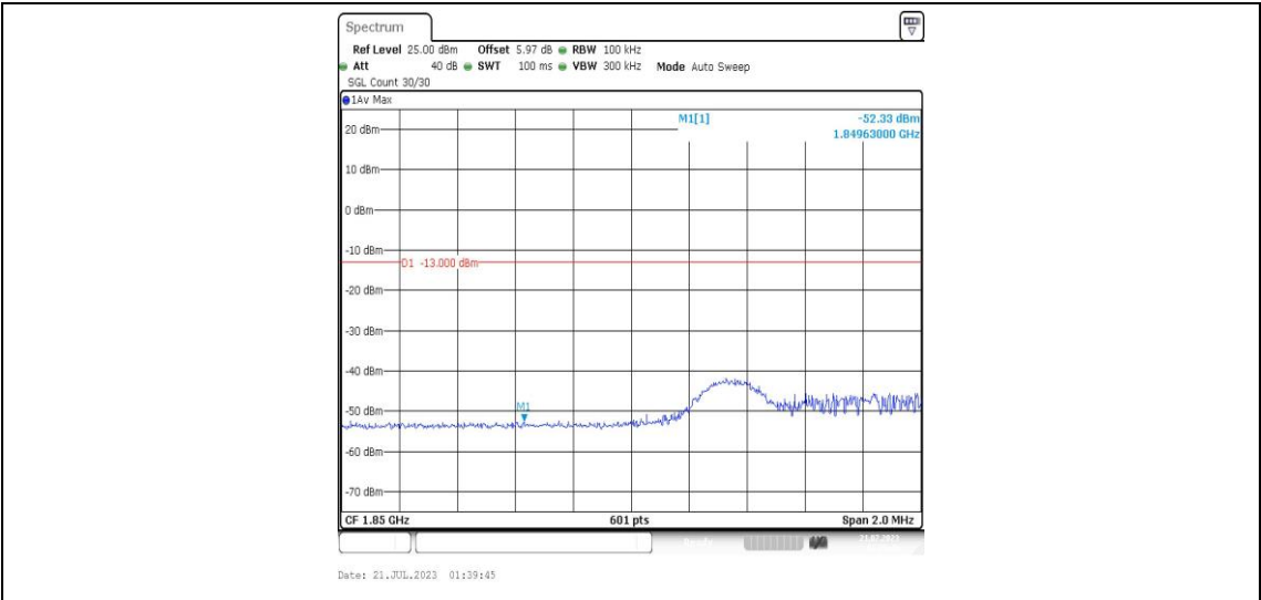
Band25-5MHz-16QAM-26065-1RB#24-PASS
