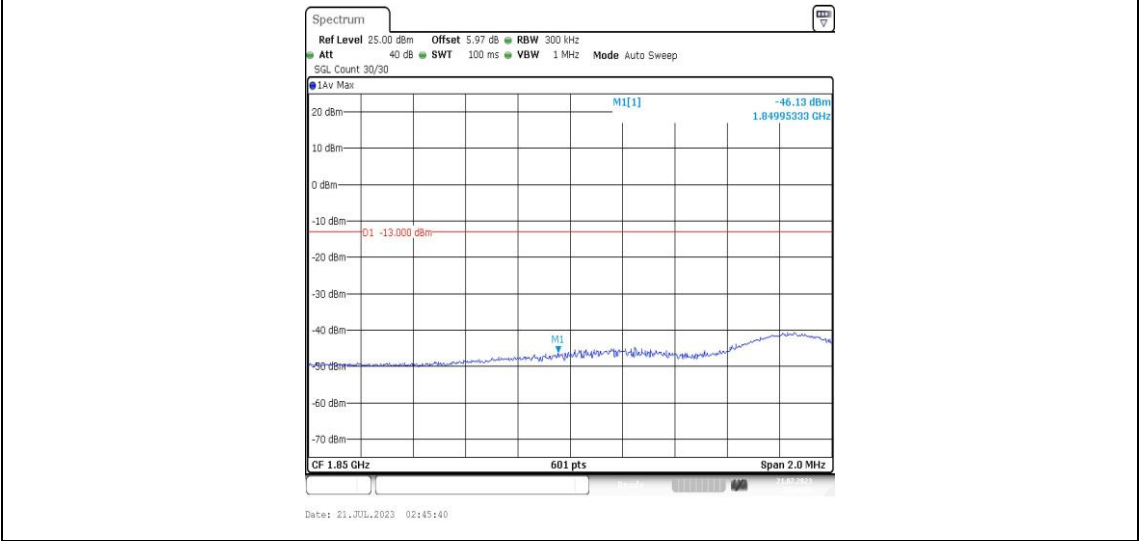
Band25-15MHz-QPSK-26115-1RB#74-PASS
