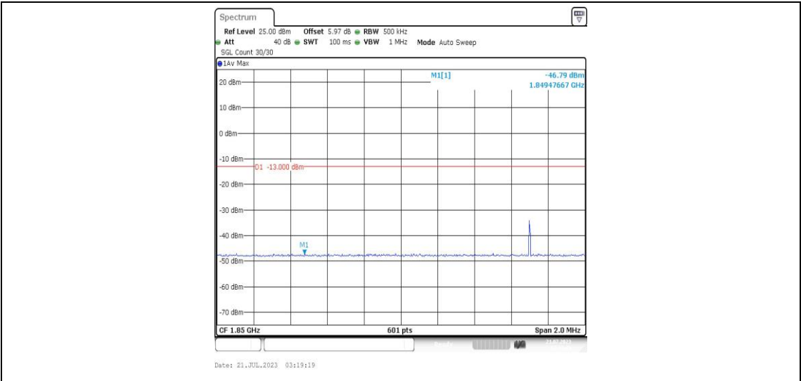
Band25-20MHz-16QAM-26140-1RB#99-PASS
