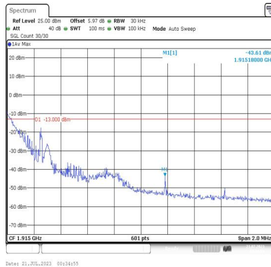
Band25-1.4MHz-16QAM-26683-1RB#0-PASS
