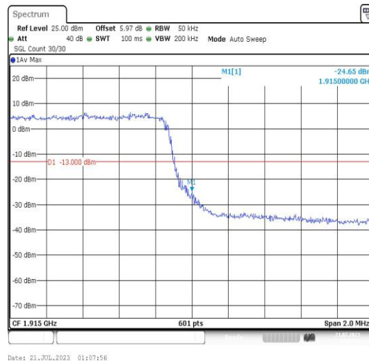
Band25-3MHz-QPSK-26675-15RB#0-PASS
