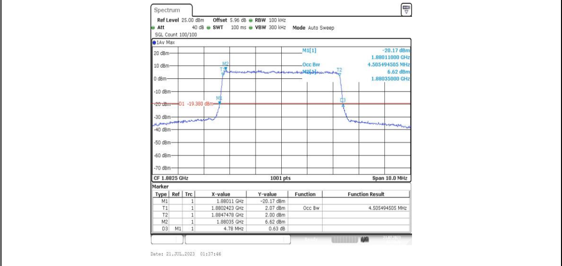
Band25-5MHz-16QAM-26365-25RB#0-PASS
