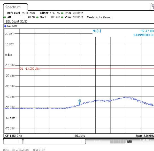
Band25-10MHz-QPSK-26090-1RB#49-PASS
