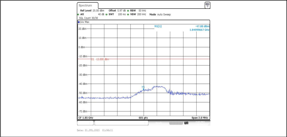
Band25-3MHz-QPSK-26055-1RB#14-PASS
