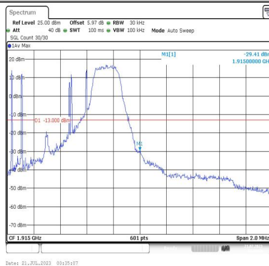
Band25-1.4MHz-QPSK-26683-1RB#5-PASS
