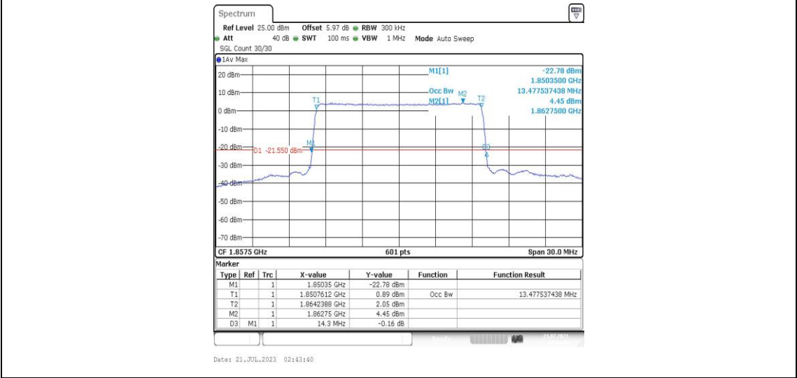
Band25-15MHz-16QAM-26115-75RB#0-PASS
