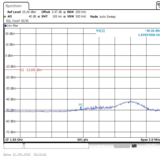
Band25-10MHz-16QAM-26090-1RB#49-PASS
