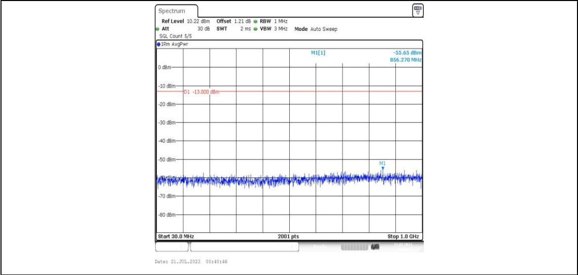
Band25-1.4MHz-16QAM-26683-1RB#0-Range3:30~1000MHz-PASS
