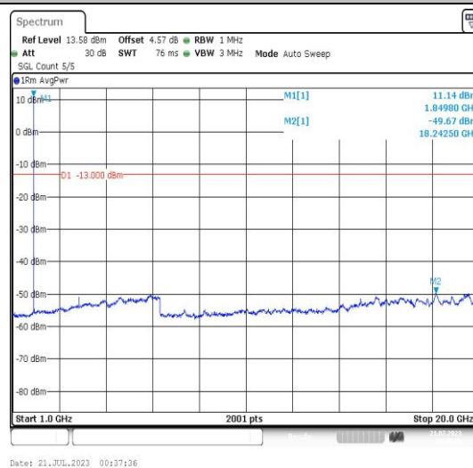
Band25-1.4MHz-16QAM-26047-1RB#0-Range4:1000~20000MHz-PASS
