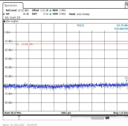
Band25-1.4MHz-QPSK-26683-1RB#0-Range3:30~1000MHz-PASS
