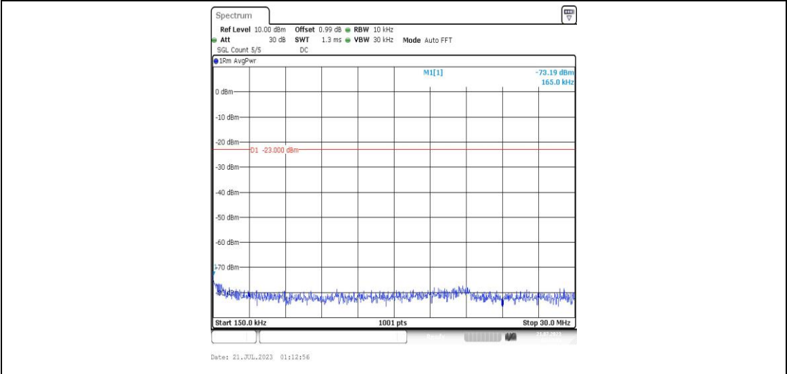
Band25-3MHz-16QAM-26675-1RB#0-Range2:0.15~30MHz-PASS
