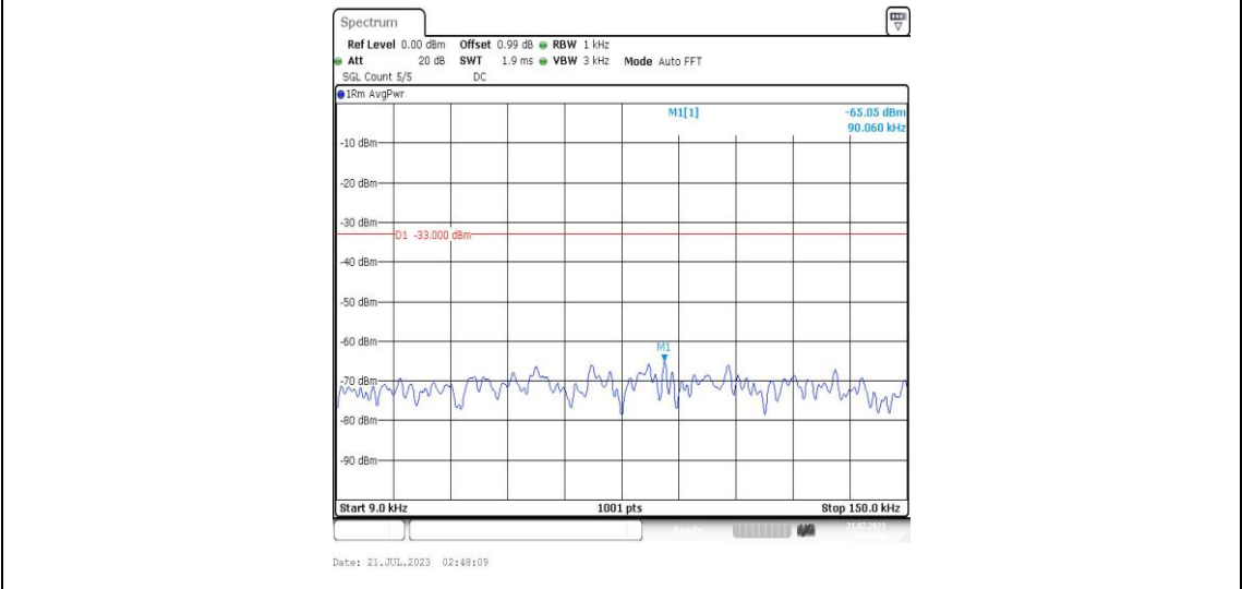
Band25-15MHz-QPSK-26115-1RB#0-Range1:0.009~0.15MHz-PASS
