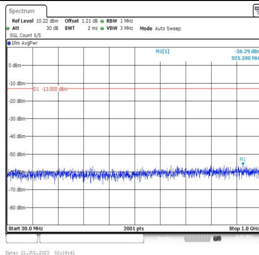
Band25-10MHz-QPSK-26640-1RB#0-Range3:30~1000MHz-PASS
