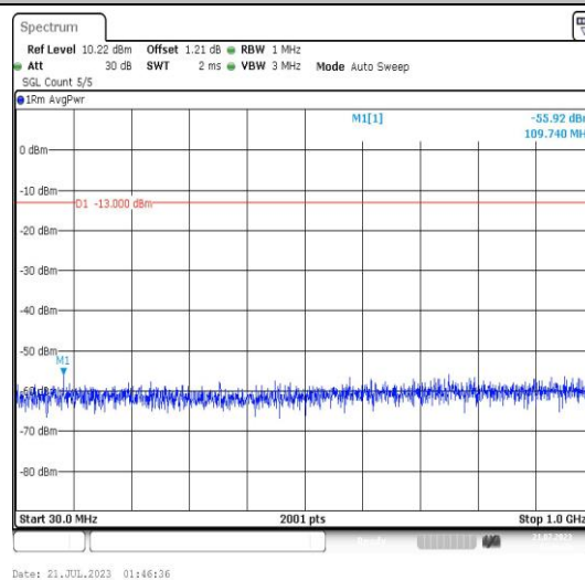
Band25-5MHz-16QAM-26665-1RB#0-Range3:30~1000MHz-PASS
