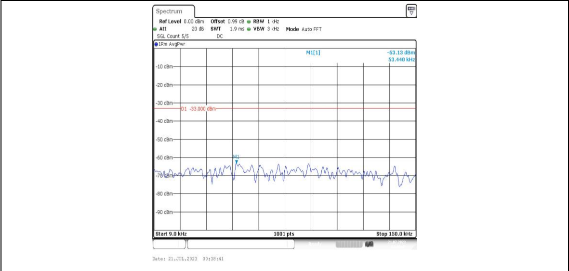
Band25-1.4MHz-16QAM-26365-1RB#0-Range1:0.009~0.15MHz-PASS
