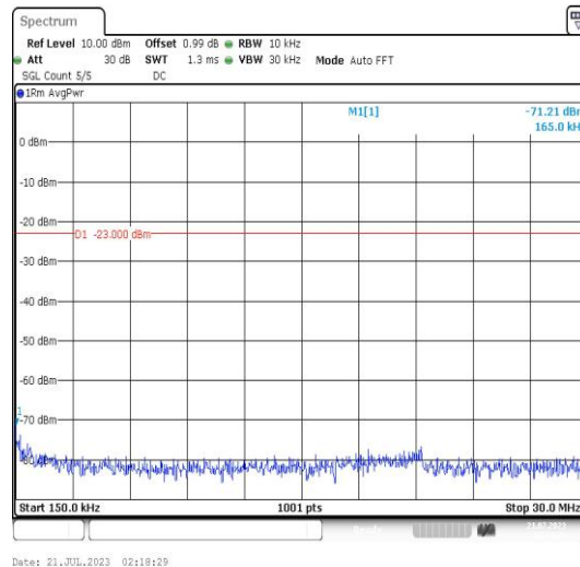
Band25-10MHz-QPSK-26640-1RB#0-Range2:0.15~30MHz-PASS
