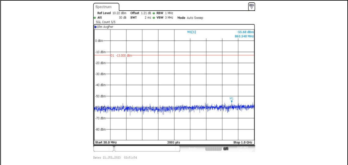
Band25-15MHz-QPSK-26615-1RB#0-Range3:30~1000MHz-PASS
