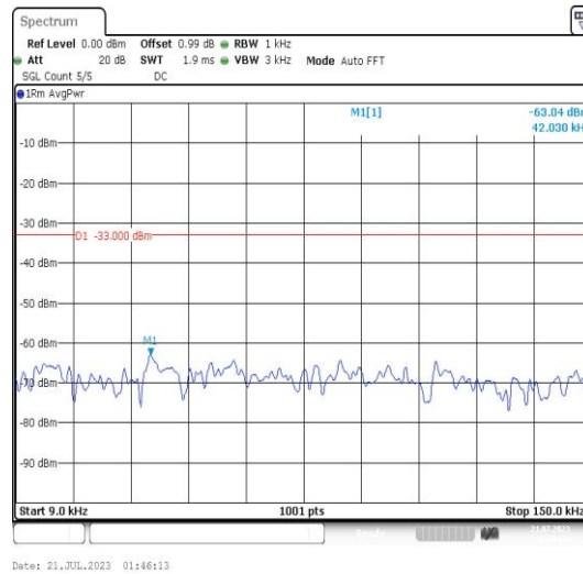
Band25-5MHz-16QAM-26665-1RB#0-Range1:0.009~0.15MHz-PASS
