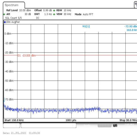
Band25-3MHz-16QAM-26055-1RB#0-Range2:0.15~30MHz-PASS
