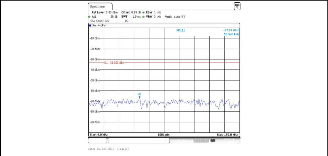
Band25-5MHz-QPSK-26065-1RB#0-Range1:0.009~0.15MHz-PASS
