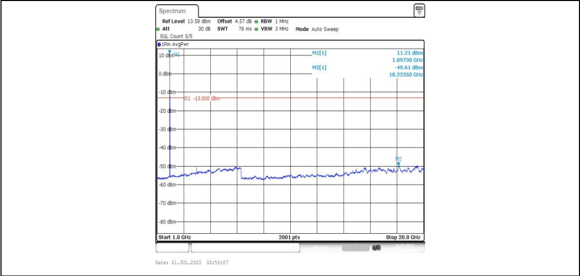
Band25-15MHz-QPSK-26615-1RB#0-Range4:1000~20000MHz-PASS
