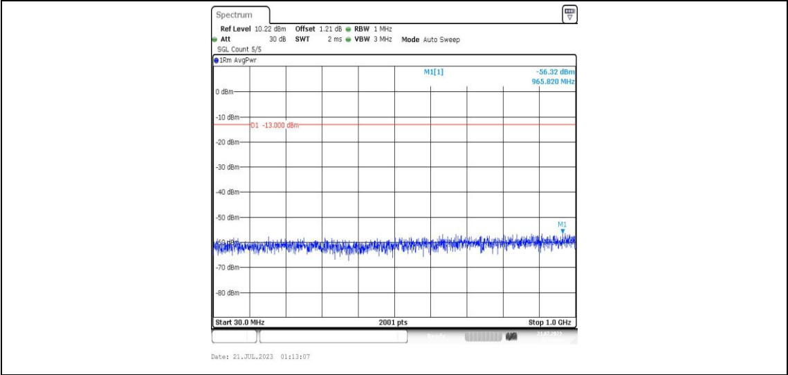
Band25-3MHz-16QAM-26675-1RB#0-Range3:30~1000MHz-PASS
