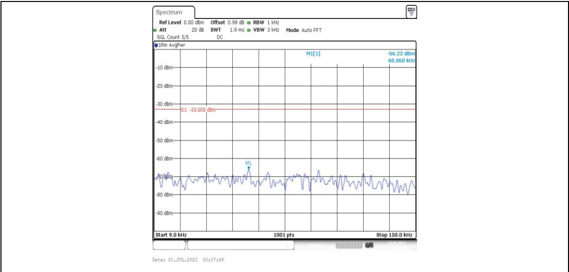
Band25-1.4MHz-QPSK-26365-1RB#0-Range1:0.009~0.15MHz-PASS
