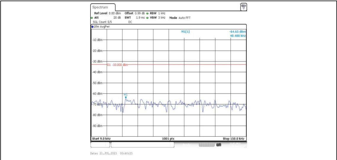
Band25-1.4MHz-16QAM-26683-1RB#0-Range1:0.009~0.15MHz-PASS
