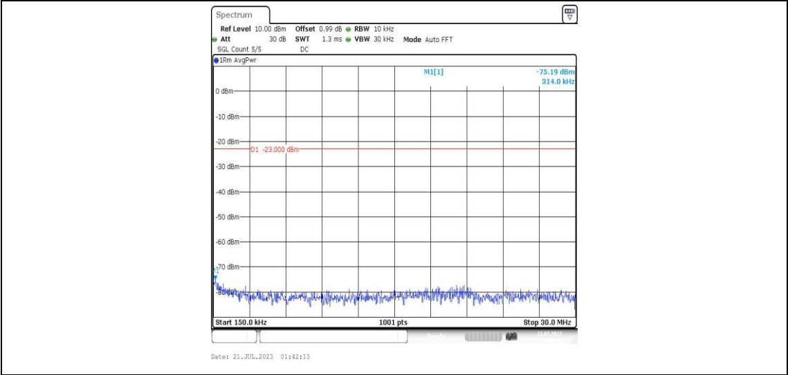
Band25-5MHz-QPSK-26065-1RB#0-Range2:0.15~30MHz-PASS
