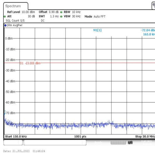
Band25-5MHz-16QAM-26665-1RB#0-Range2:0.15~30MHz-PASS
