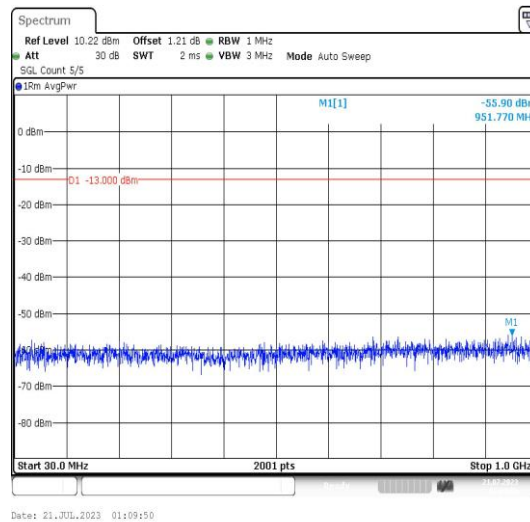
Band25-3MHz-16QAM-26055-1RB#0-Range3:30~1000MHz-PASS
