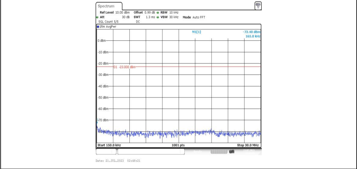
Band25-15MHz-QPSK-26115-1RB#0-Range2:0.15~30MHz-PASS
