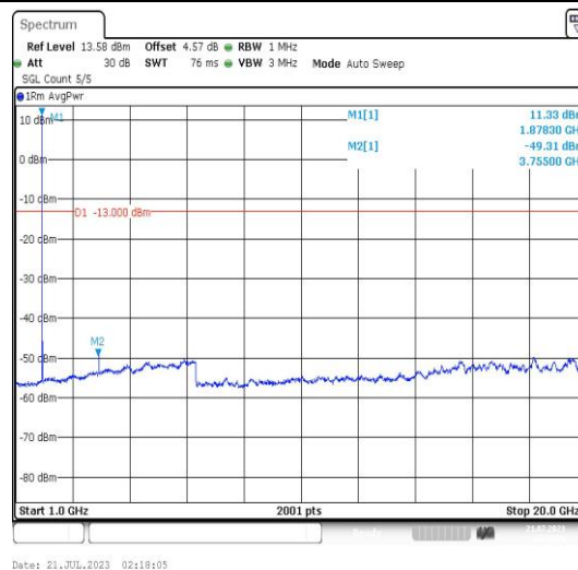
Band25-10MHz-16QAM-26365-1RB#0-Range4:1000~20000MHz-PASS
