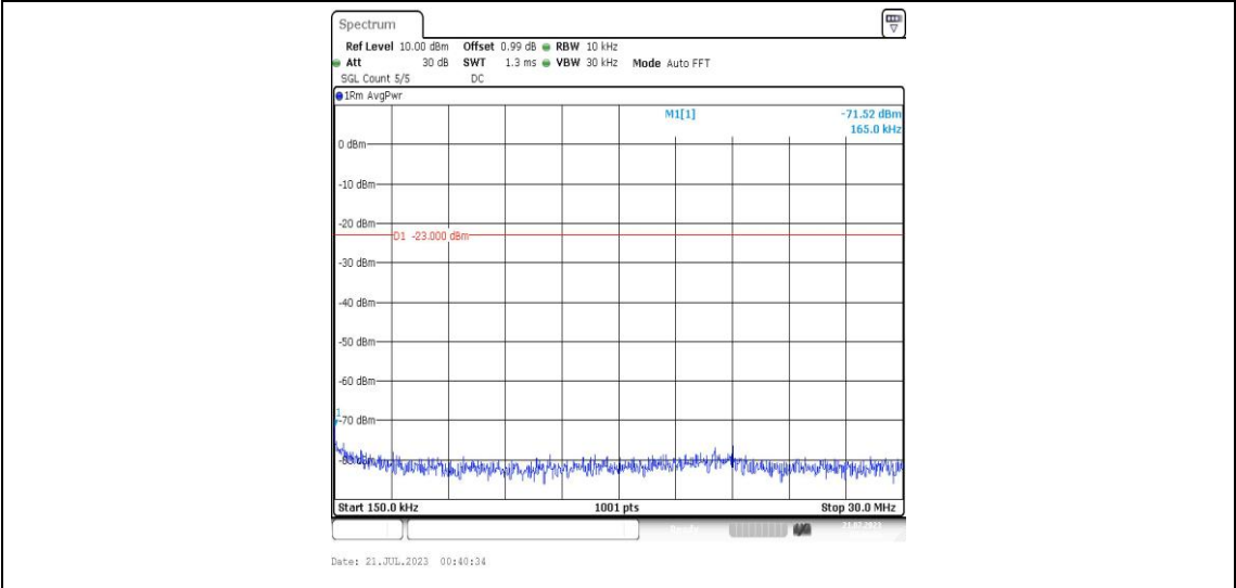
Band25-1.4MHz-16QAM-26683-1RB#0-Range2:0.15~30MHz-PASS
