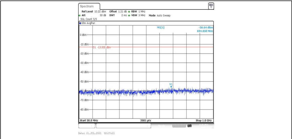
Band25-10MHz-QPSK-26090-1RB#0-Range3:30~1000MHz-PASS
