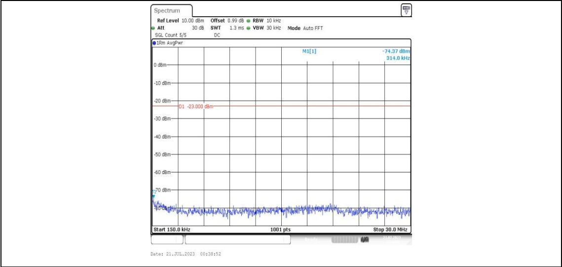
Band25-1.4MHz-16QAM-26365-1RB#0-Range2:0.15~30MHz-PASS
