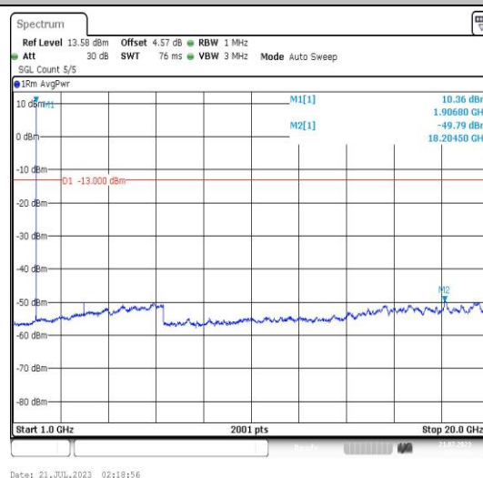
Band25-10MHz-QPSK-26640-1RB#0-Range4:1000~20000MHz-PASS
