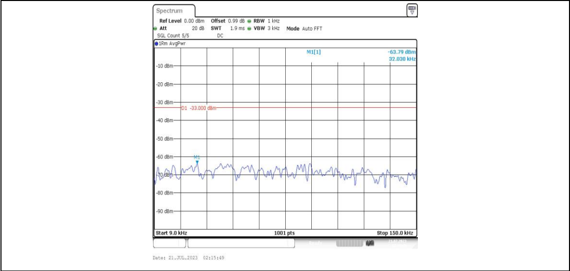
Band25-10MHz-16QAM-26090-1RB#0-Range1:0.009~0.15MHz-PASS
