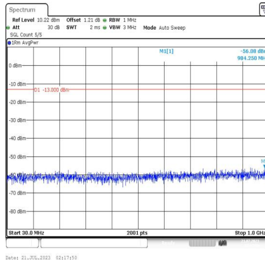
Band25-10MHz-16QAM-26365-1RB#0-Range3:30~1000MHz-PASS
