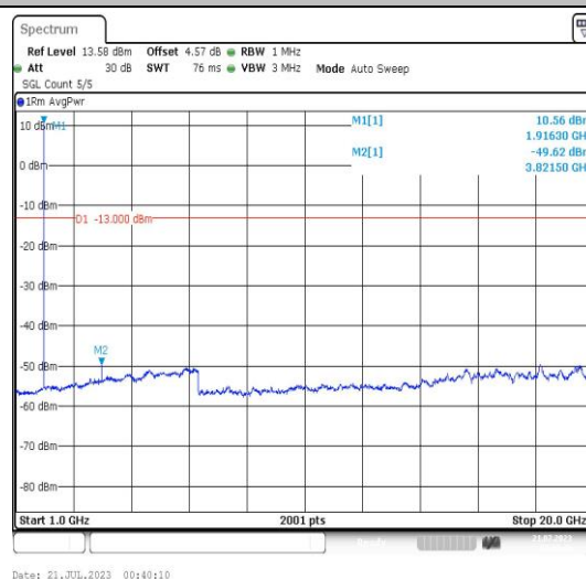
Band25-1.4MHz-QPSK-26683-1RB#0-Range4:1000~20000MHz-PASS
