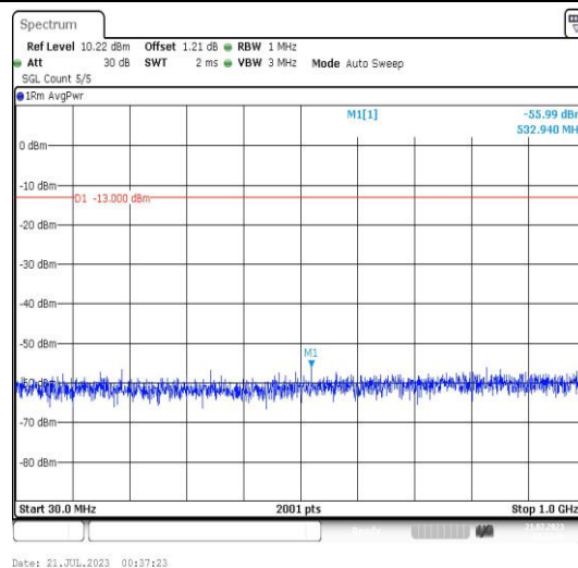
Band25-1.4MHz-16QAM-26047-1RB#0-Range3:30~1000MHz-PASS
