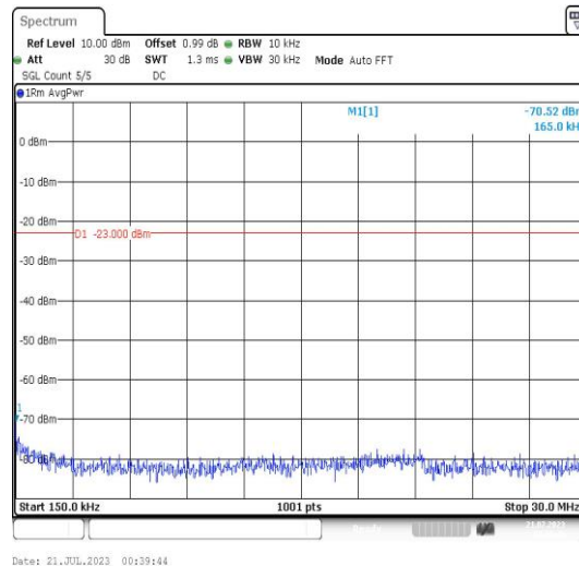
Band25-1.4MHz-QPSK-26683-1RB#0-Range2:0.15~30MHz-PASS
