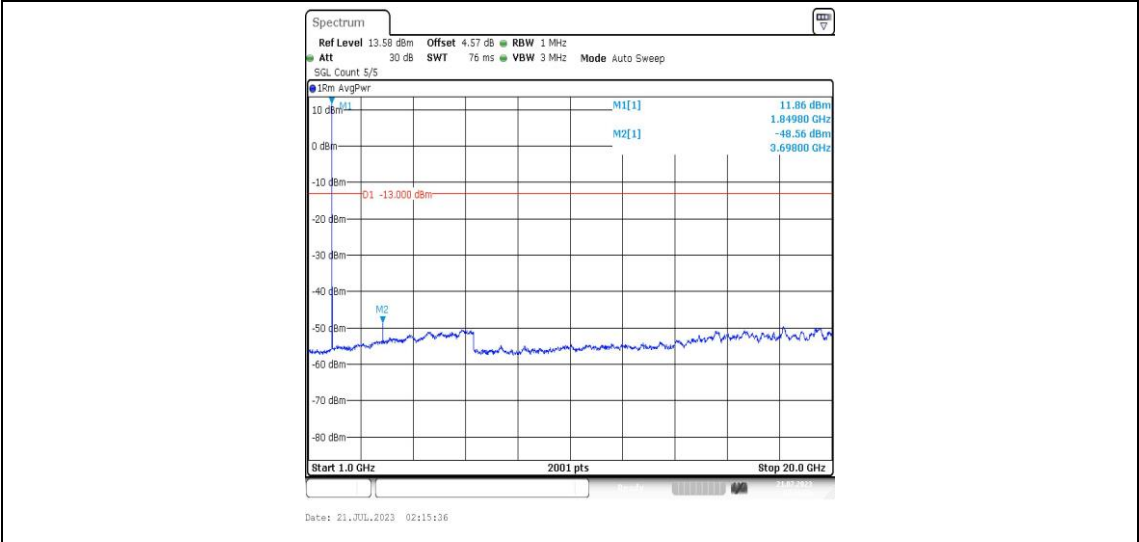
Band25-10MHz-QPSK-26090-1RB#0-Range4:1000~20000MHz-PASS
