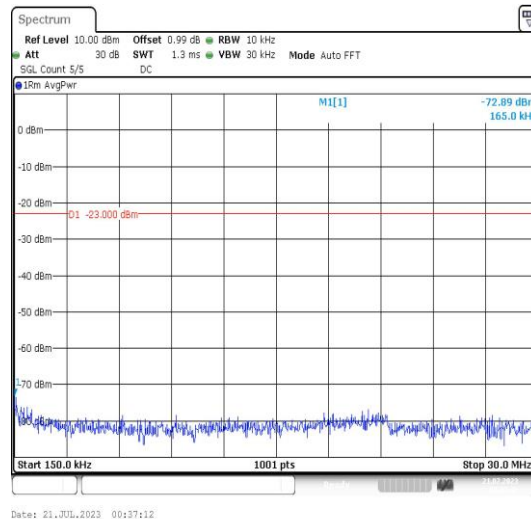
Band25-1.4MHz-16QAM-26047-1RB#0-Range2:0.15~30MHz-PASS
