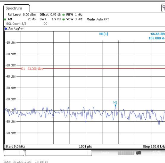
Band25-10MHz-QPSK-26640-1RB#0-Range1:0.009~0.15MHz-PASS
