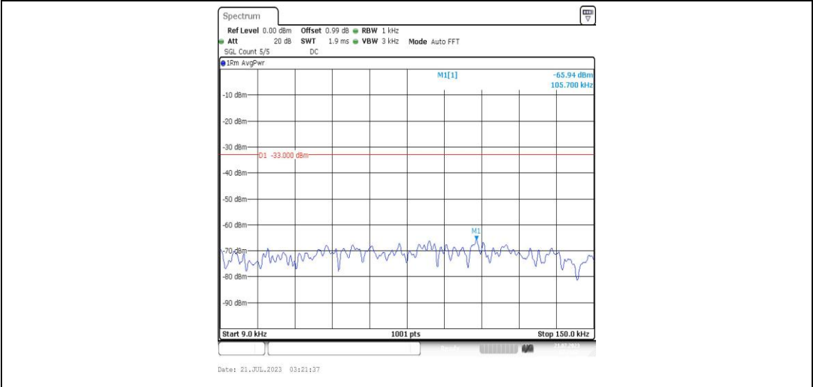
Band25-20MHz-QPSK-26140-1RB#0-Range1:0.009~0.15MHz-PASS
