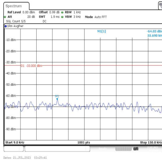
Band25-20MHz-16QAM-26590-1RB#0-Range1:0.009~0.15MHz-PASS
