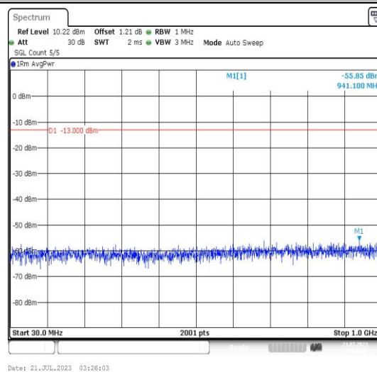
Band25-20MHz-16QAM-26590-1RB#0-Range3:30~1000MHz-PASS
