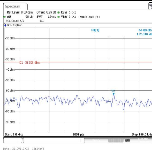
Band25-20MHz-16QAM-26365-1RB#0-Range1:0.009~0.15MHz-PASS
