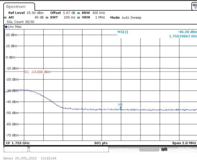
Band4-15MHz-QPSK-20325-1RB#74
