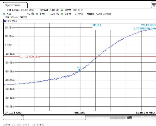
Band4-20MHz-16QAM-20050-1RB#99
