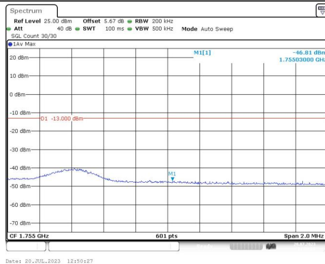
Band4-10MHz-16QAM-20350-1RB#49
