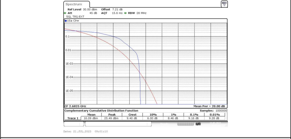
Band41-15MHz-16QAM-41515-75RB#0
