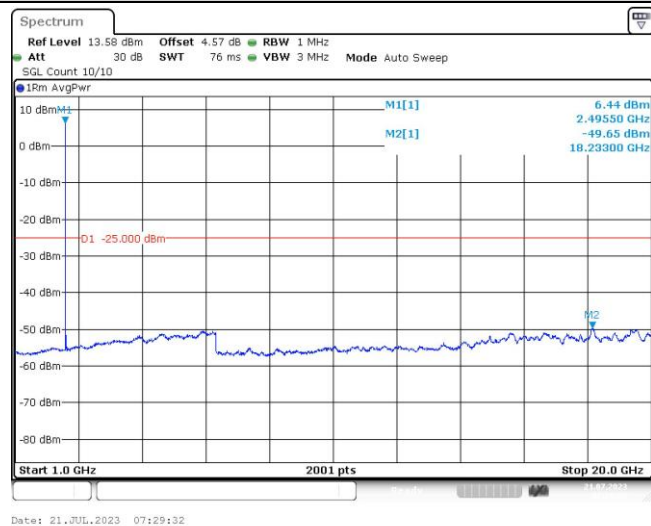
Band41-5MHz-16QAM-39675-1RB#0-Range5:20000~27000MHz
