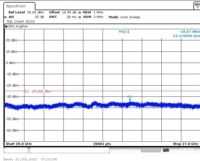
Band41-5MHz-16QAM-41565-1RB#0-Range1:0.009~0.15MHz
