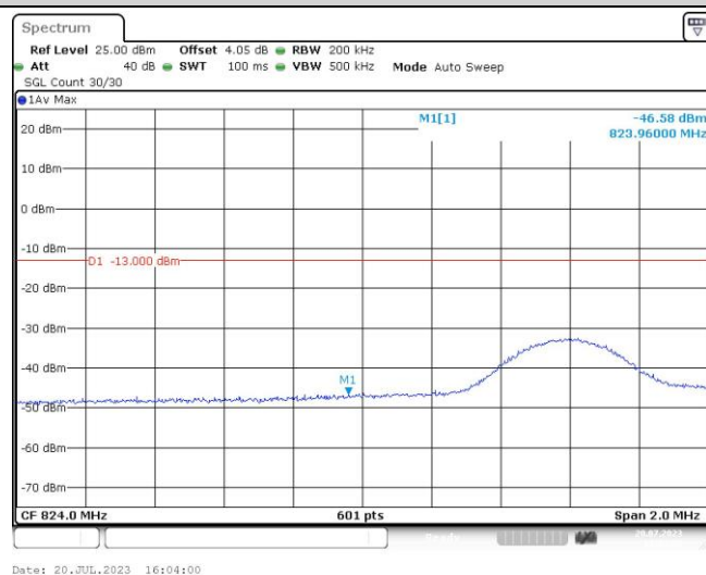
Band5-10MHz-16QAM-20450-50RB#0
