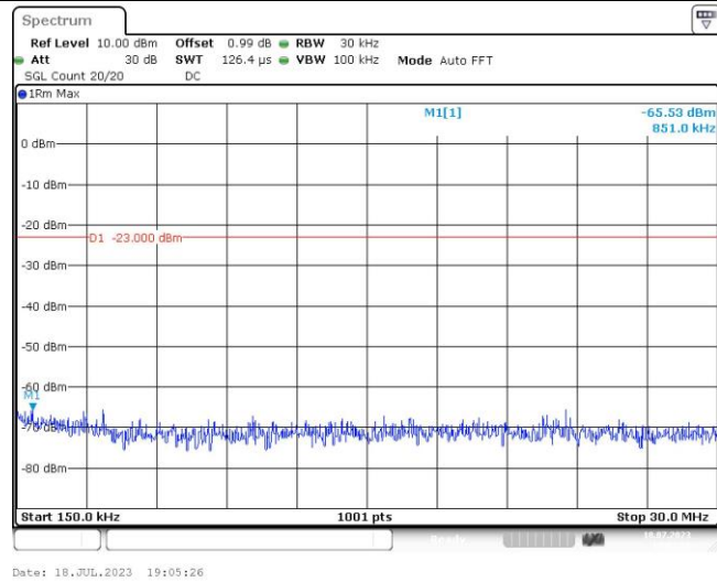
Band2-9400-2-0.15~30MHz
