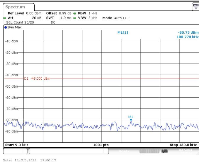
Band2-9538-2-0.009~0.15MHz
