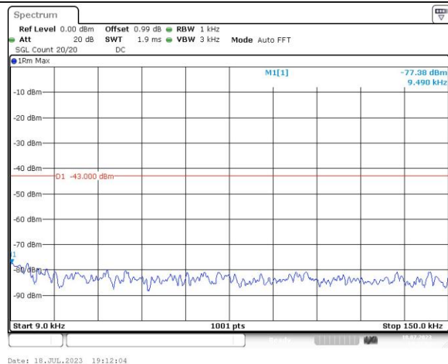
Band2-9400-4-0.009~0.15MHz
