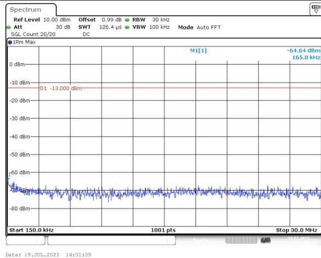
Band5-4183-2-0.15~30MHz
