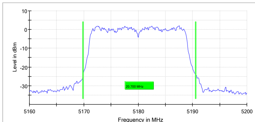
26 dB Bandwidth
