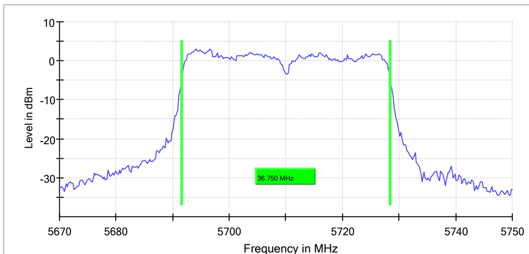
99 % Bandwidth
