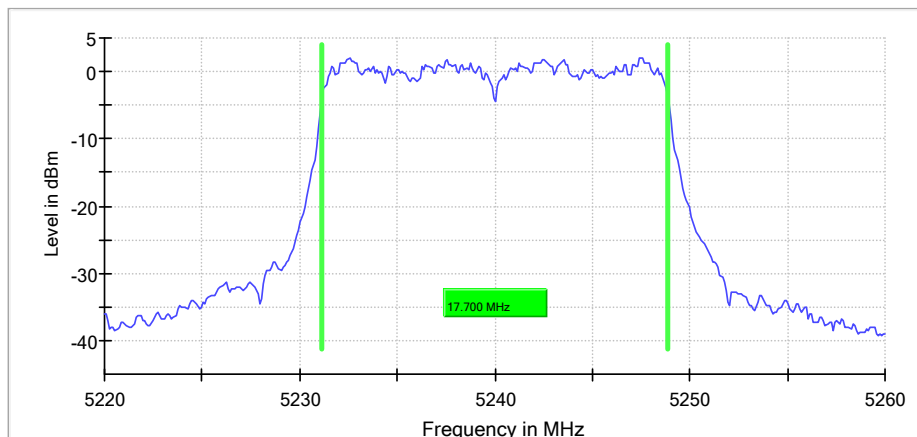
99 % Bandwidth
