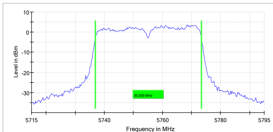
99 % Bandwidth
