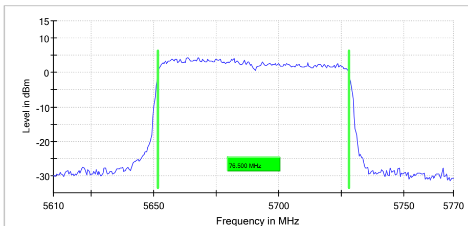
99 % Bandwidth
