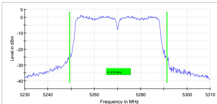
26 dB Bandwidth
