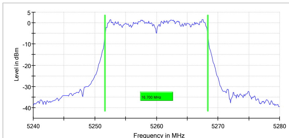
99 % Bandwidth
