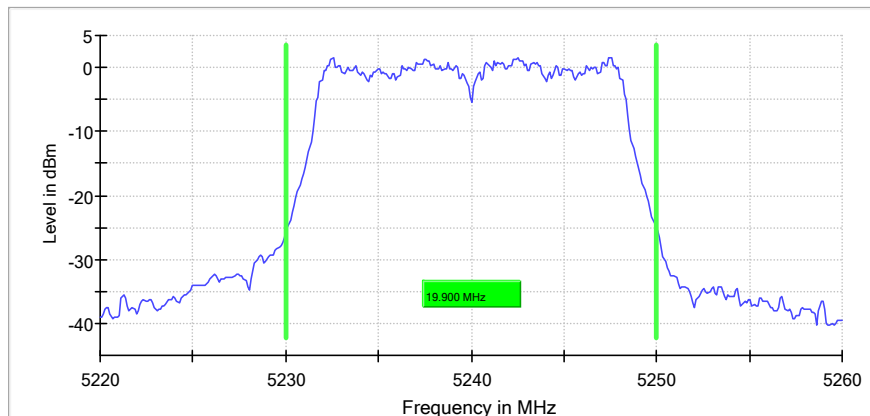
26 dB Bandwidth
