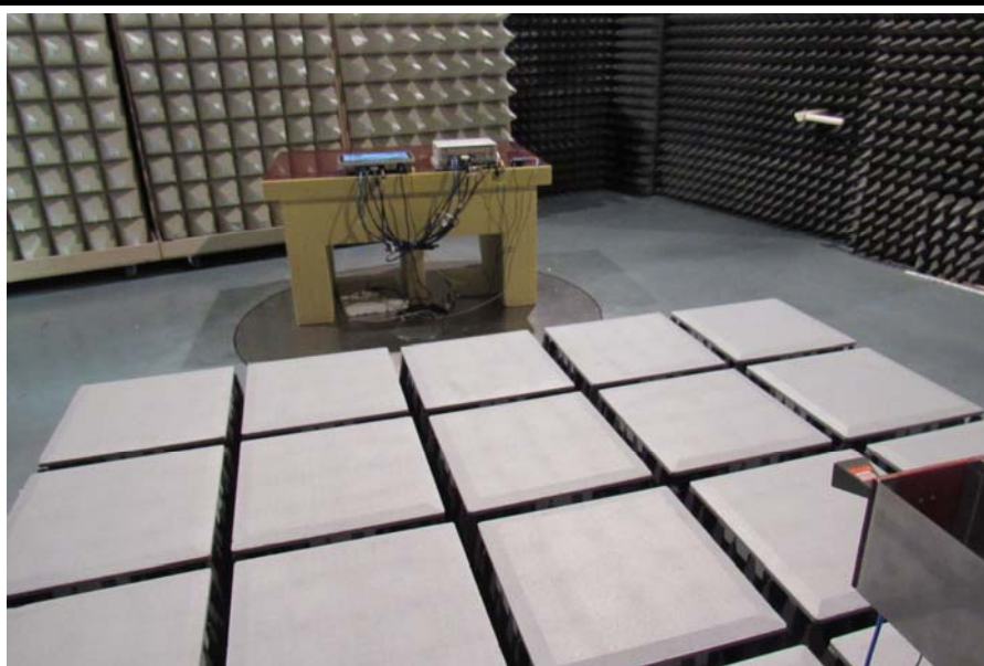
TEST SETUP 4 RADIATED EMISSION
