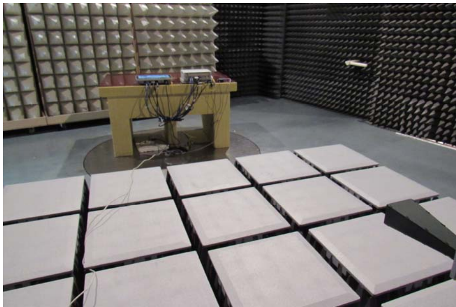
TEST SETUP 5 RADIATED EMISSION
