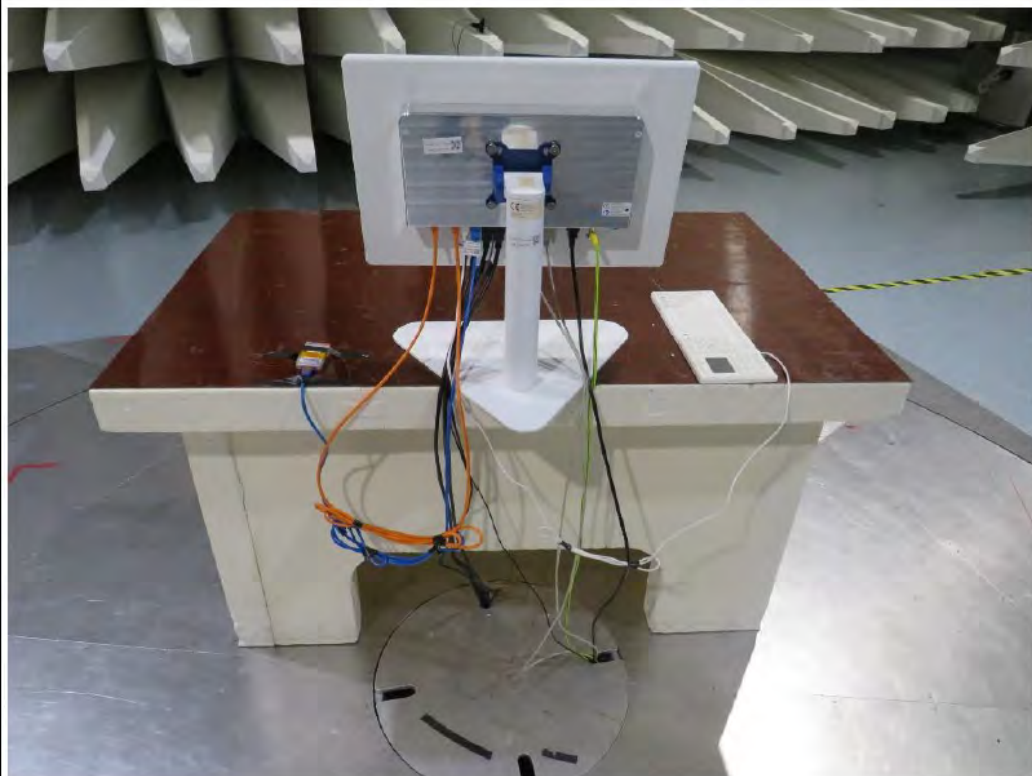
OR-PC® 24 Radiated Emission Test Setup 30 – 1000 MHz
