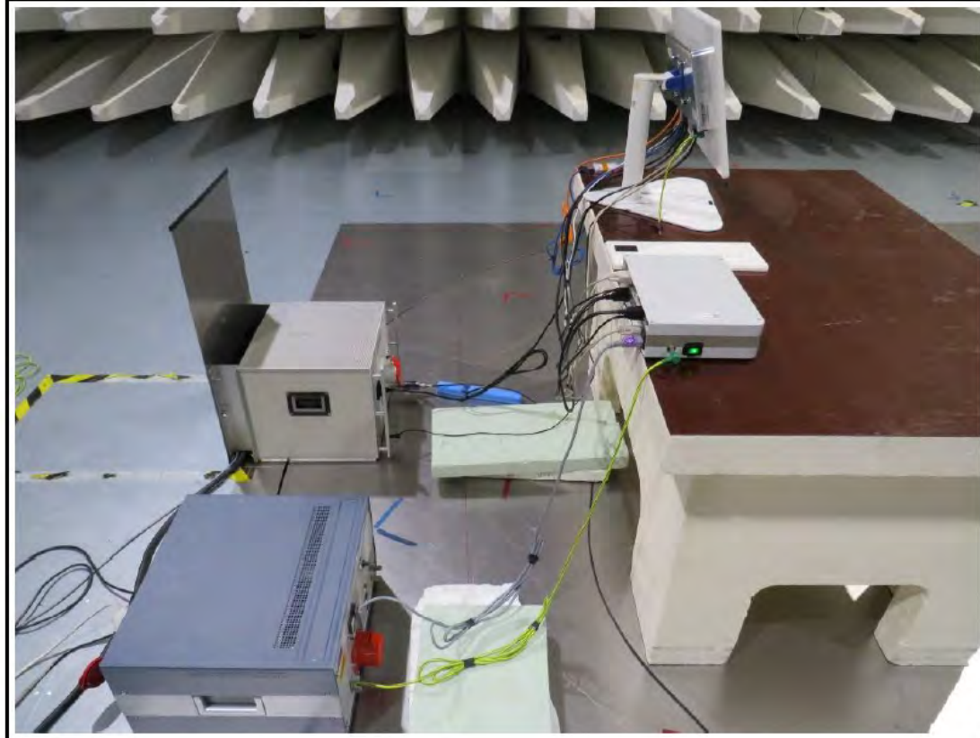
OR-PC® 24 Conducted Emission Test Setup
